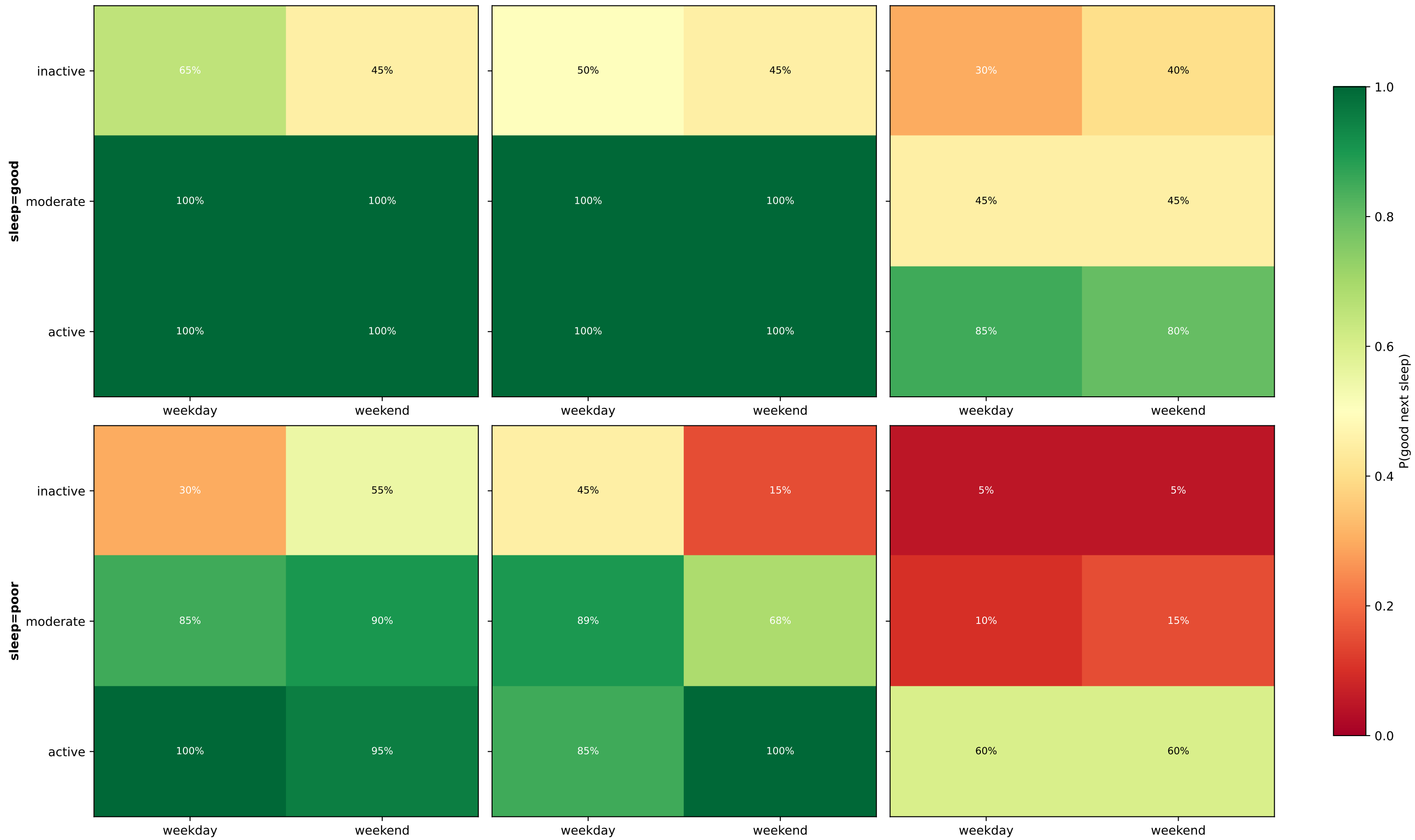
social_responder_deepseek-v4-flash — P(next sleep = good | step_bin_daily, burden, day_type, sleep) Rows: current sleep. Columns: burden level (low, medium, high). Realistic: poor sleep or higher burden reduces P(good).
