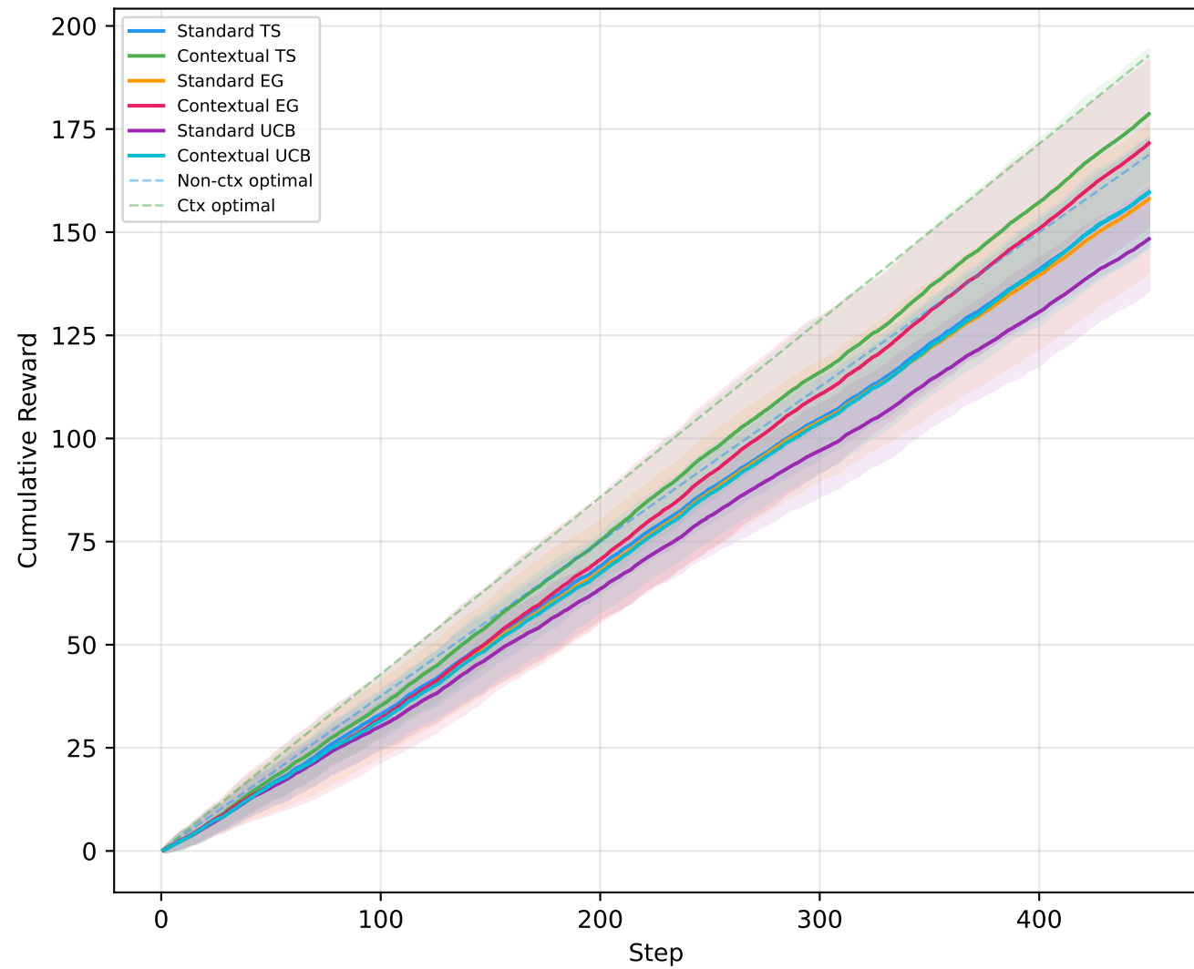
Cumulative Reward
