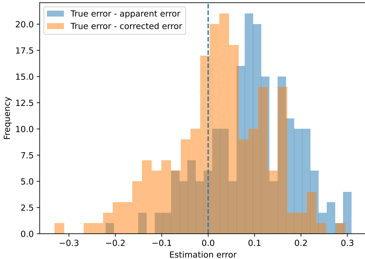
Effect of Efron's optimism correction
