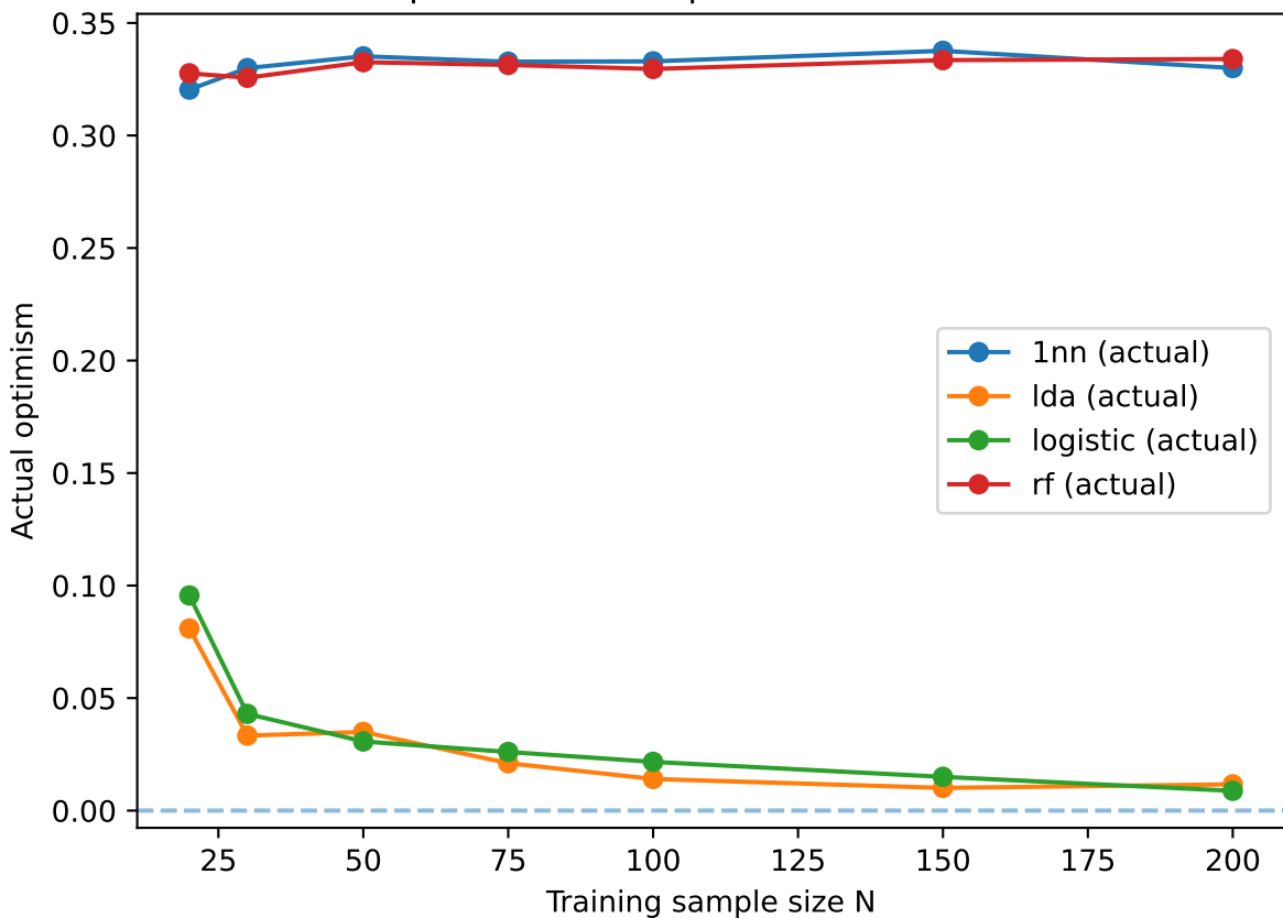
Actual optimism vs sample size for DGP: nonlinear
