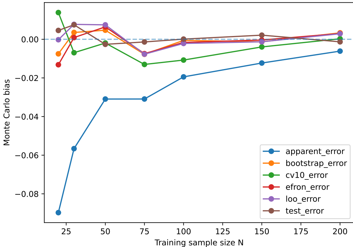
Bias of prediction-error estimators for logistic model, DGP: efron
