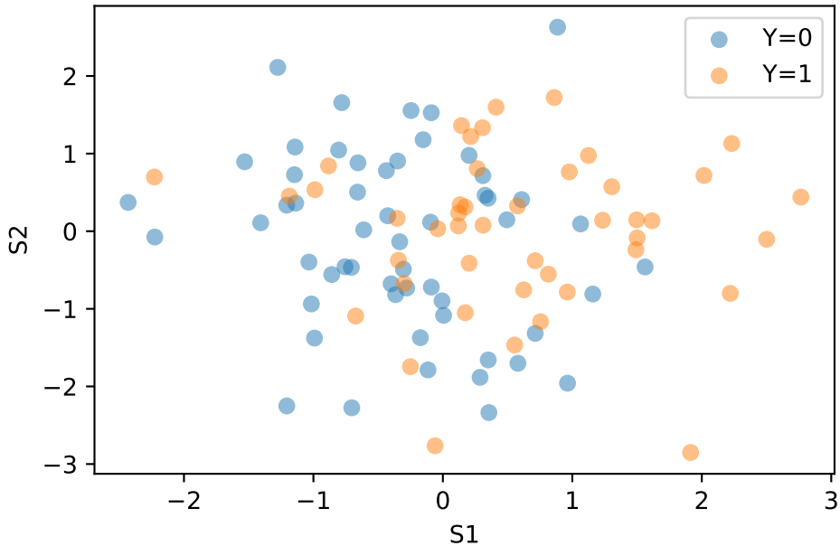
Simulated Data
