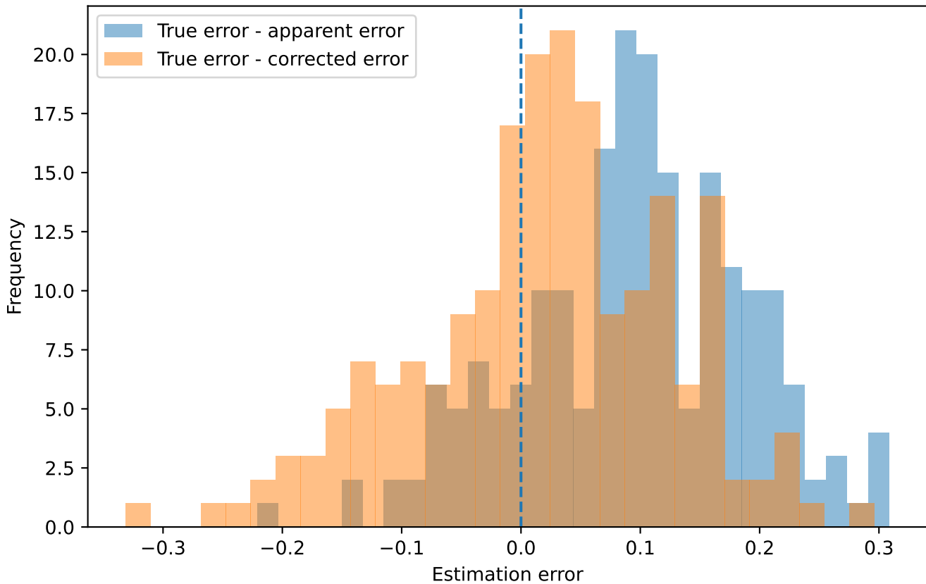
Effect of Efron's optimism correction
