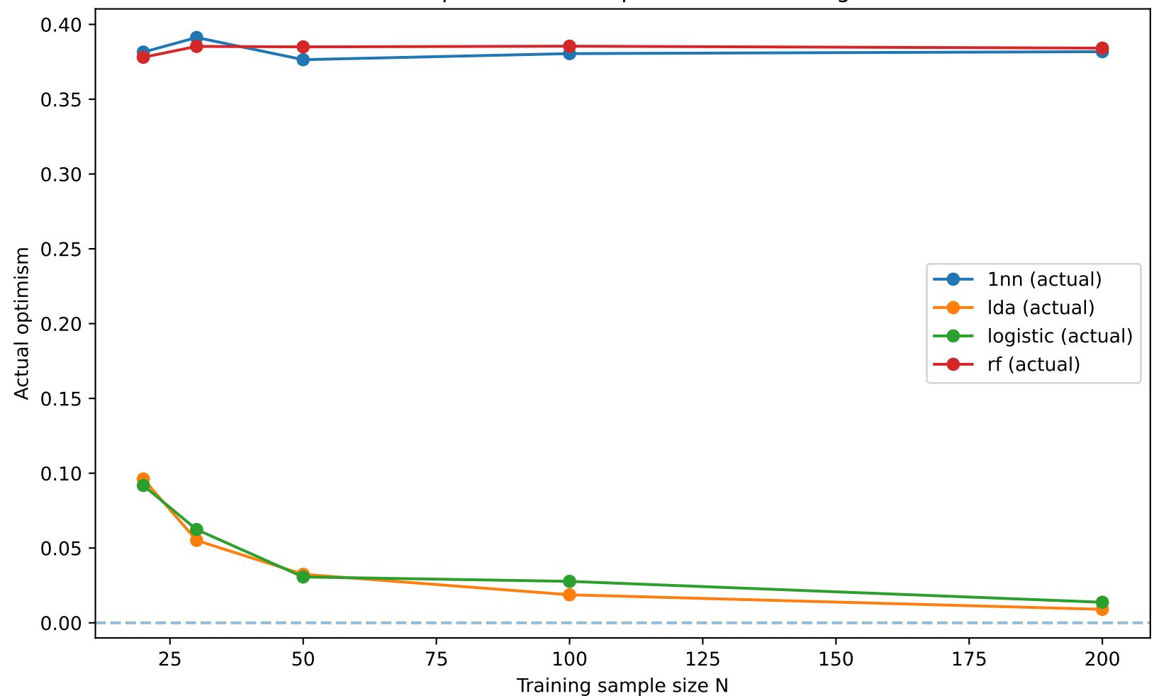
Actual optimism vs sample size for DGP: logistic
