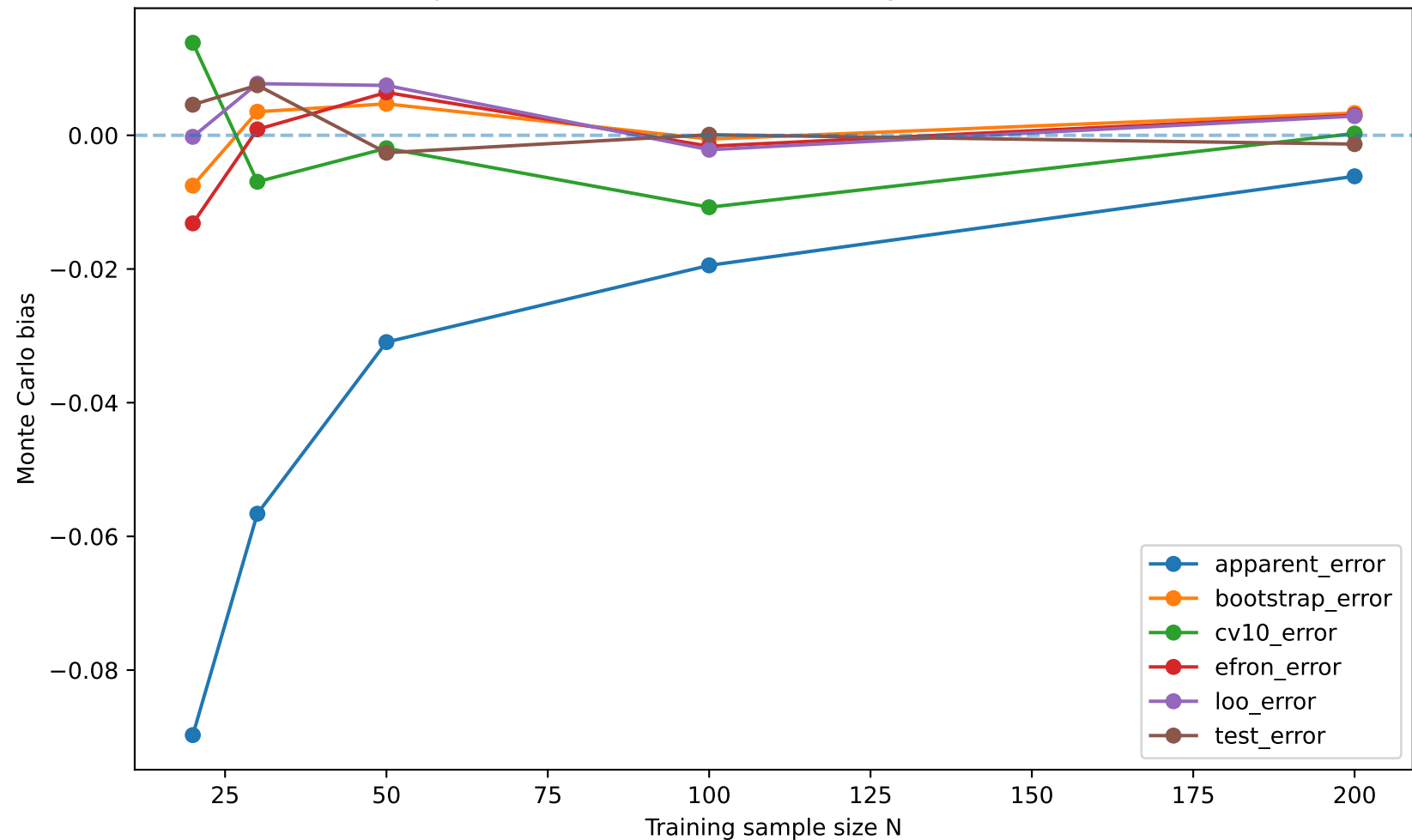
Bias of prediction-error estimators for logistic model, DGP: efron
