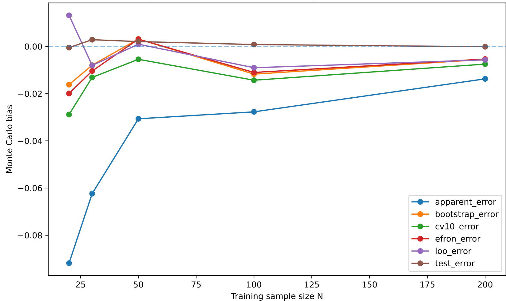
Bias of prediction-error estimators for logistic model, DGP: logistic
