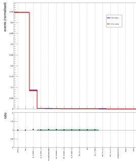
8 TeV cutflow versus 13 TeV cutflow for selection ee
