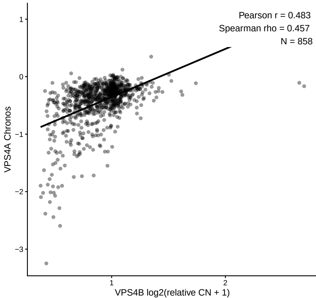
VPS4B CN vs VPS4A Dependency
