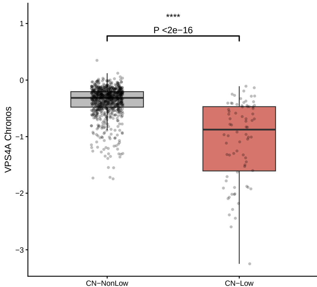
VPS4A Dependency by VPS4B CN Status
