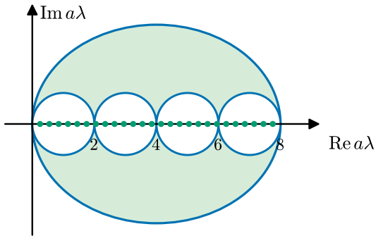
spectrum of D_{\text{Wilson}} (m=0) : cusps related to doubler modes
