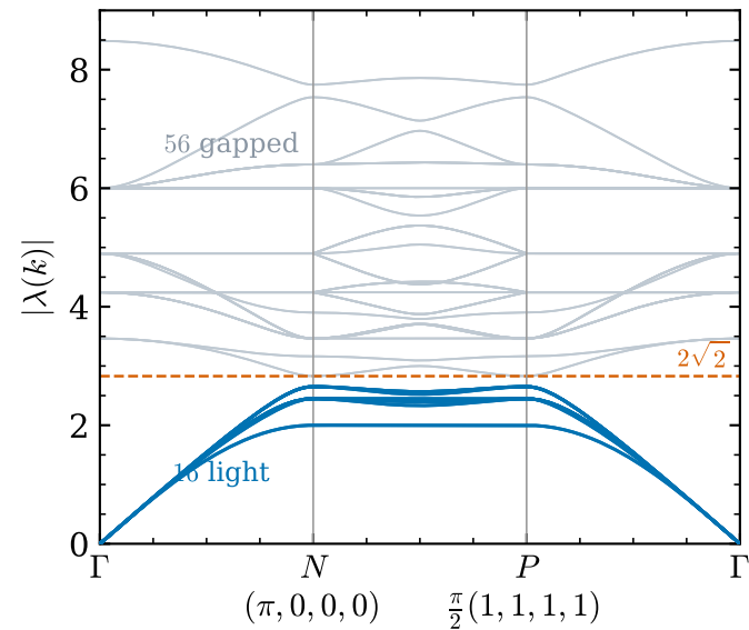
(a) D_4 : 72 branches of d - \delta
