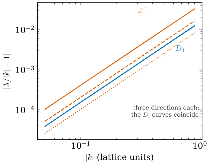
(b) discretisation error of the light modes
