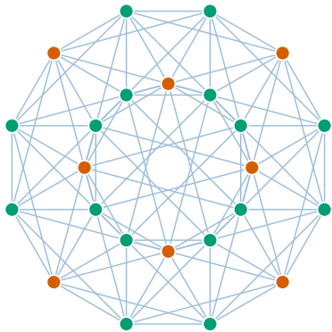
(b) D_4^* : (\pm 1, 0, 0, 0) \oplus (\pm \frac{1}{2}, \dots)
