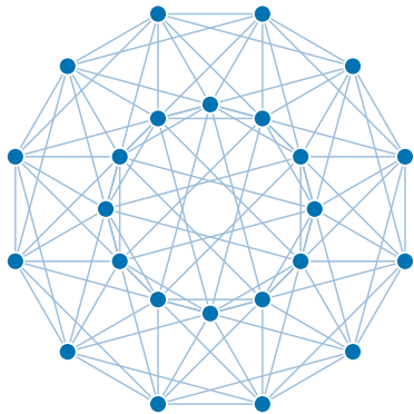
(a) D_4 : (\pm 1, \pm 1, 0, 0)
