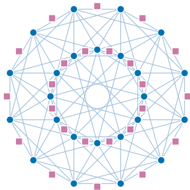
(c) shell 1 and shell 2 of D_4
