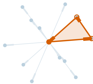
(b) the minimal loop is a triangle
