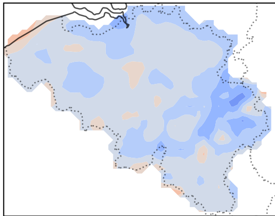
ALARO-12km average value = -0.25\text{ }^{\circ}\text{C}
