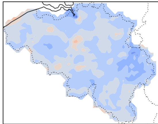
ALARO-4km average value = -0.32\text{ }^{\circ}\text{C}
