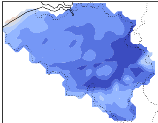
ALARO-25km average value = -1.14\text{ }^{\circ}\text{C}
