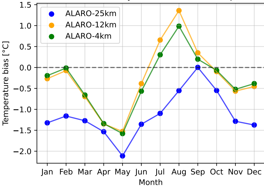
Bias in mean monthly near-surface air temperature
