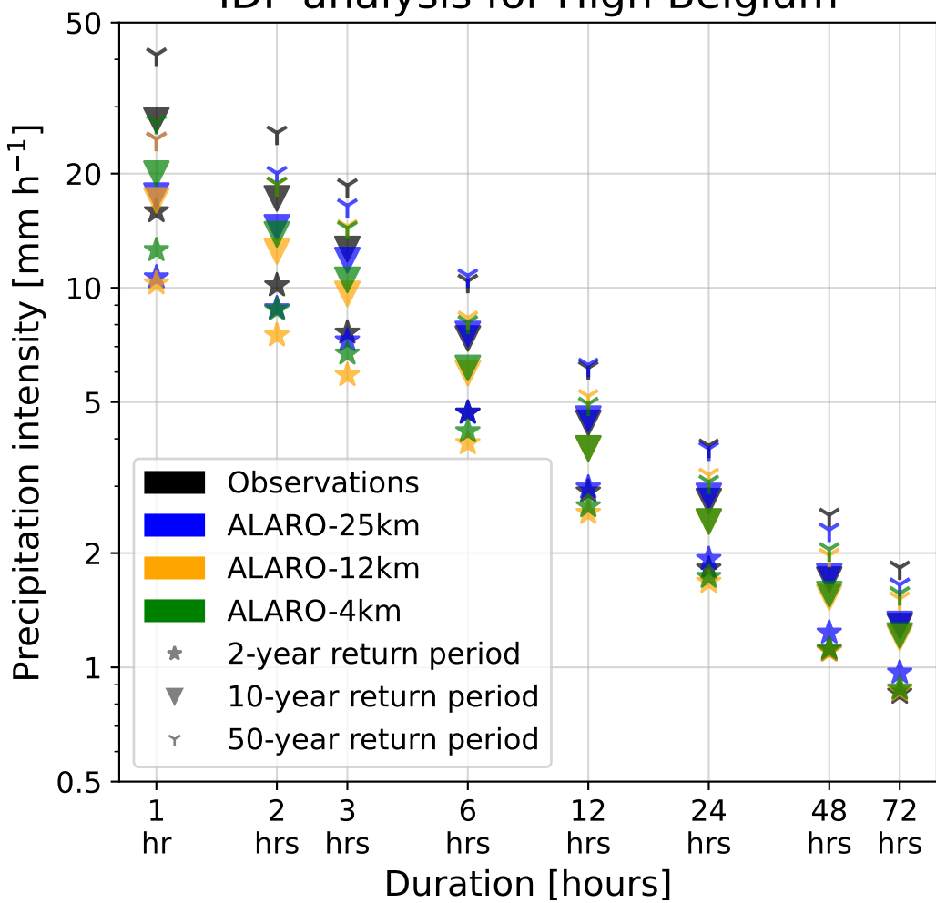
IDF-analysis for High-Belgium
