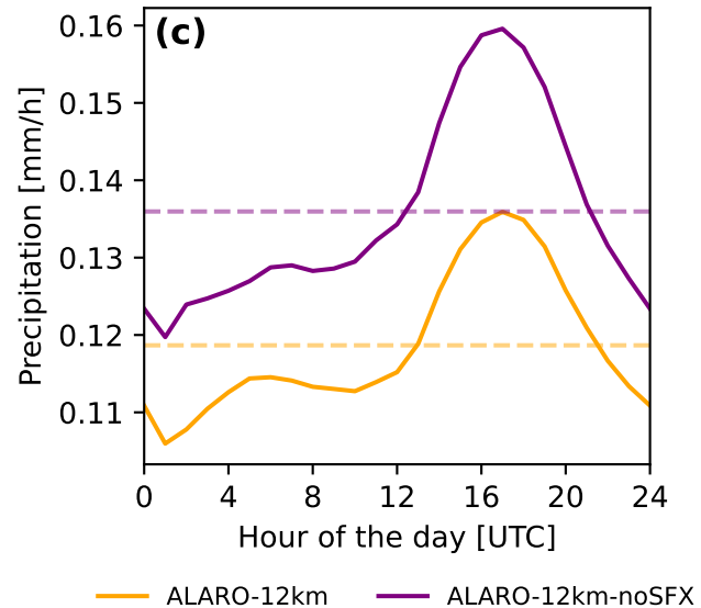
Diurnal cycle over Belgium
