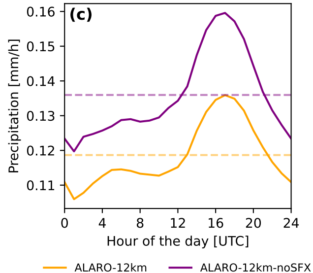
Diurnal cycle over Belgium
