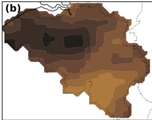
Precipitation average value = -12.6 %
