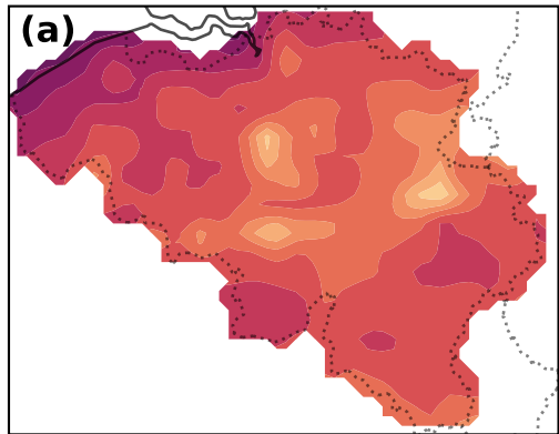
Near-Surface Air Temperature average value = 0.82 °C
