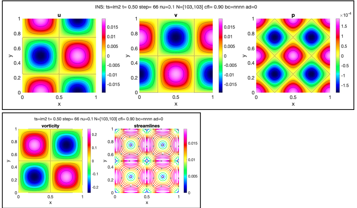
Figure 1: Taylor Green vortex
