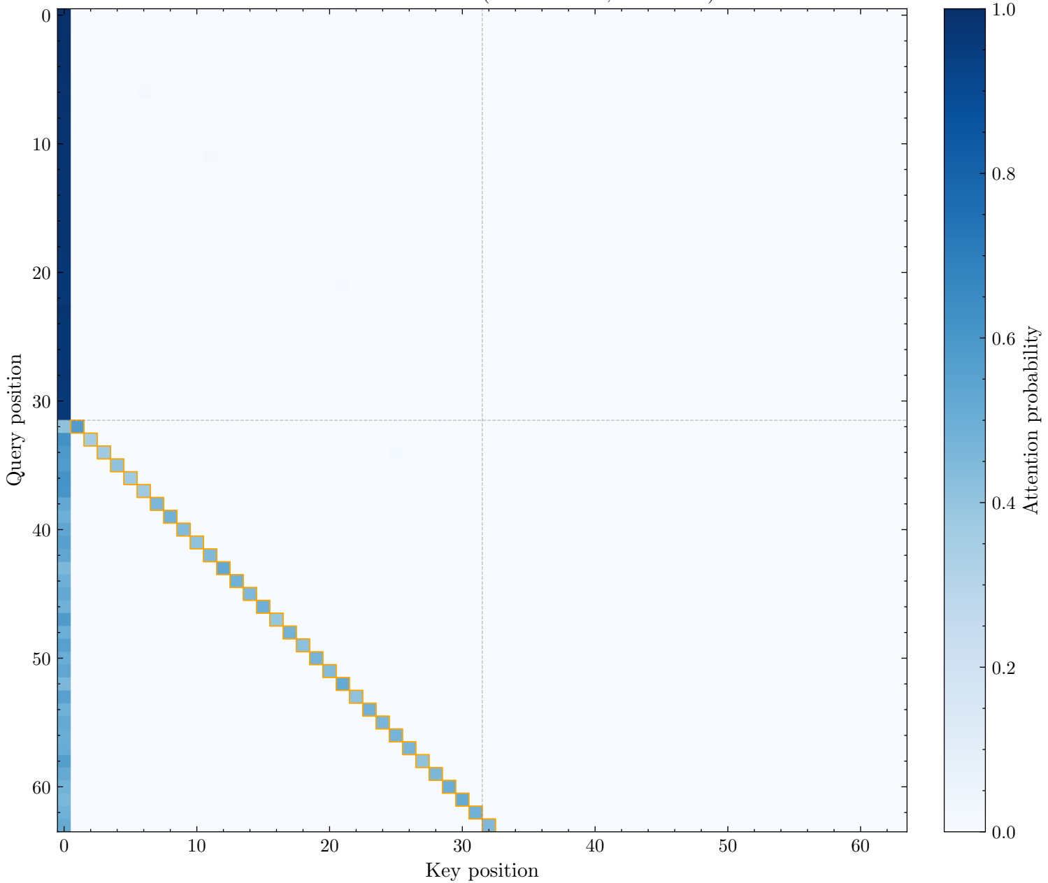
Induction Head: L2H20 (Score: 0.468, Rank: 13)
