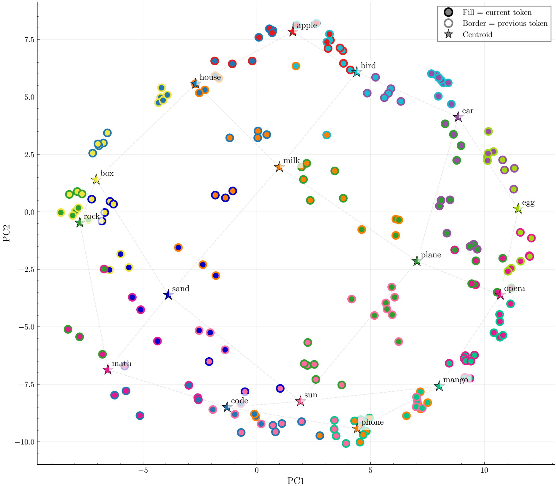
Layer 26 Activations (Bigram View)
