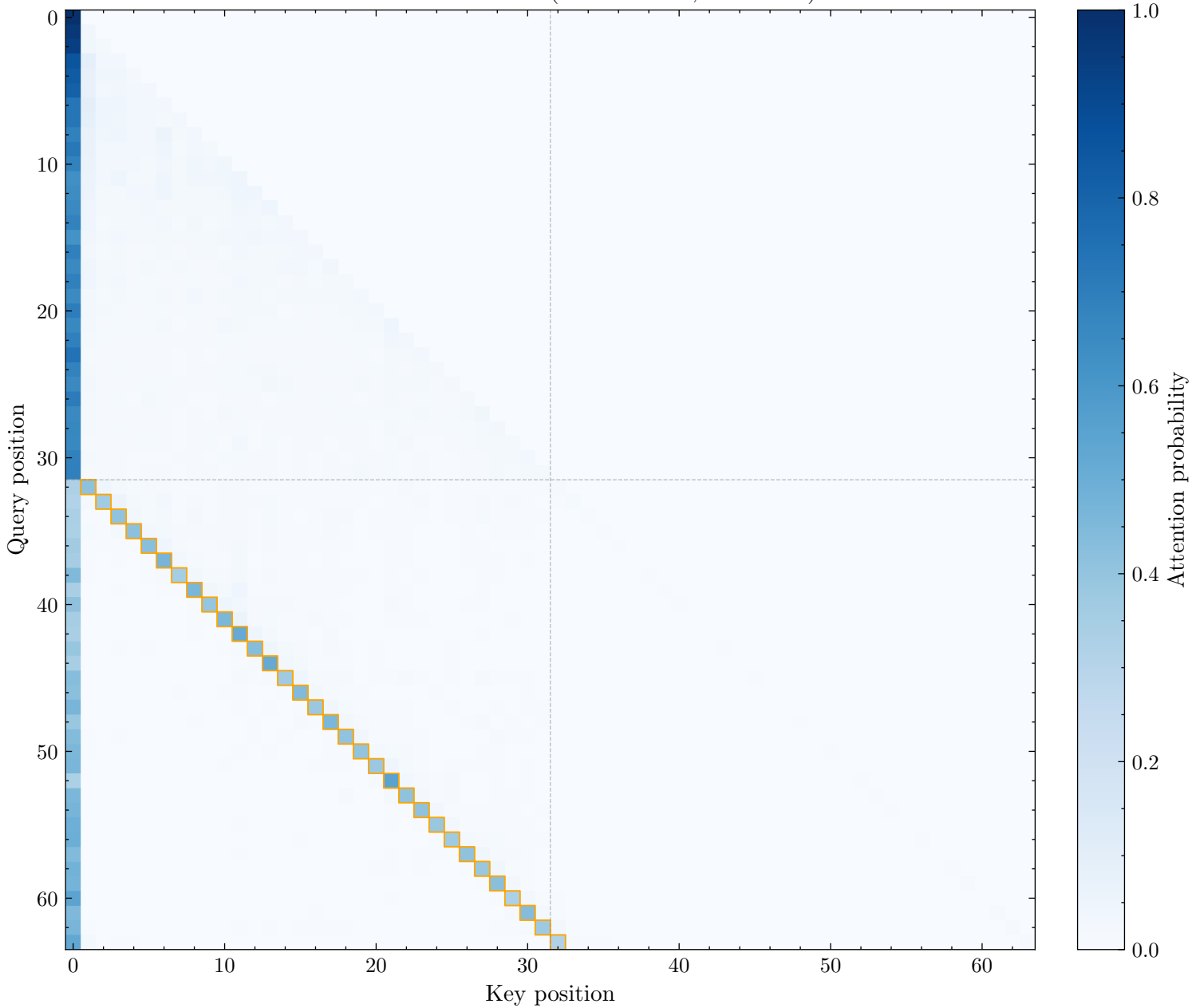
Induction Head: L27H6 (Score: 0.423, Rank: 16)
