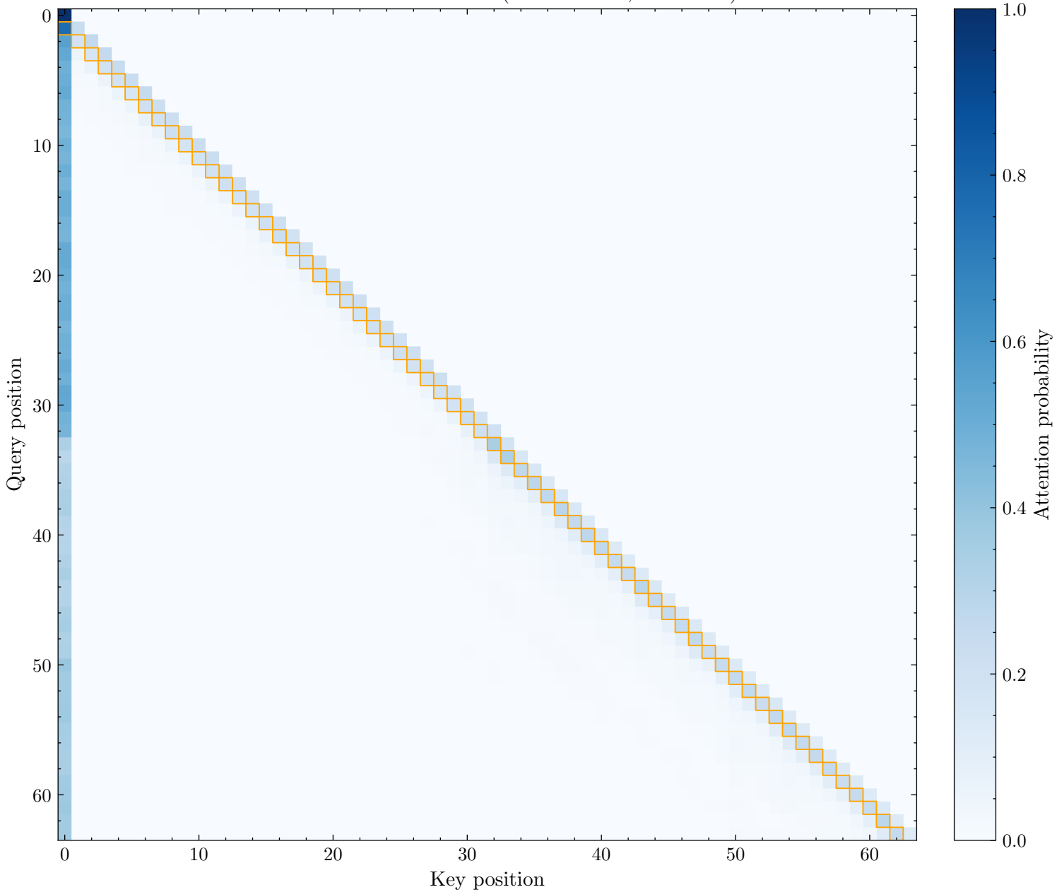
Prev Token Head: L16H29 (Score: 0.237, Rank: 26)
