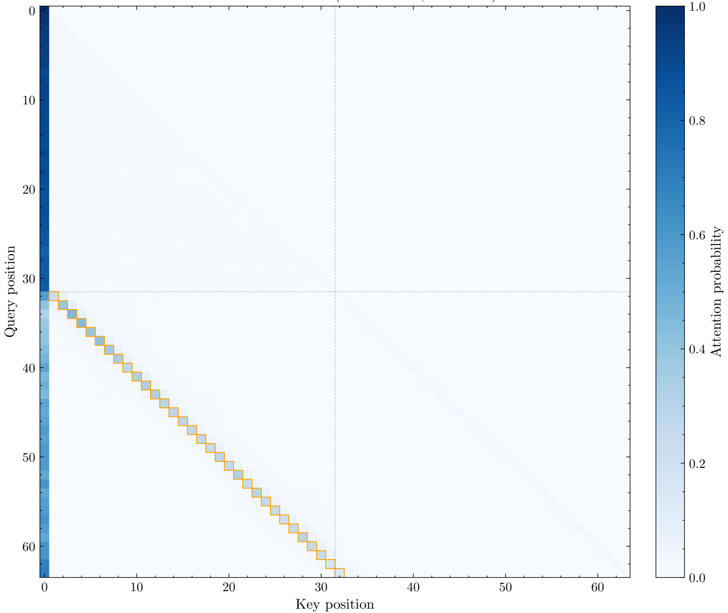
Induction Head: L16H1 (Score: 0.307, Rank: 21)
