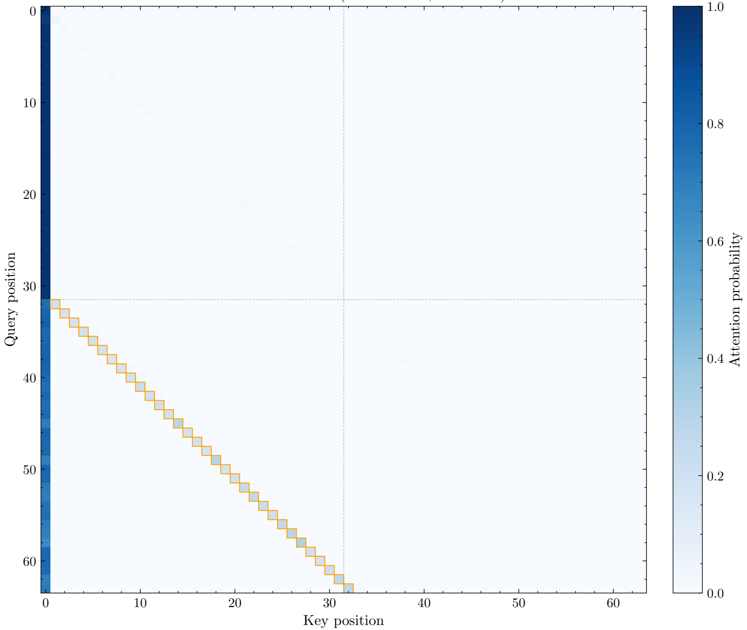
Induction Head: L5H9 (Score: 0.243, Rank: 28)
