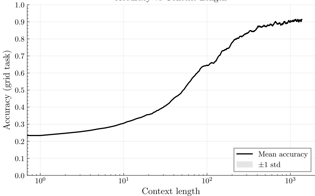
Accuracy vs Context Length
