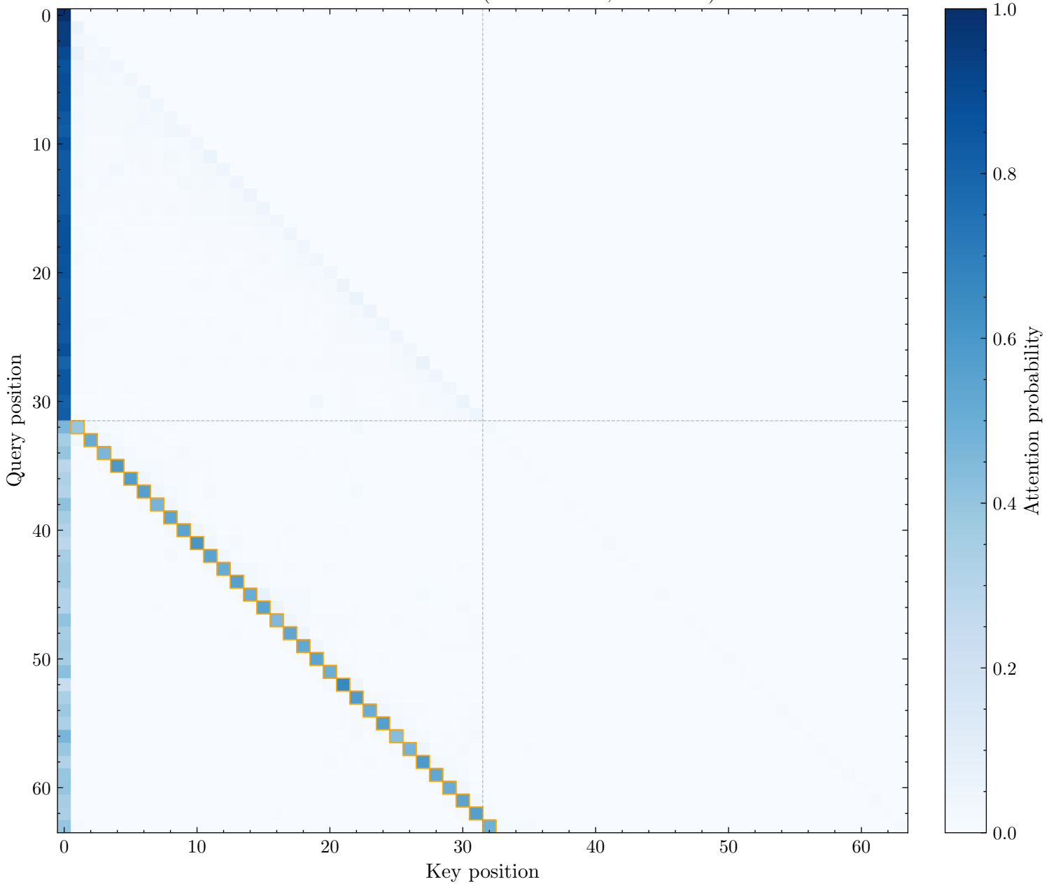
Induction Head: L20H1 (Score: 0.538, Rank: 11)
