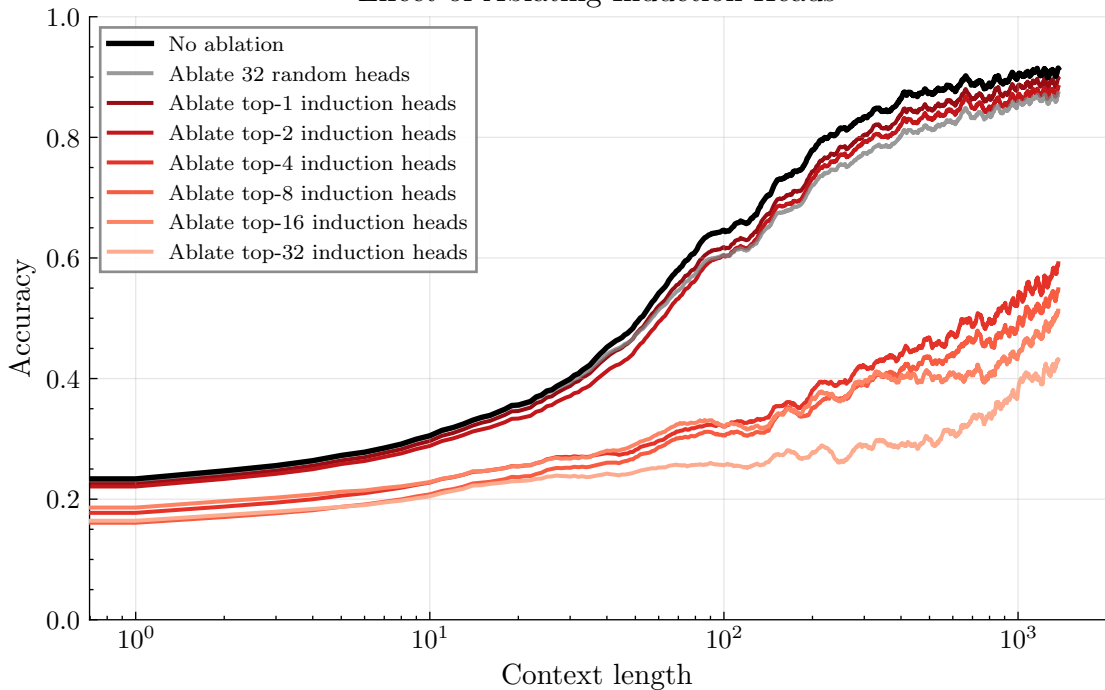
Effect of Ablating Induction Heads
