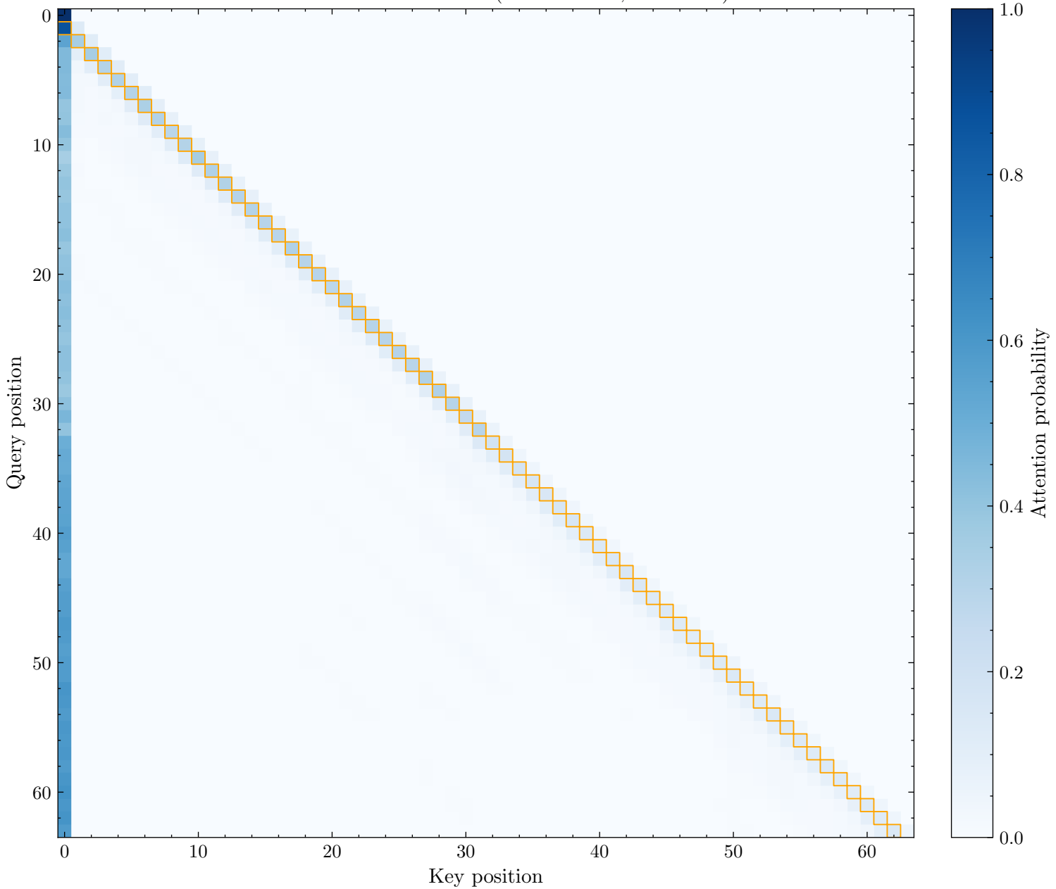
Prev Token Head: L14H9 (Score: 0.233, Rank: 29)
