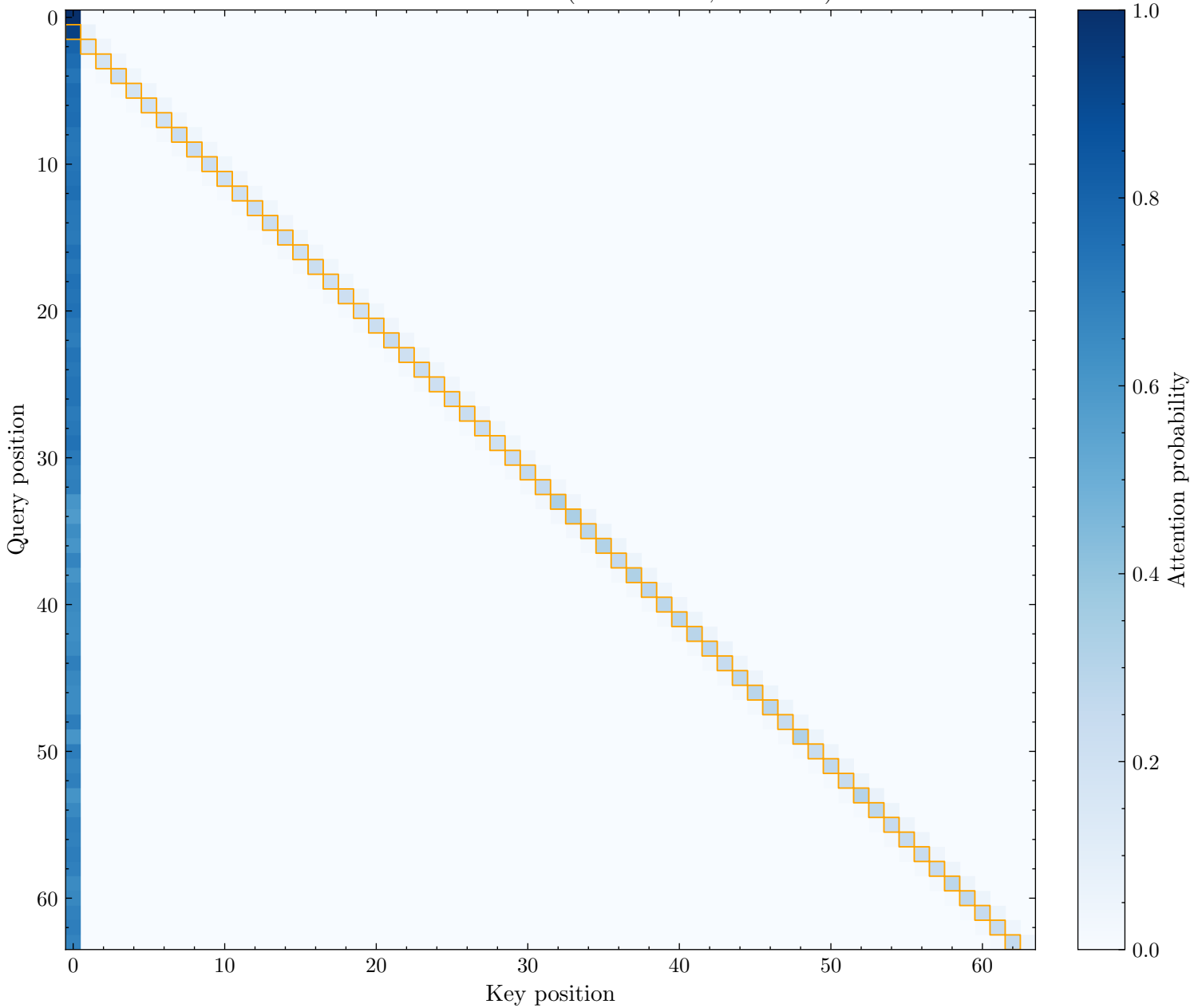
Prev Token Head: L25H20 (Score: 0.253, Rank: 24)
