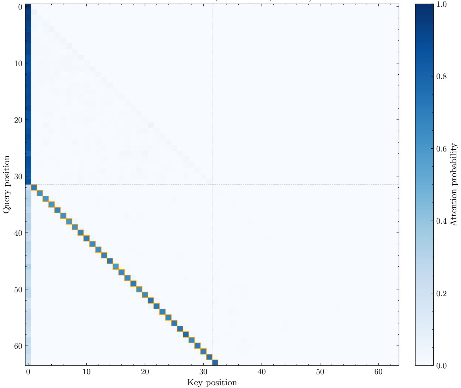
Induction Head: L5H11 (Score: 0.682, Rank: 6)
