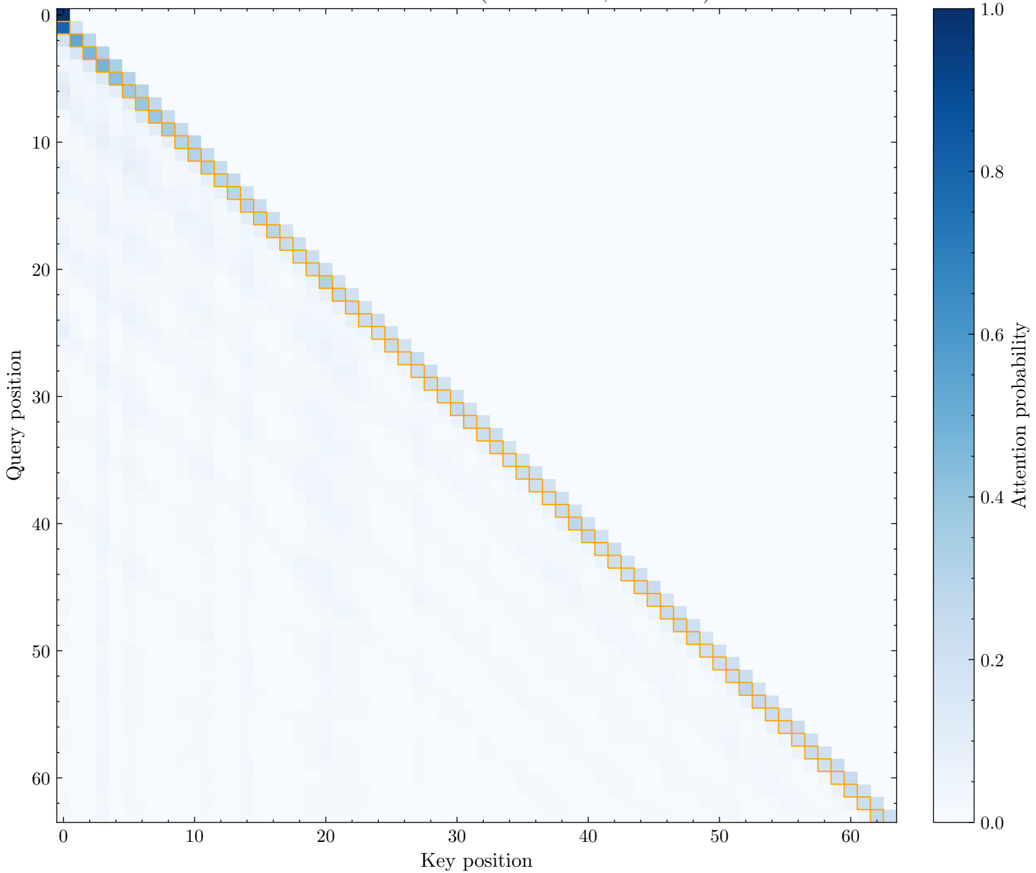
Prev Token Head: L1H4 (Score: 0.274, Rank: 18)
