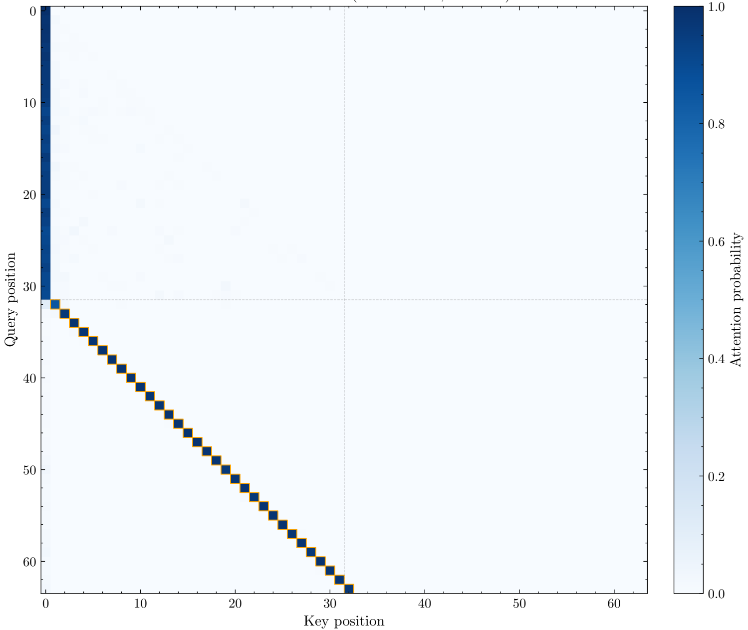
Induction Head: L15H30 (Score: 0.972, Rank: 1)
