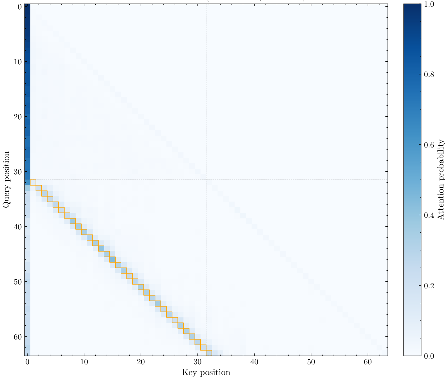
Induction Head: L13H6 (Score: 0.309, Rank: 20)
