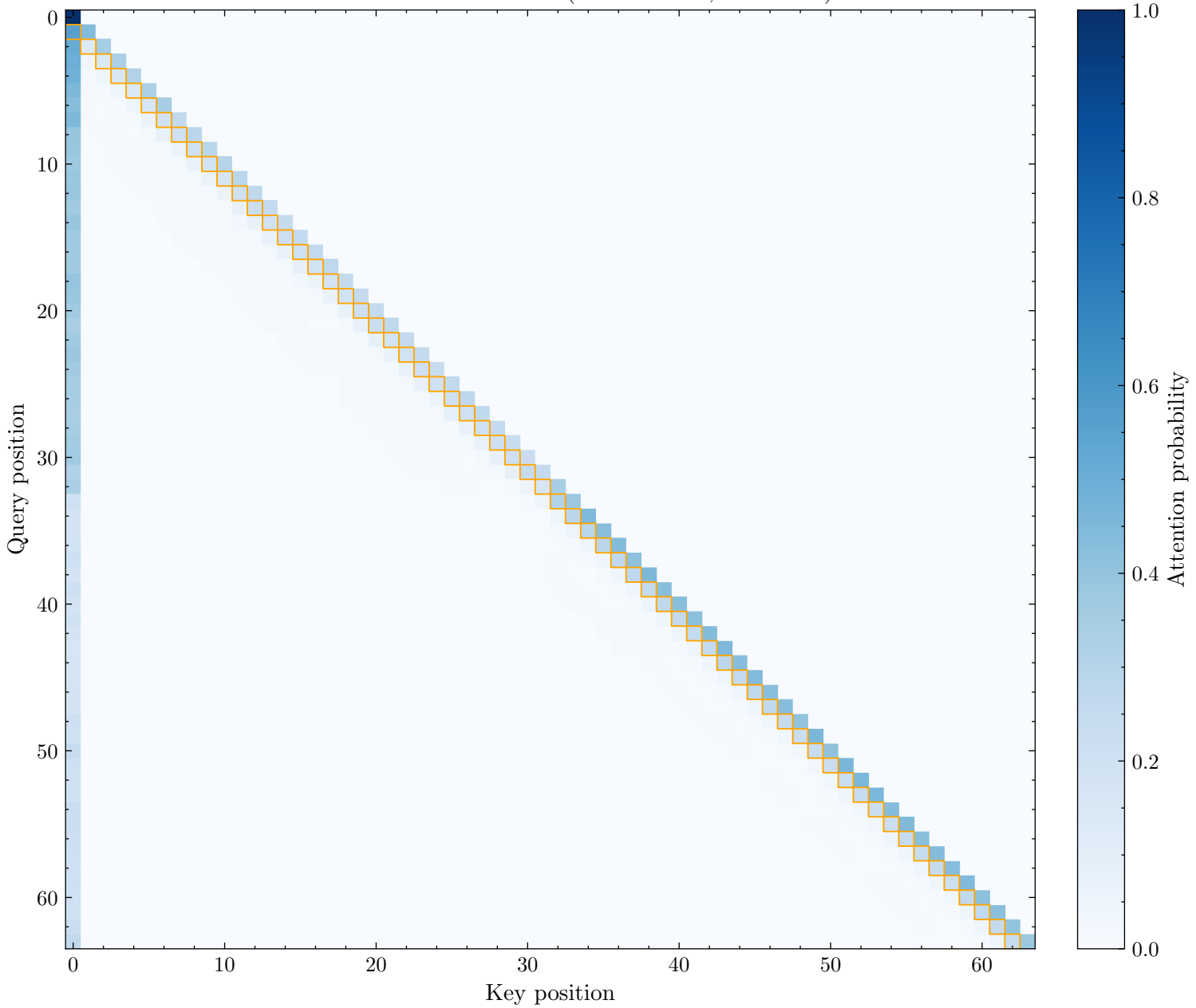
Prev Token Head: L21H10 (Score: 0.229, Rank: 31)
