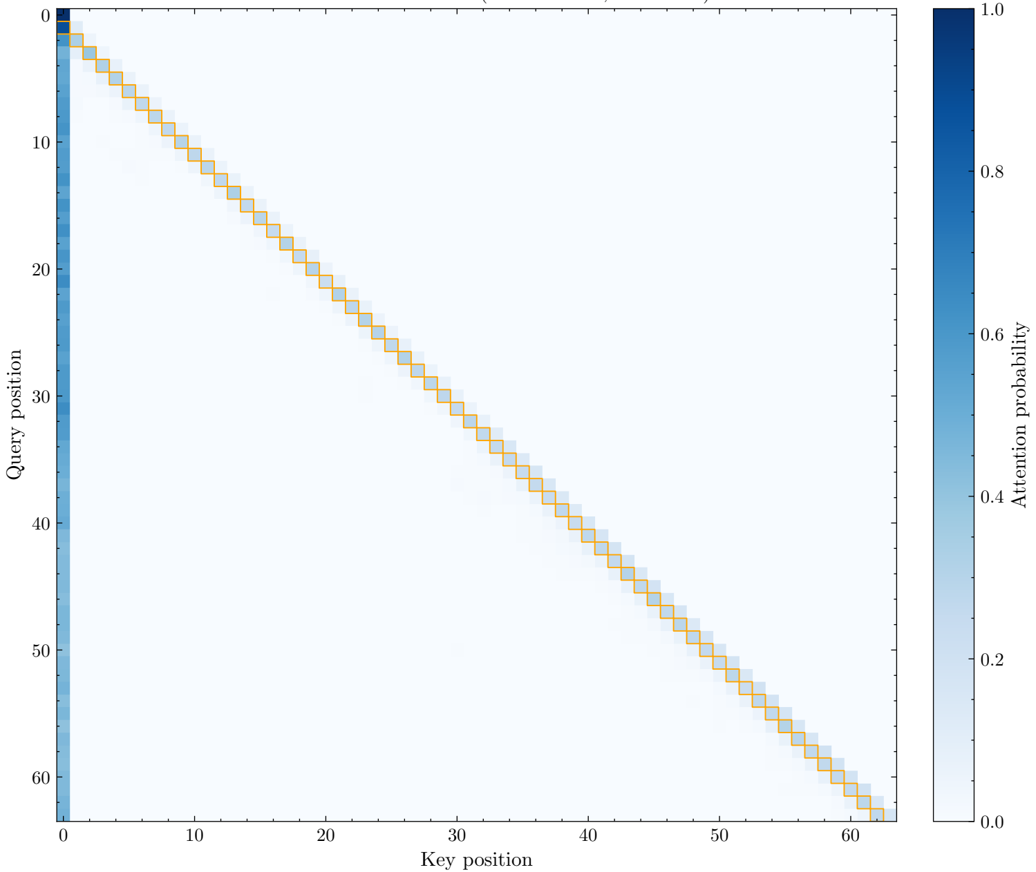
Prev Token Head: L7H1 (Score: 0.286, Rank: 15)
