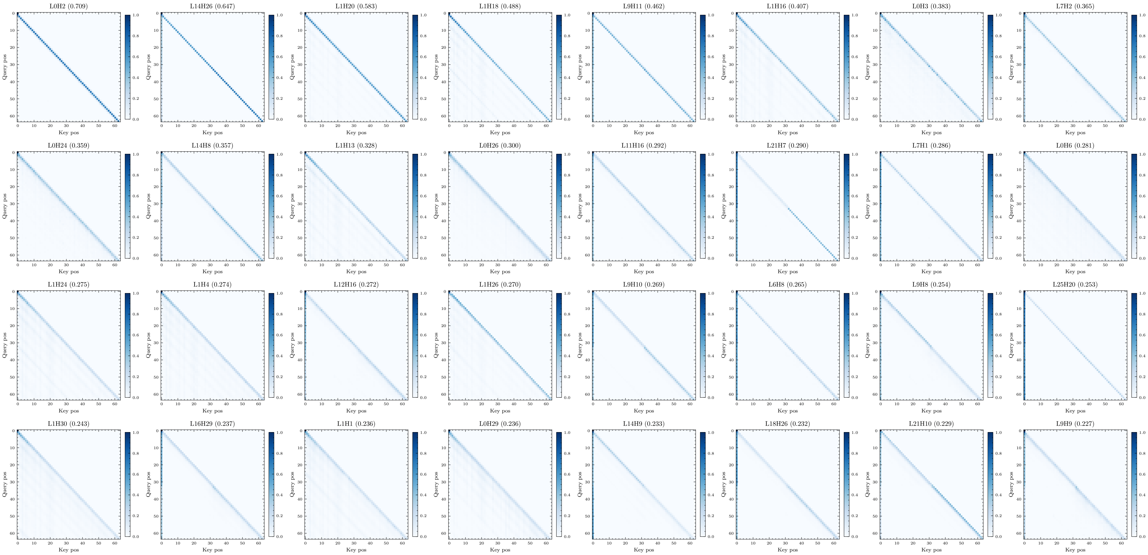
Top 32 Prev Token Heads
