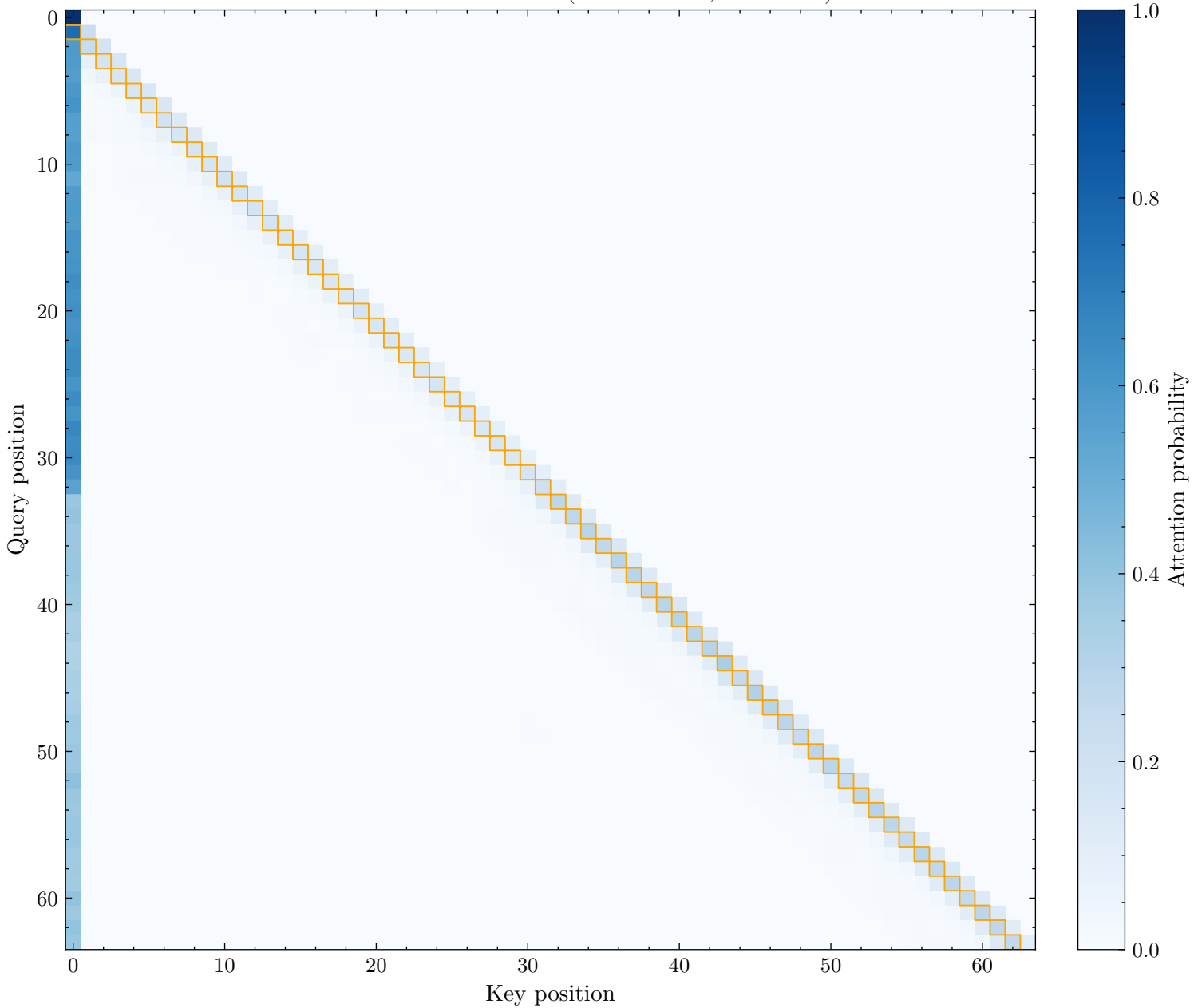
Prev Token Head: L18H26 (Score: 0.232, Rank: 30)
