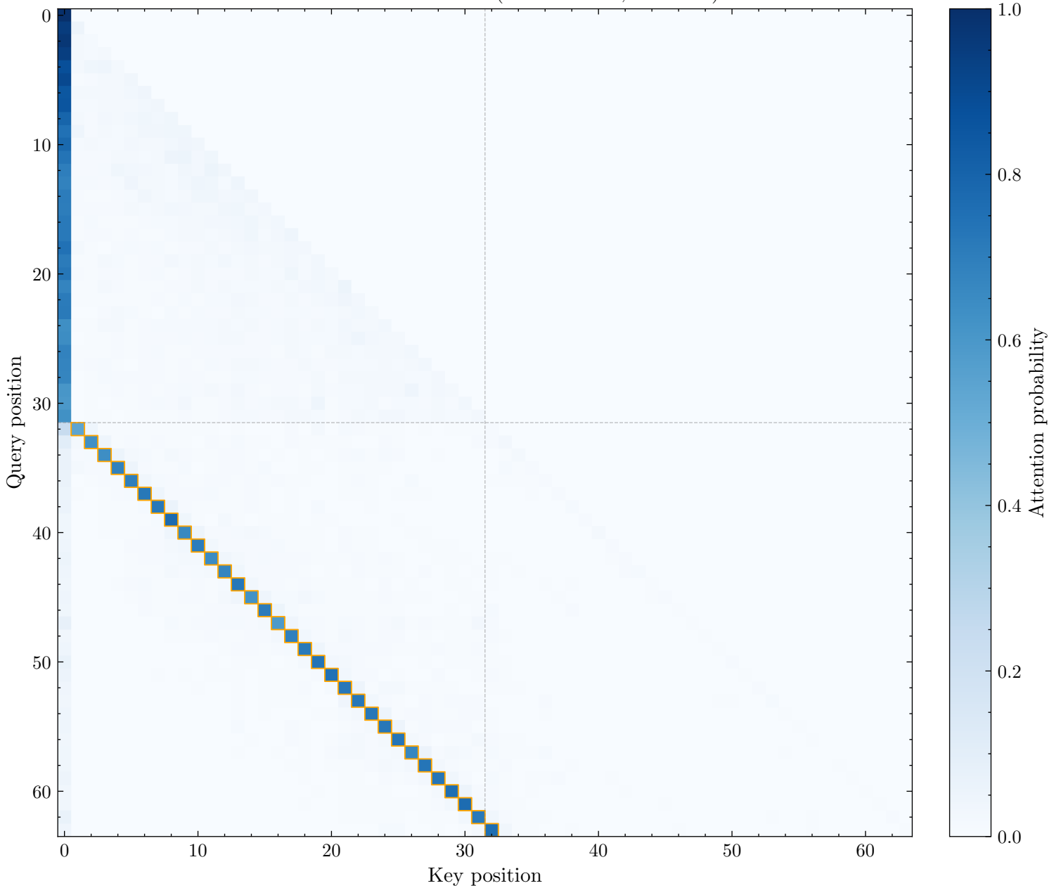
Induction Head: L10H14 (Score: 0.697, Rank: 5)
