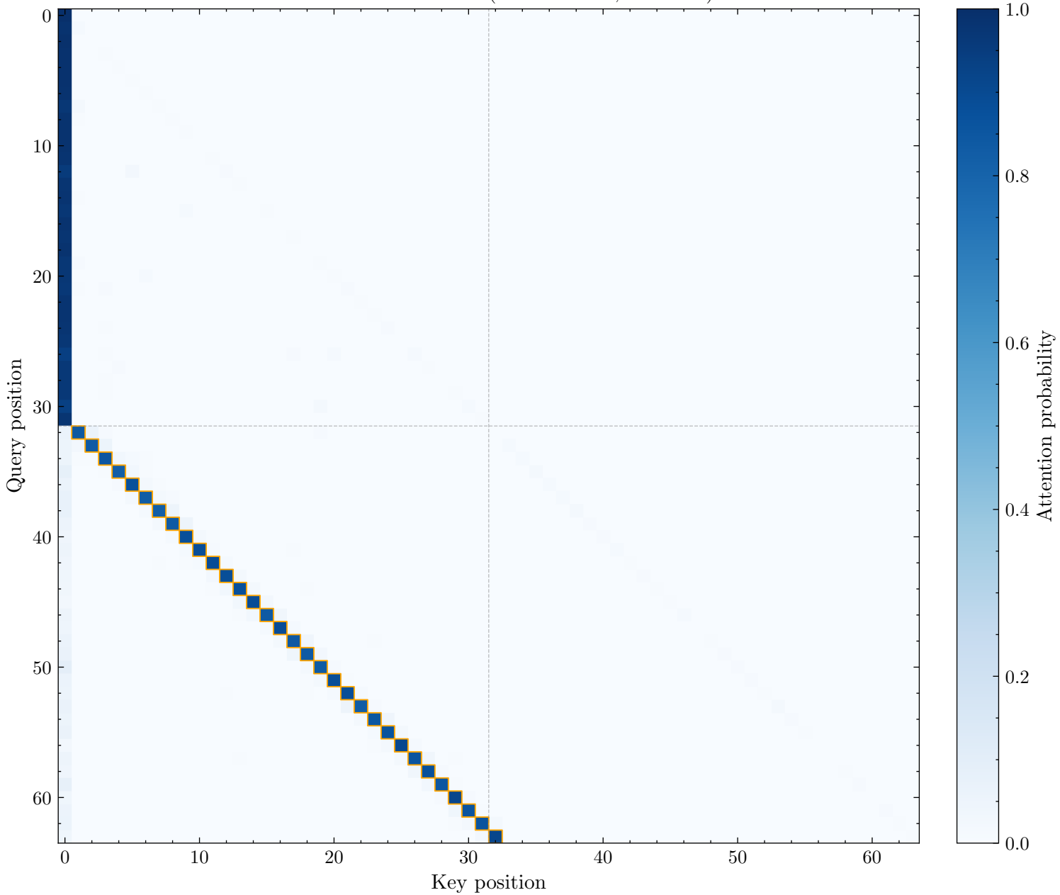
Induction Head: L8H1 (Score: 0.867, Rank: 2)
