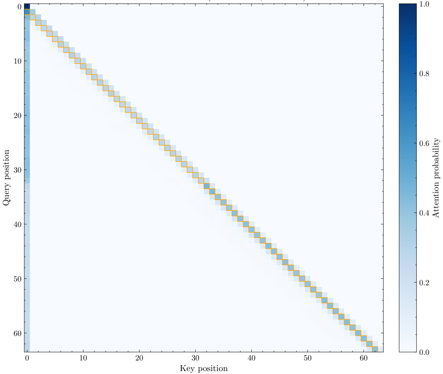
Prev Token Head: L14H8 (Score: 0.357, Rank: 10)
