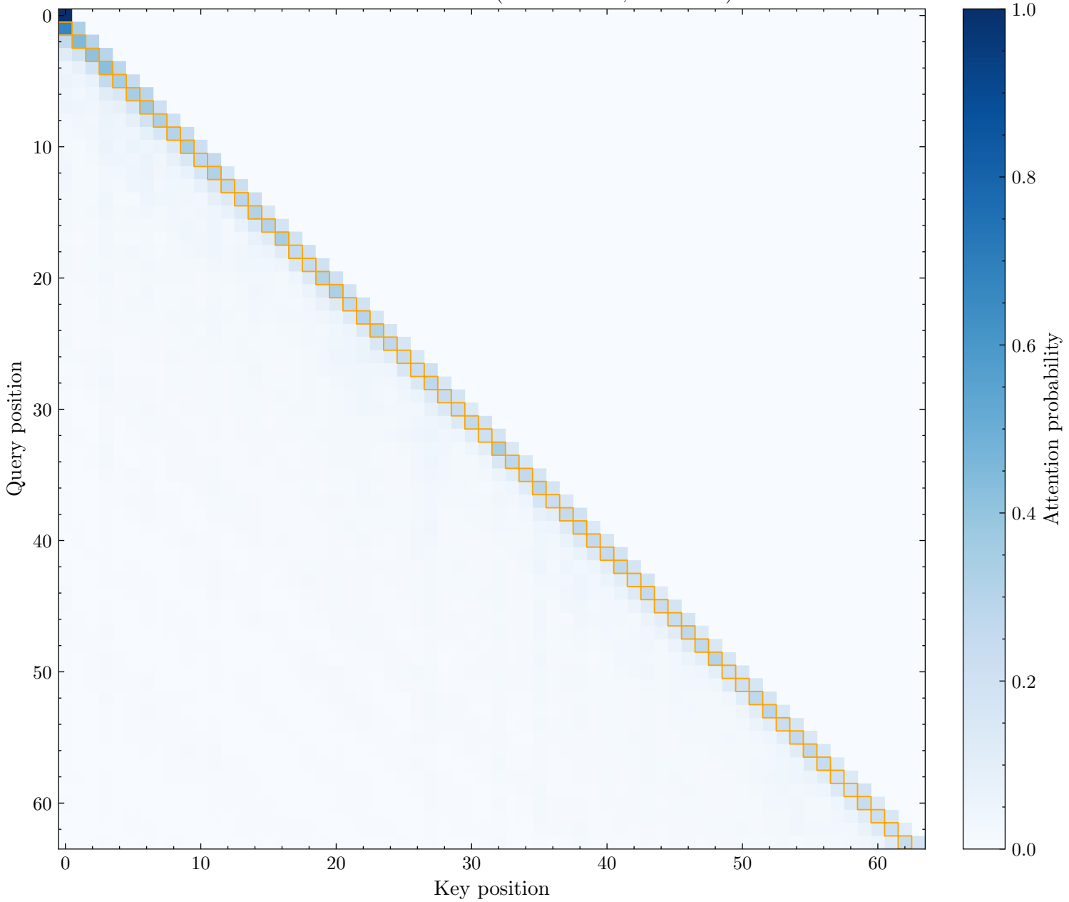
Prev Token Head: L0H6 (Score: 0.281, Rank: 16)
