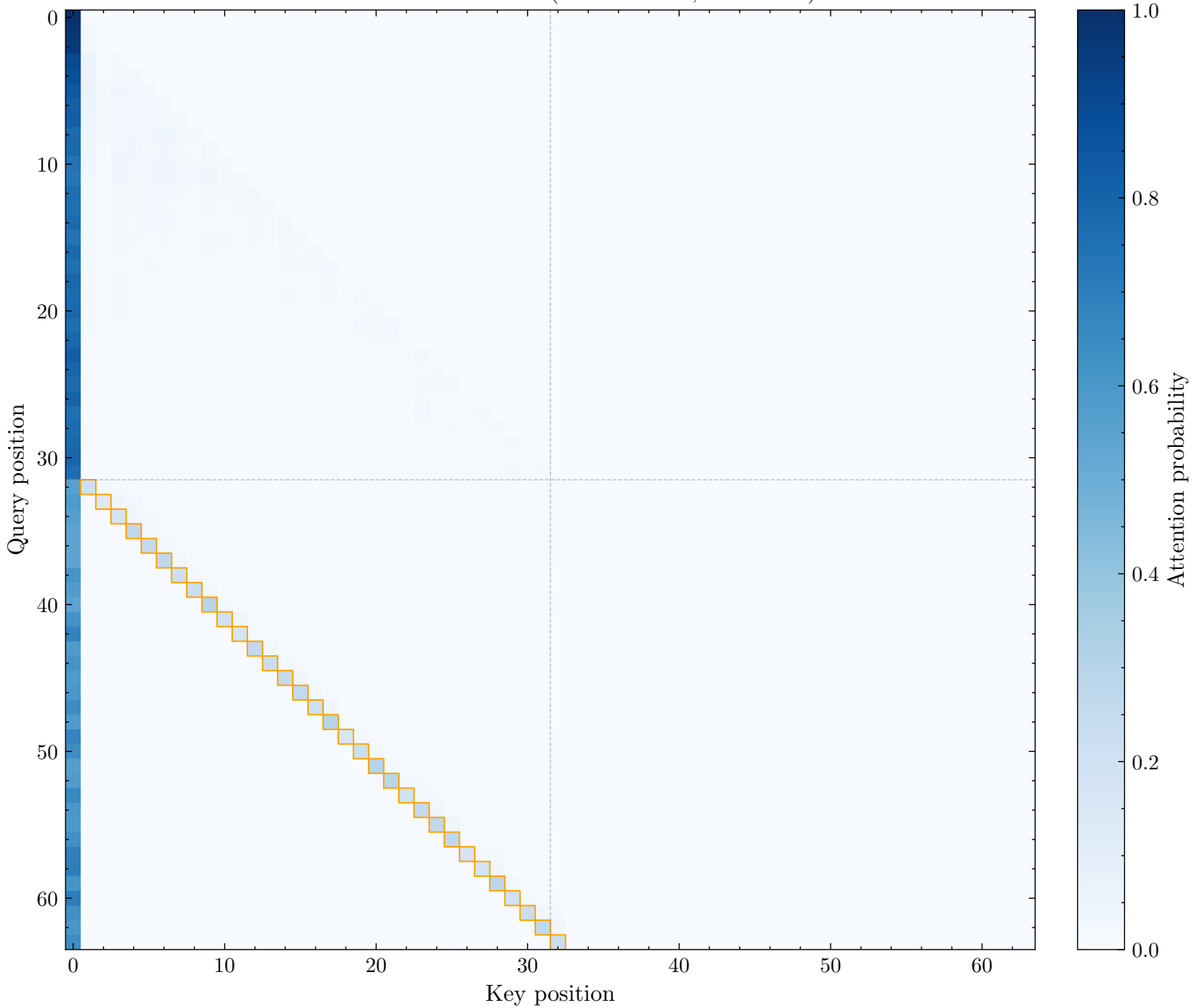
Induction Head: L27H4 (Score: 0.248, Rank: 25)
