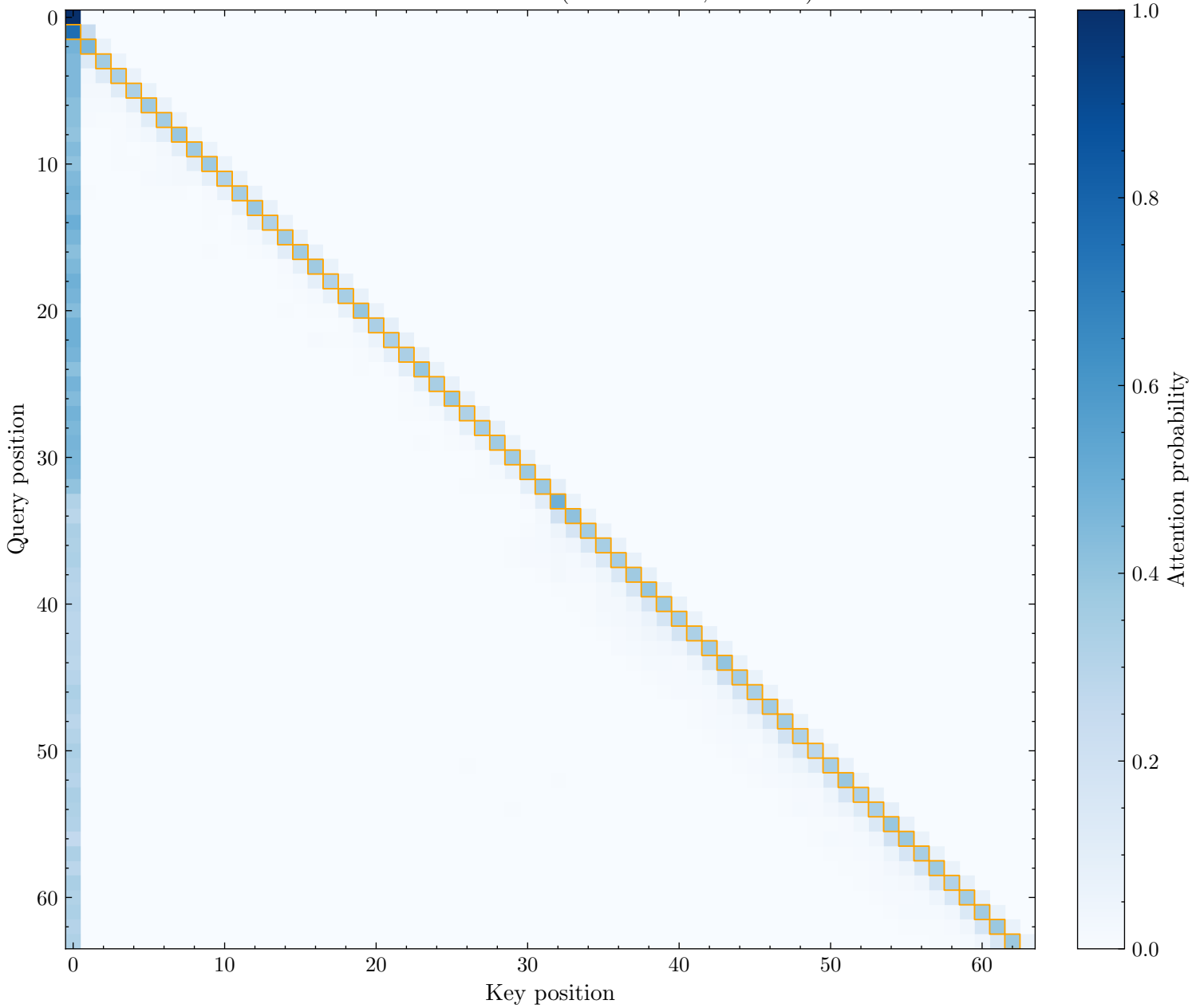
Prev Token Head: L7H2 (Score: 0.365, Rank: 8)
