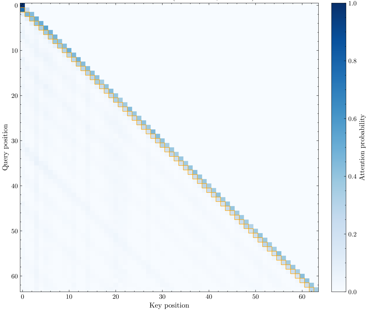
Prev Token Head: L1H26 (Score: 0.270, Rank: 20)
