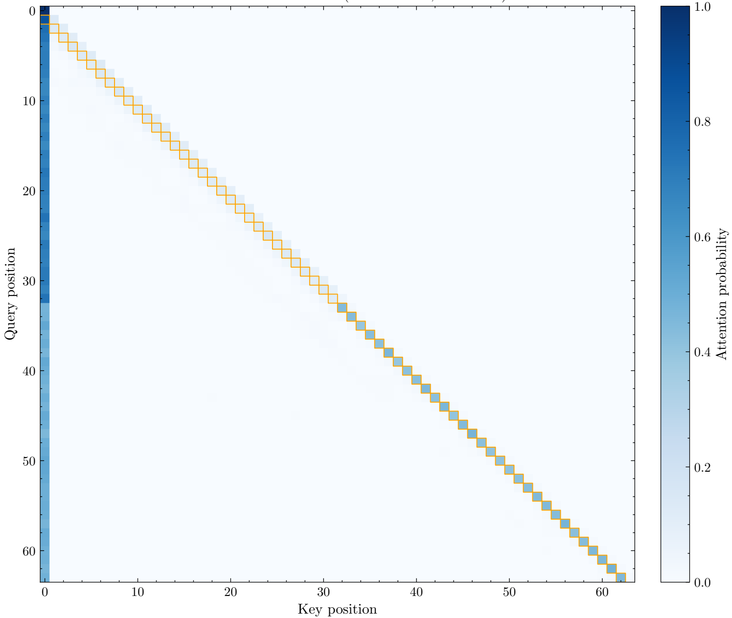
Prev Token Head: L21H7 (Score: 0.290, Rank: 14)
