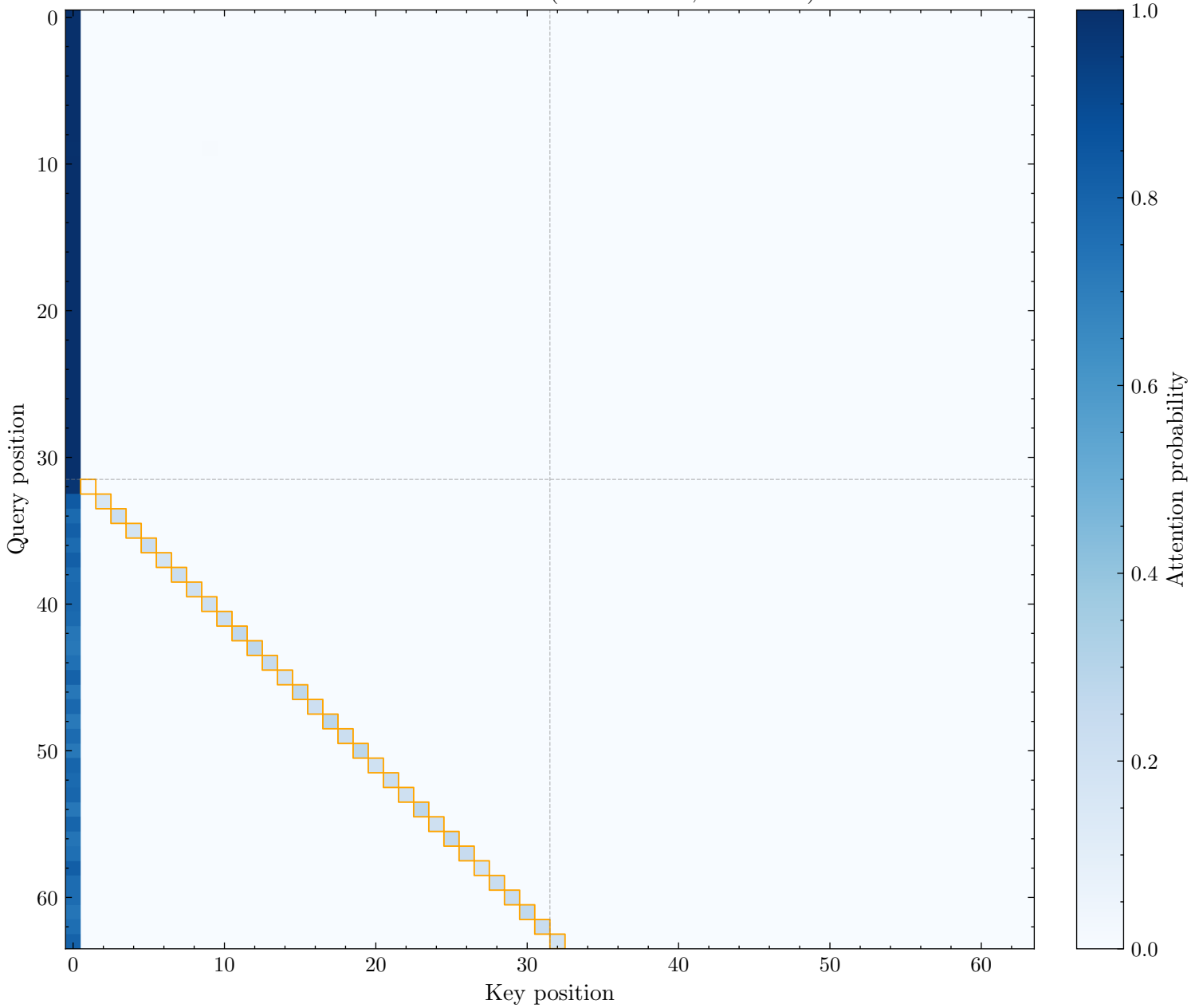
Induction Head: L2H21 (Score: 0.244, Rank: 26)
