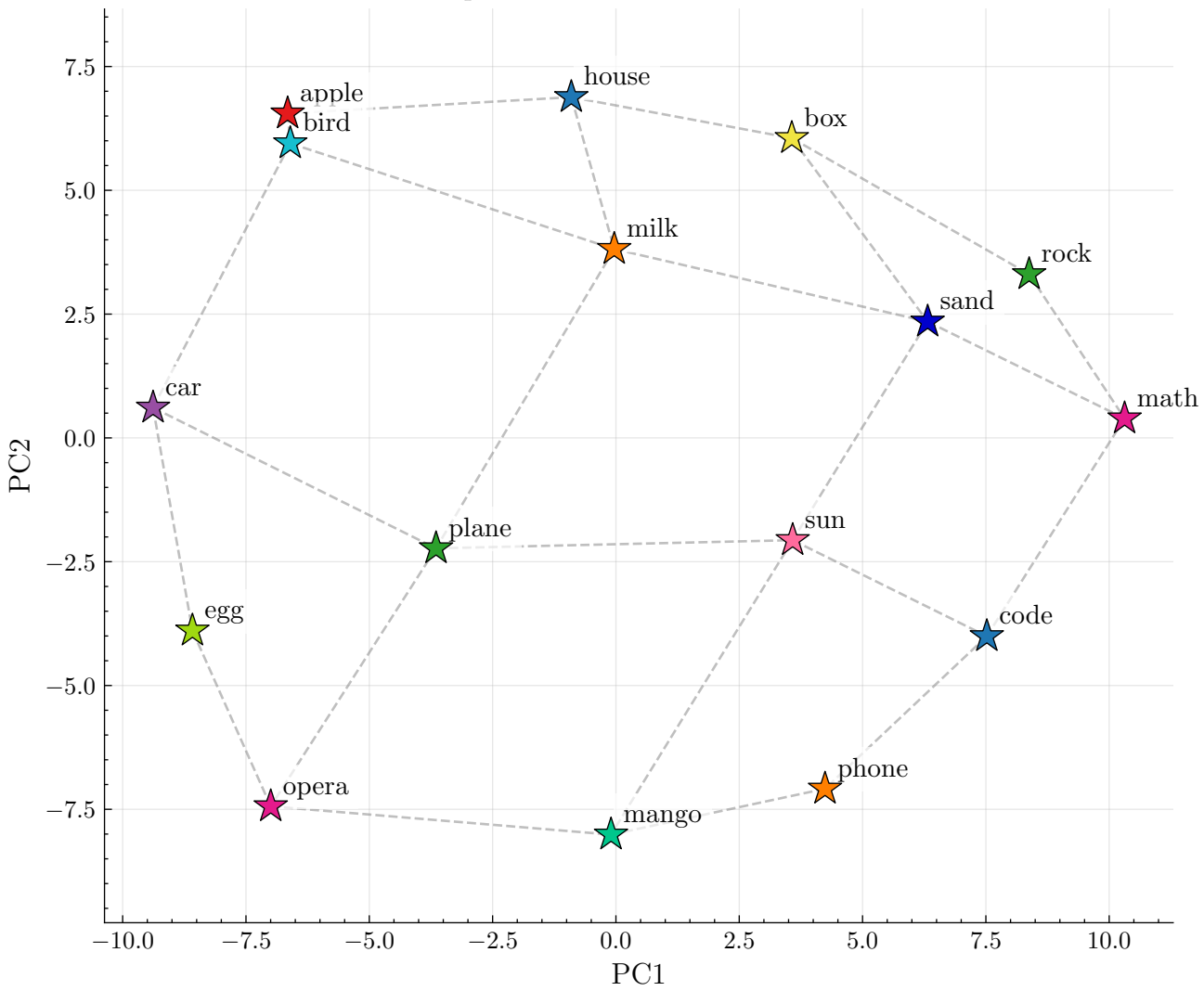
Top 32 Induction Heads Ablated
