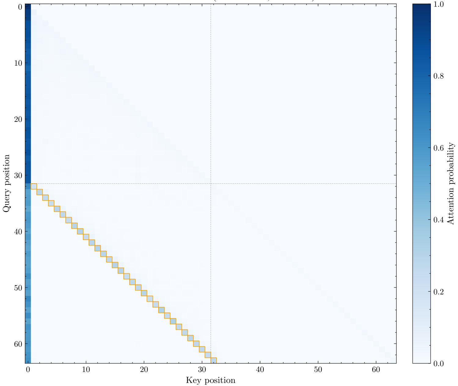
Induction Head: L22H14 (Score: 0.290, Rank: 22)
