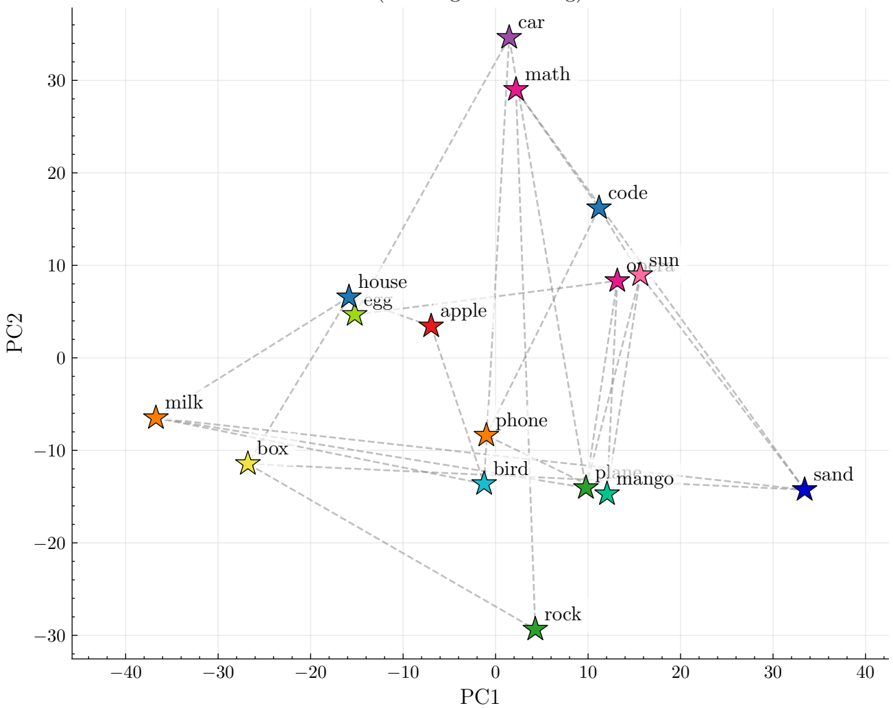
Random Embeddings (No Neighbor Mixing)
