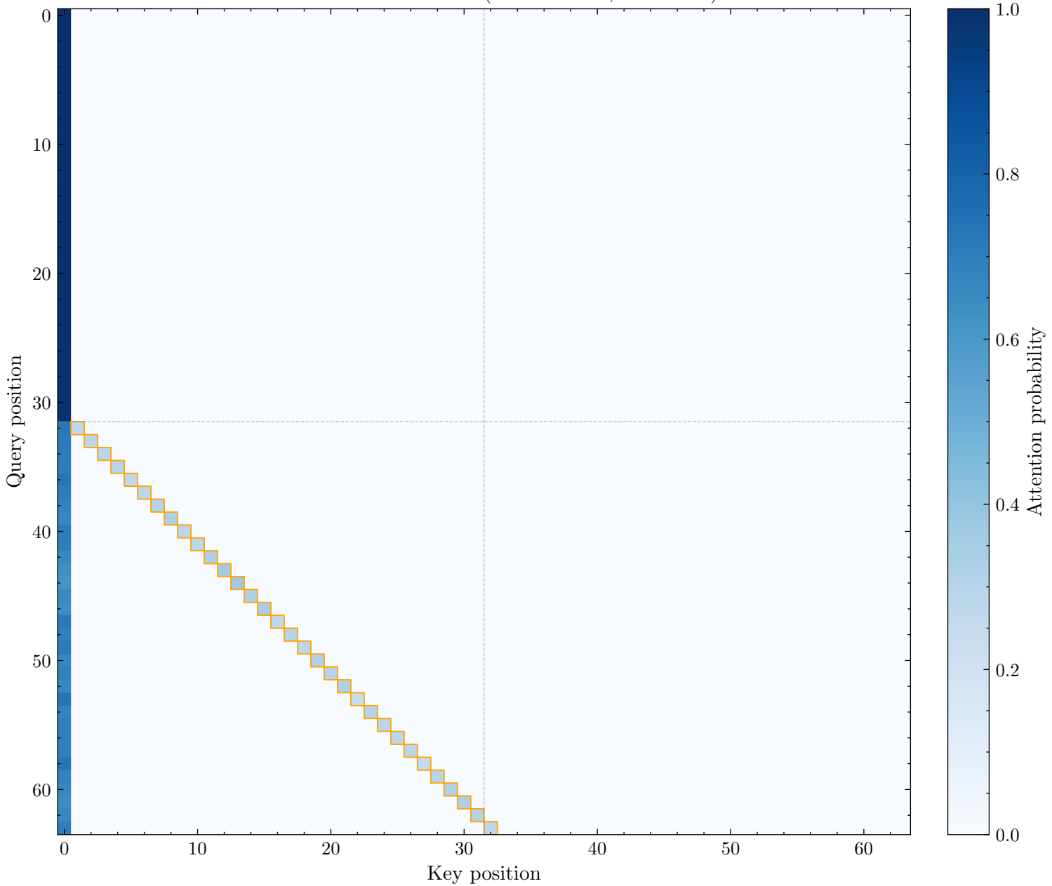
Induction Head: L2H25 (Score: 0.321, Rank: 19)
