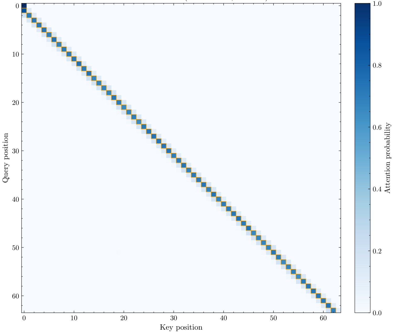
Prev Token Head: L0H2 (Score: 0.709, Rank: 1)
