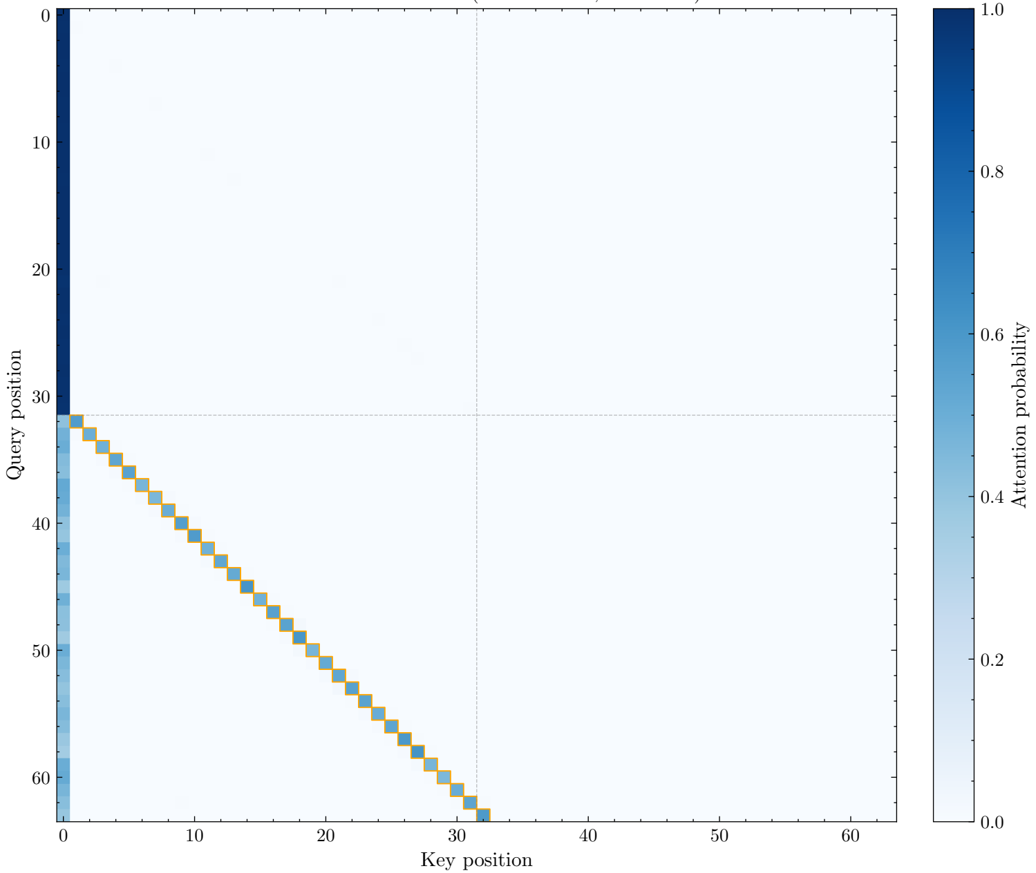
Induction Head: L5H8 (Score: 0.545, Rank: 10)
