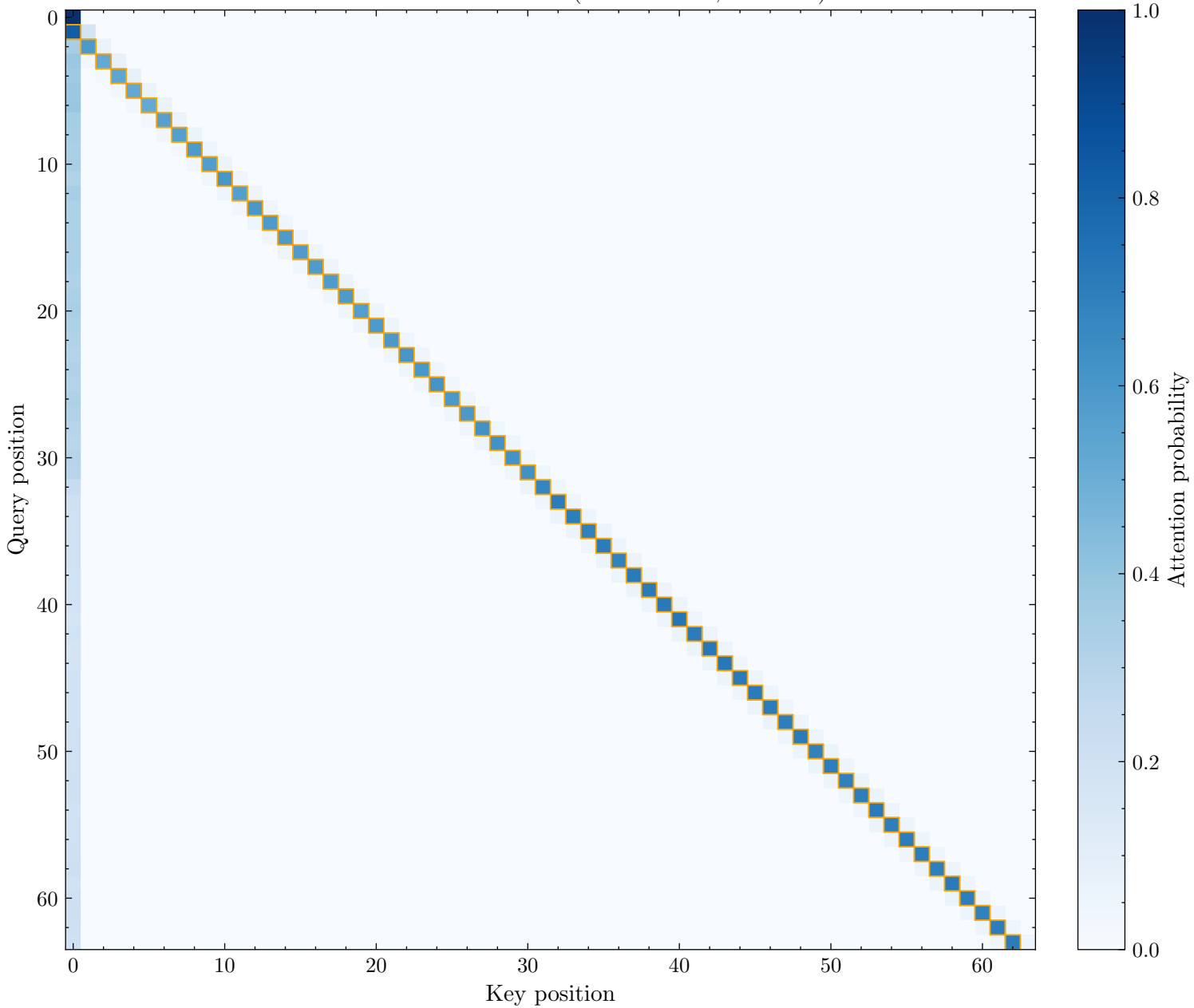
Prev Token Head: L14H26 (Score: 0.647, Rank: 2)
