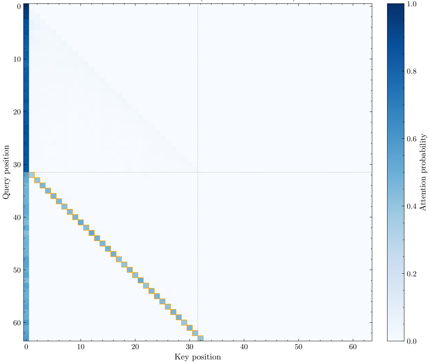
Induction Head: L26H15 (Score: 0.461, Rank: 14)
