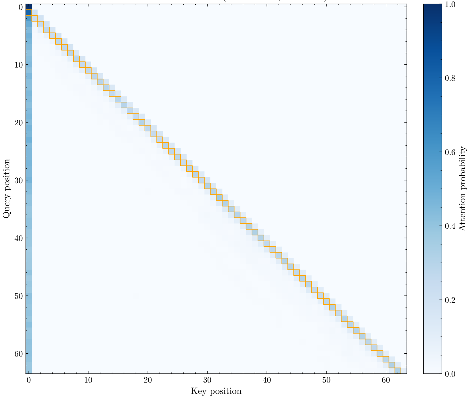
Prev Token Head: L11H16 (Score: 0.292, Rank: 13)
