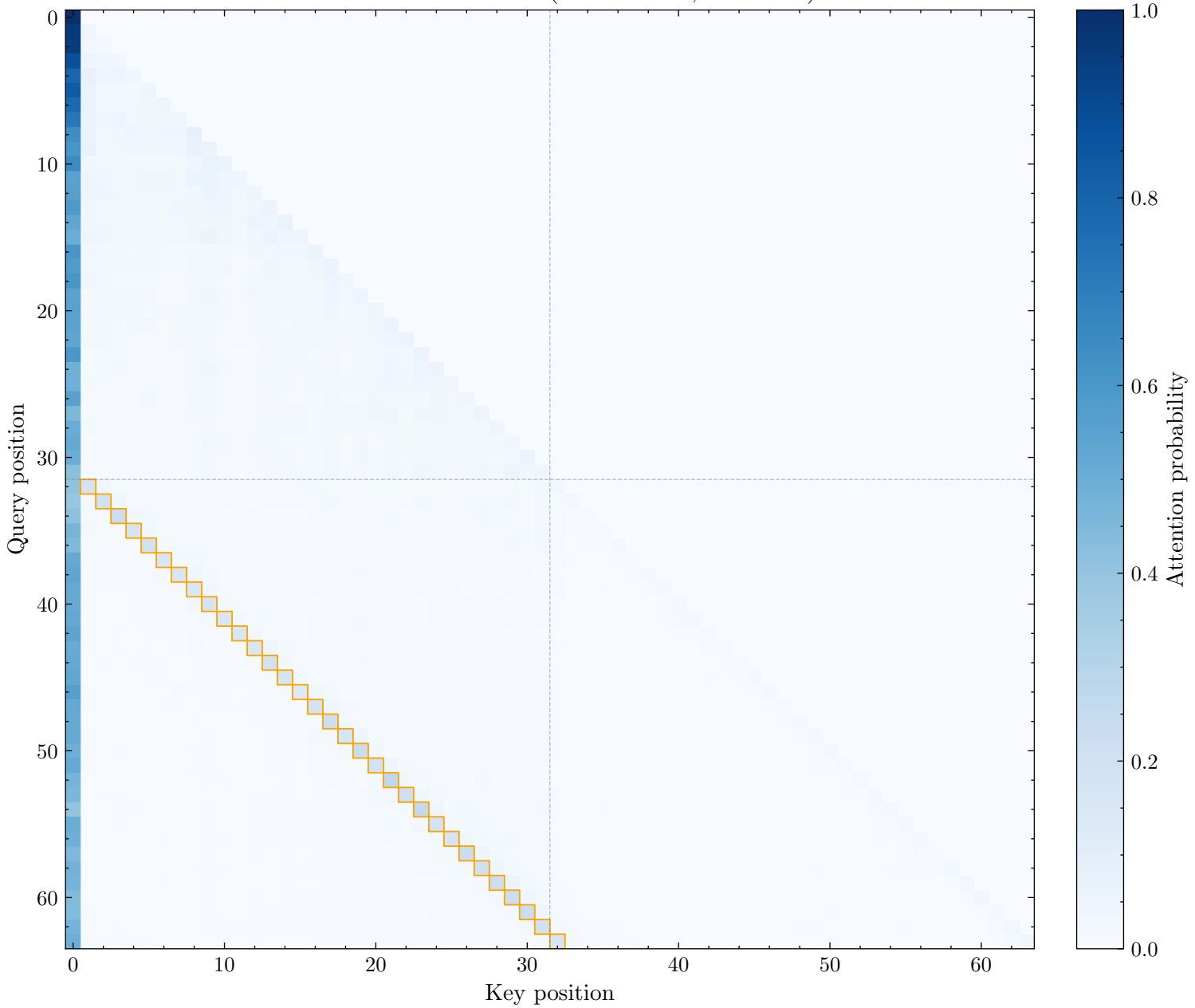
Induction Head: L19H0 (Score: 0.198, Rank: 32)
