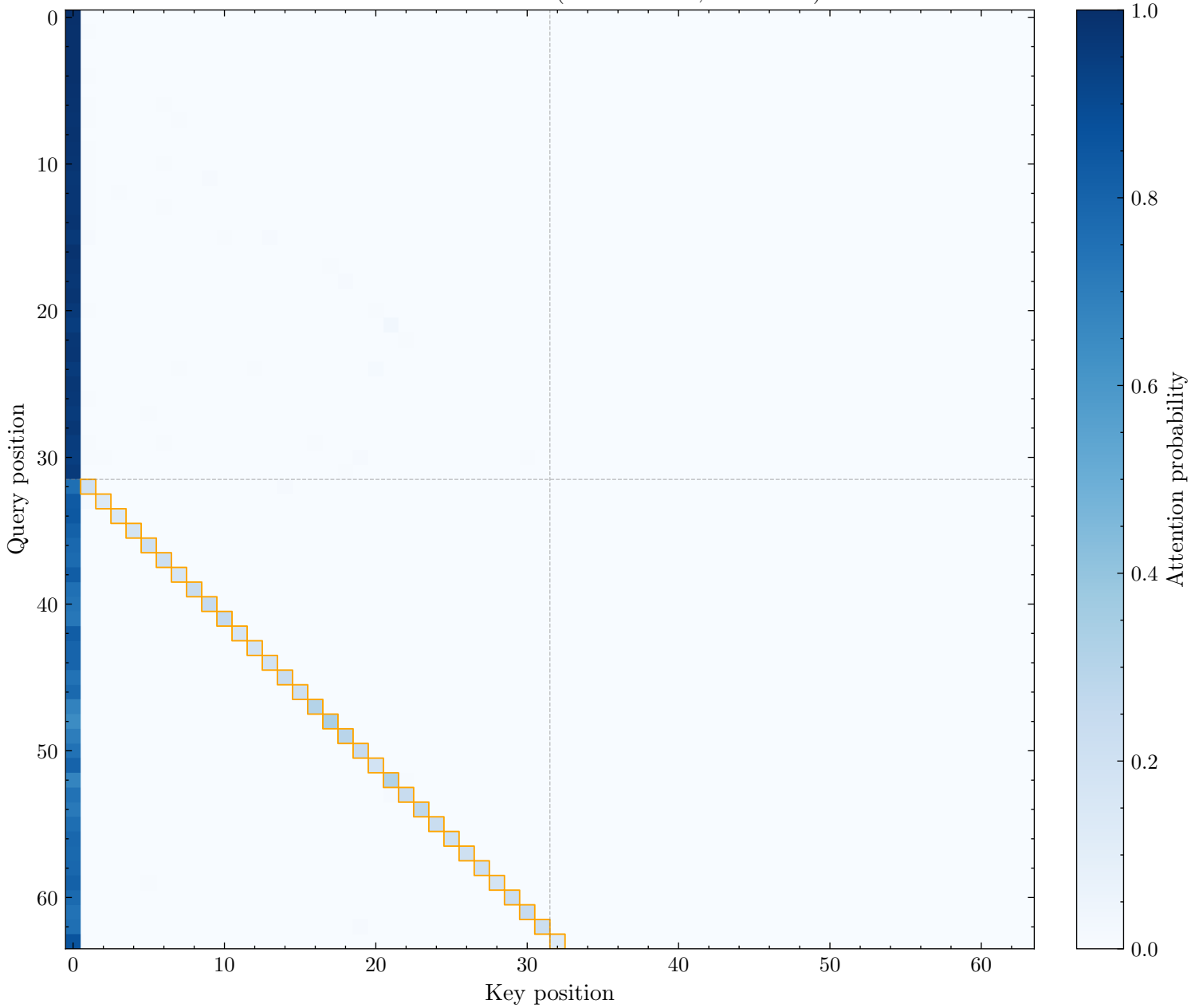
Induction Head: L16H23 (Score: 0.241, Rank: 29)
