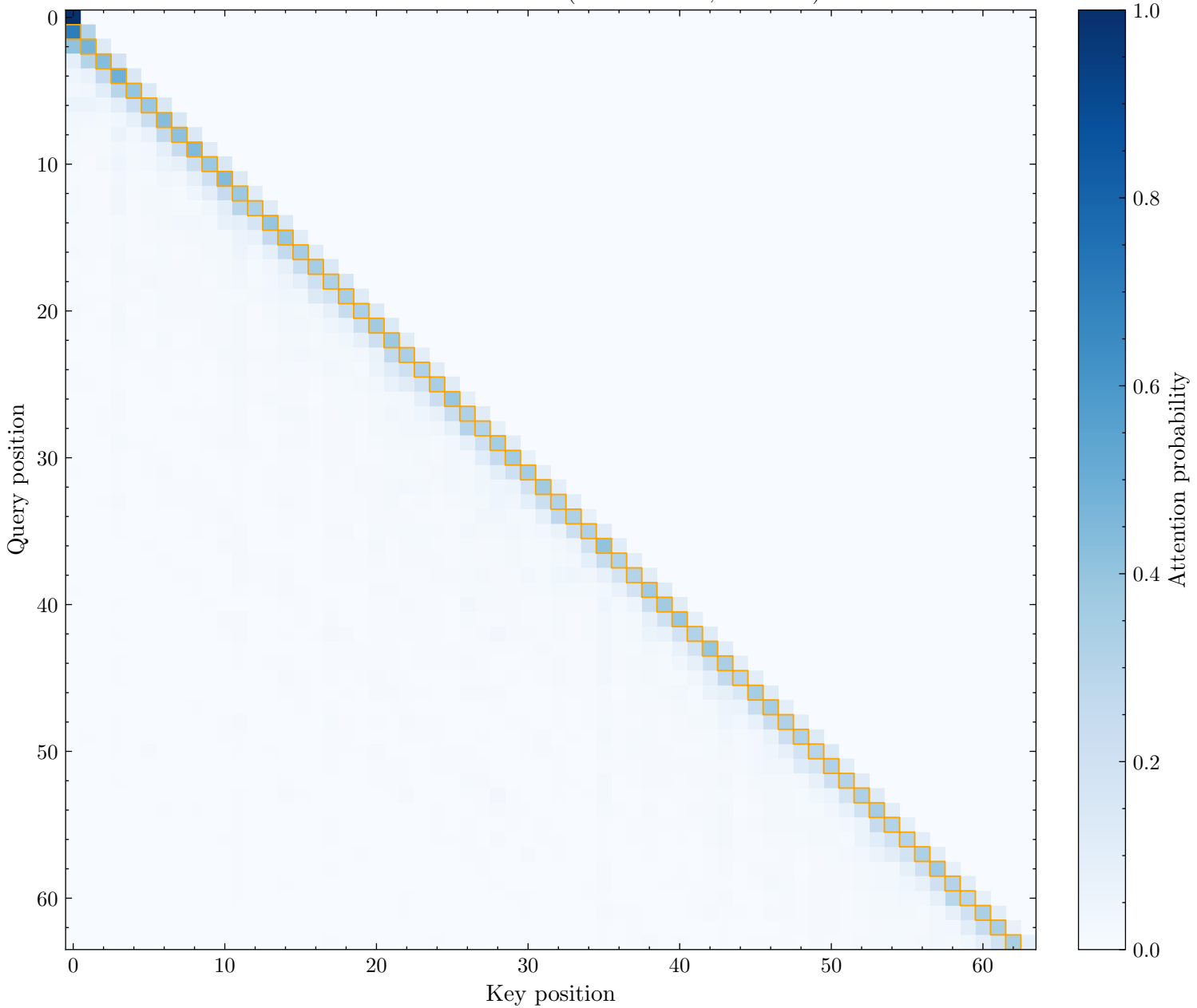
Prev Token Head: L0H24 (Score: 0.359, Rank: 9)
