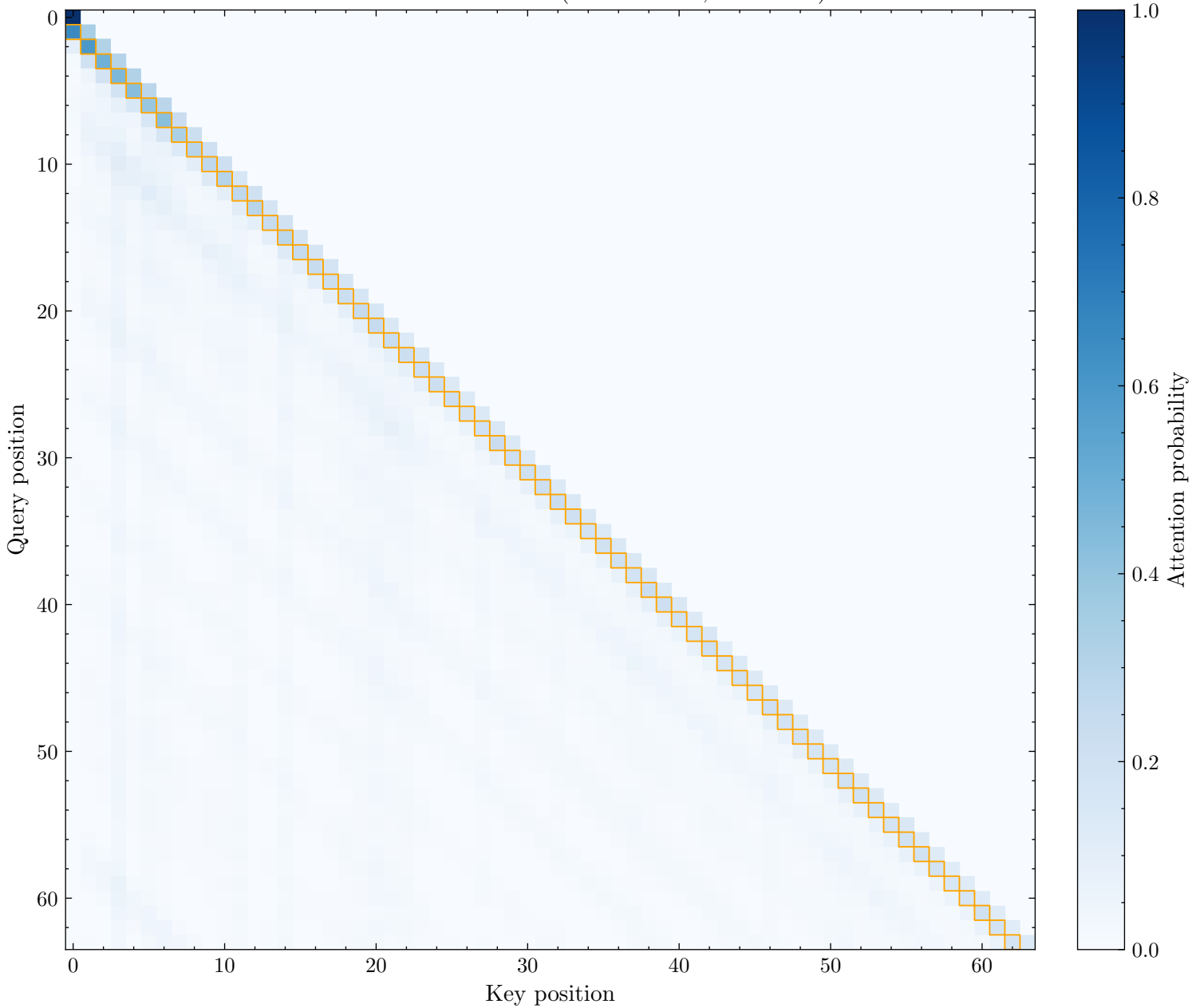
Prev Token Head: L1H30 (Score: 0.243, Rank: 25)
