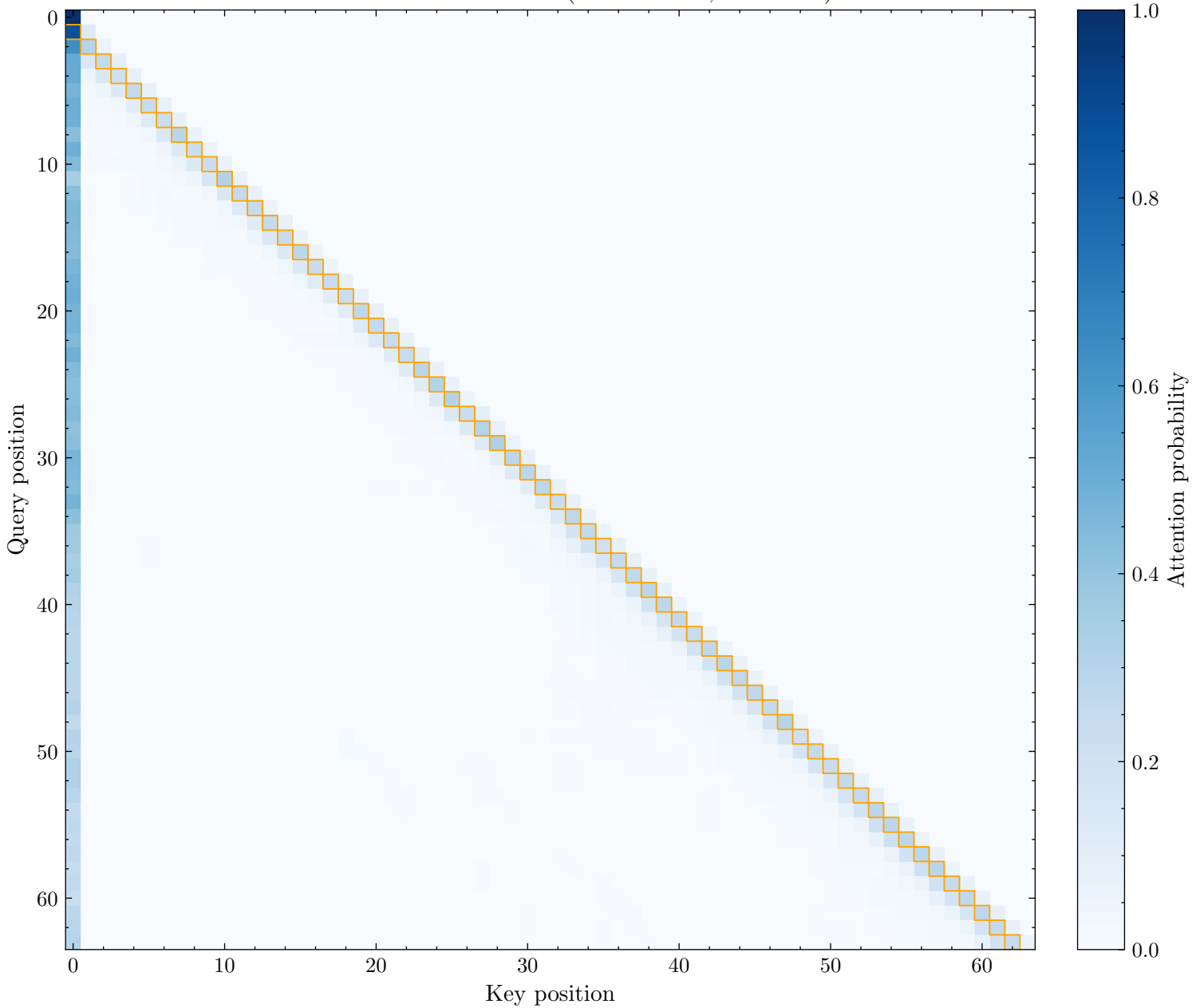
Prev Token Head: L12H16 (Score: 0.272, Rank: 19)
