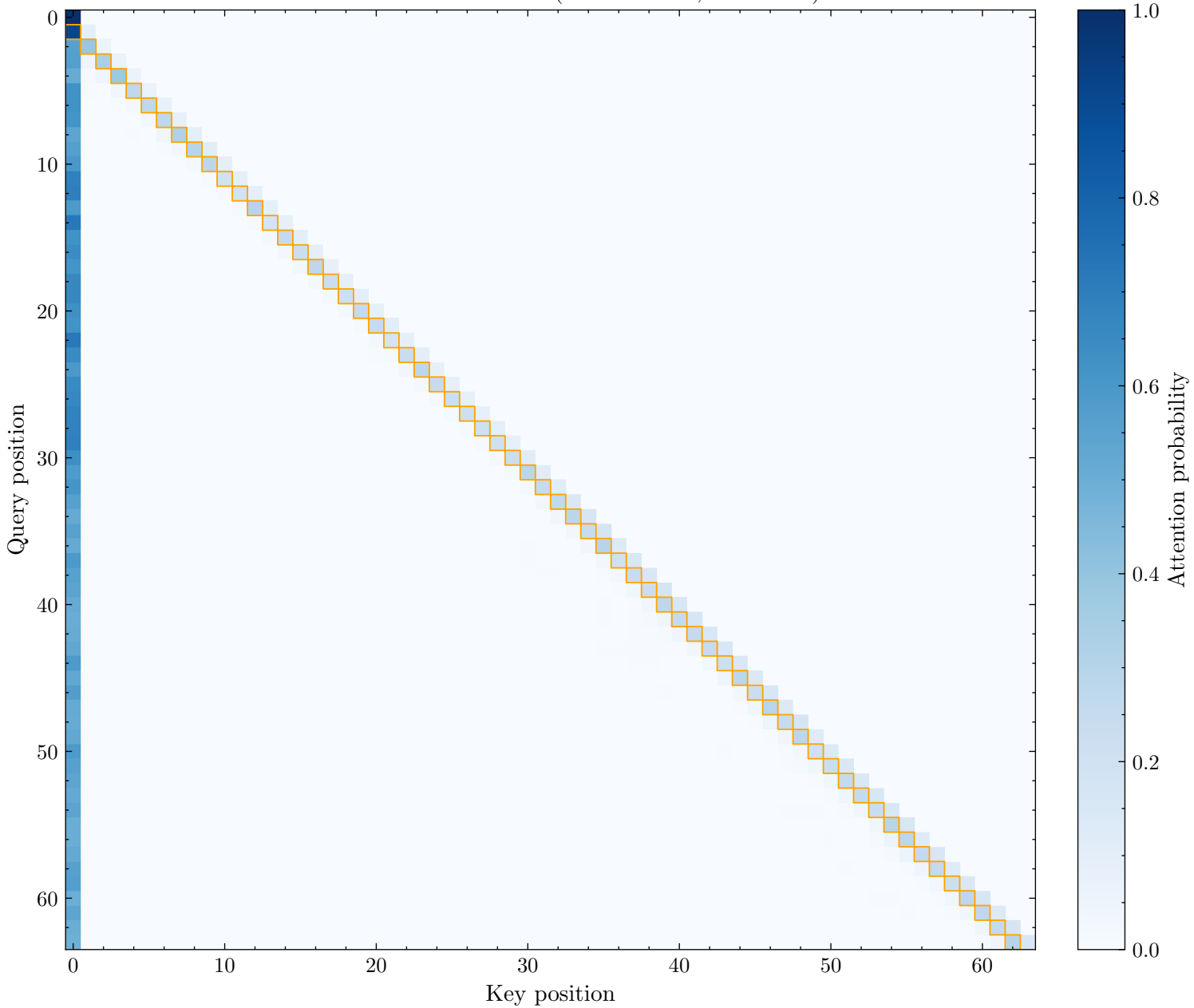
Prev Token Head: L6H8 (Score: 0.265, Rank: 22)
