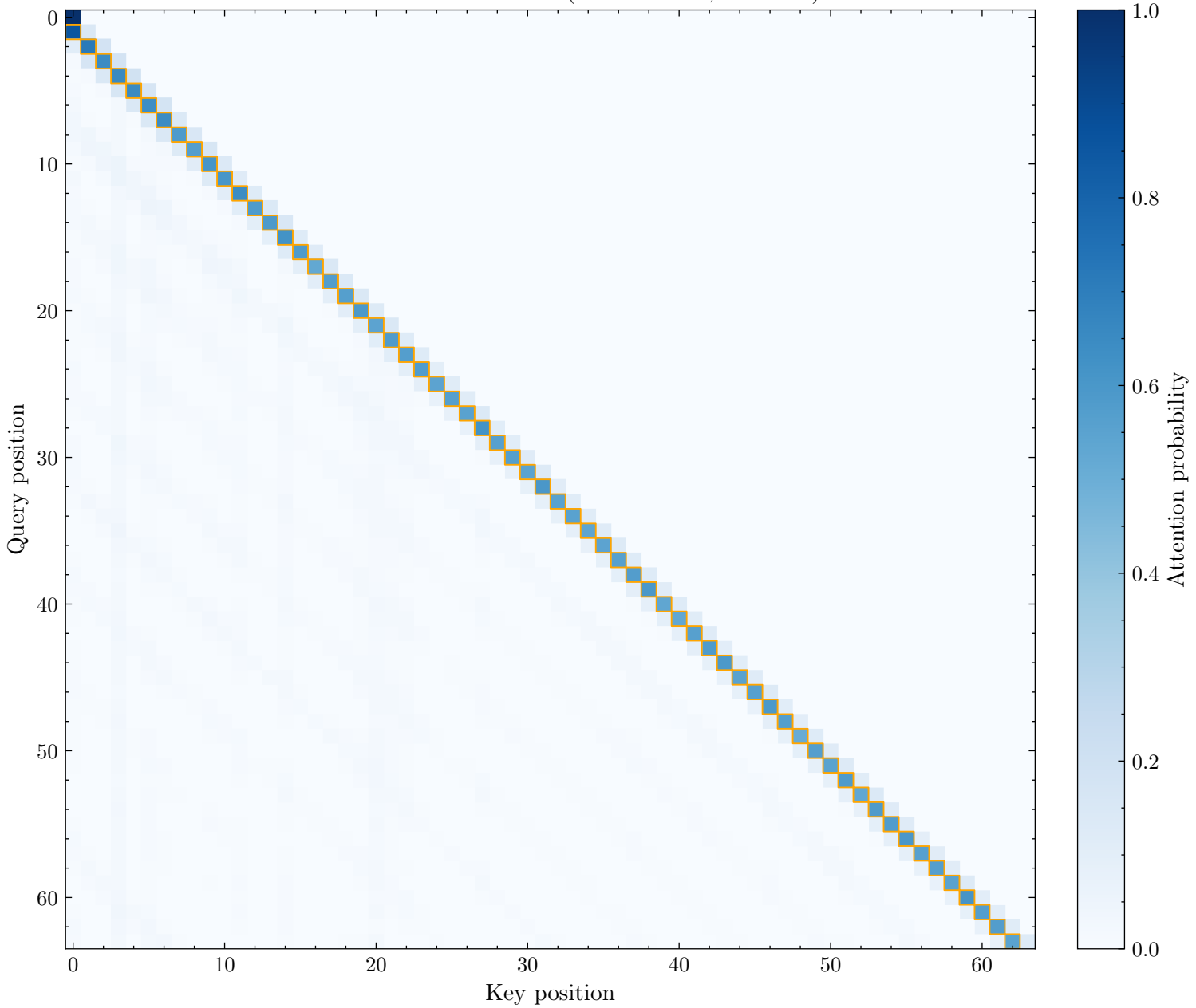
Prev Token Head: L1H20 (Score: 0.583, Rank: 3)
