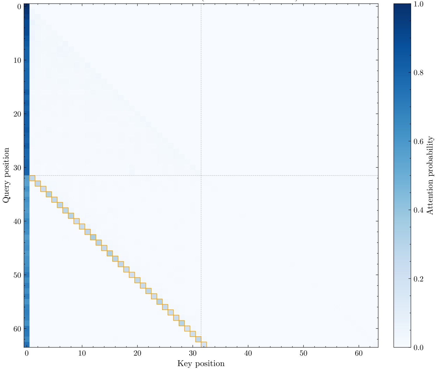
Induction Head: L27H7 (Score: 0.280, Rank: 24)
