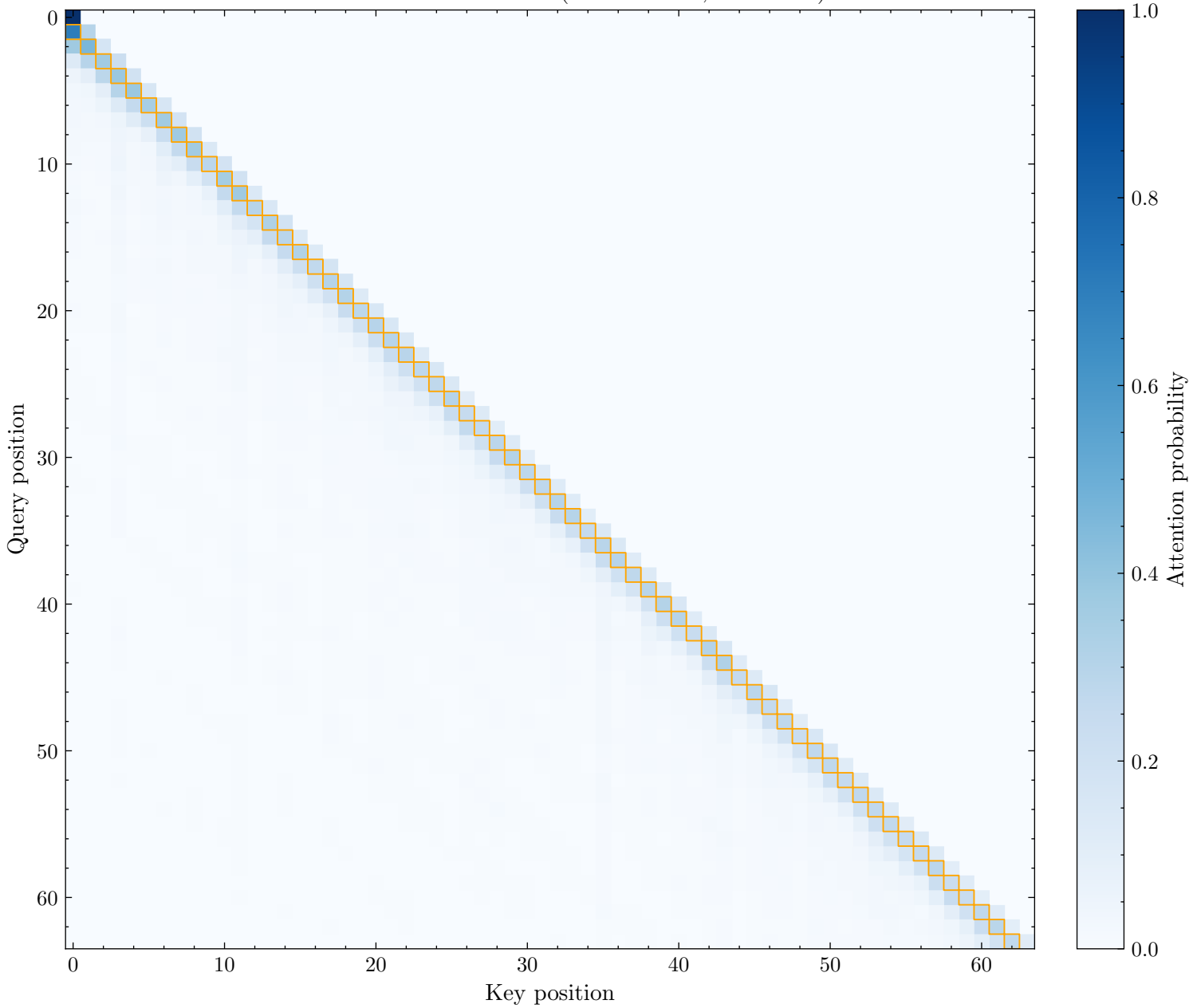
Prev Token Head: L0H26 (Score: 0.300, Rank: 12)
