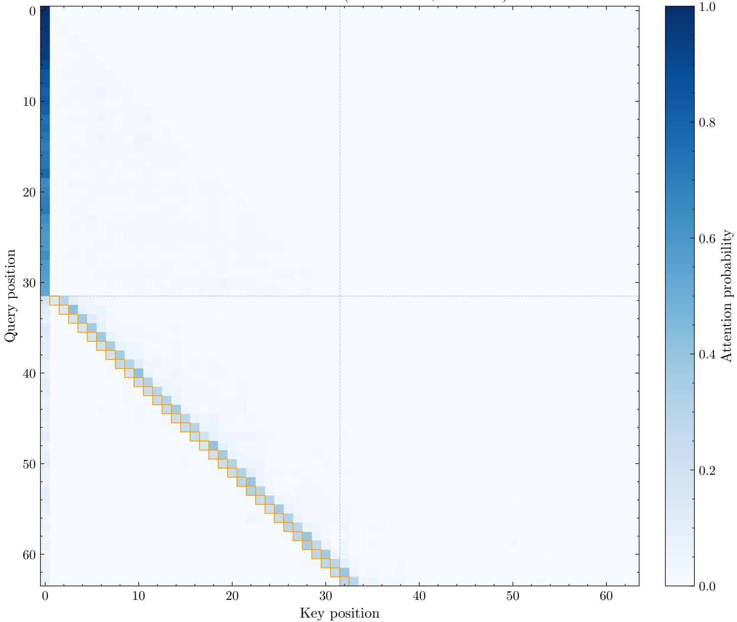
Induction Head: L10H13 (Score: 0.244, Rank: 27)
