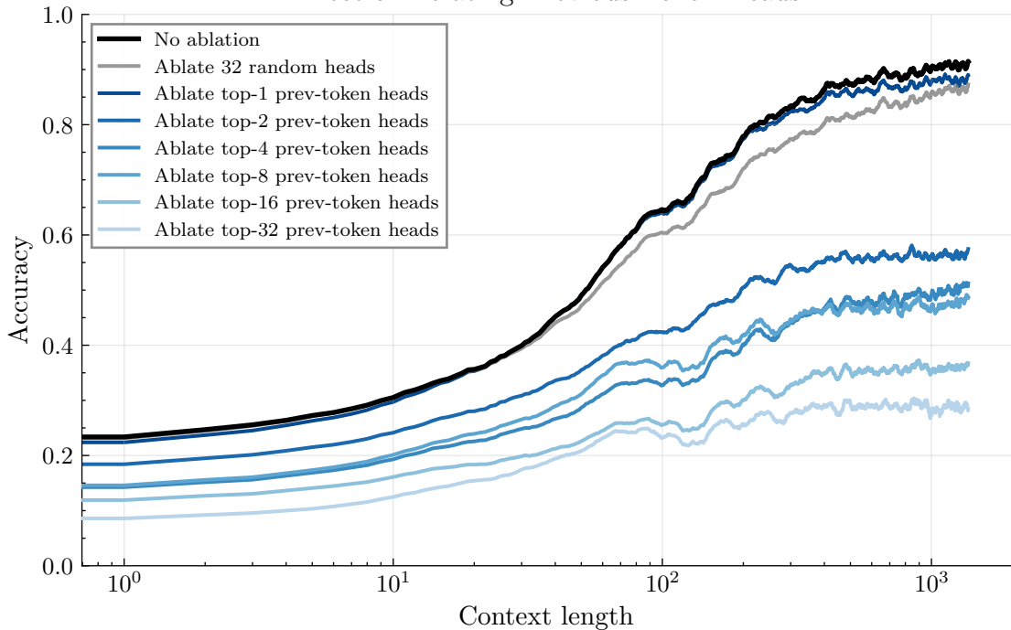
Effect of Ablating Previous-Token Heads
