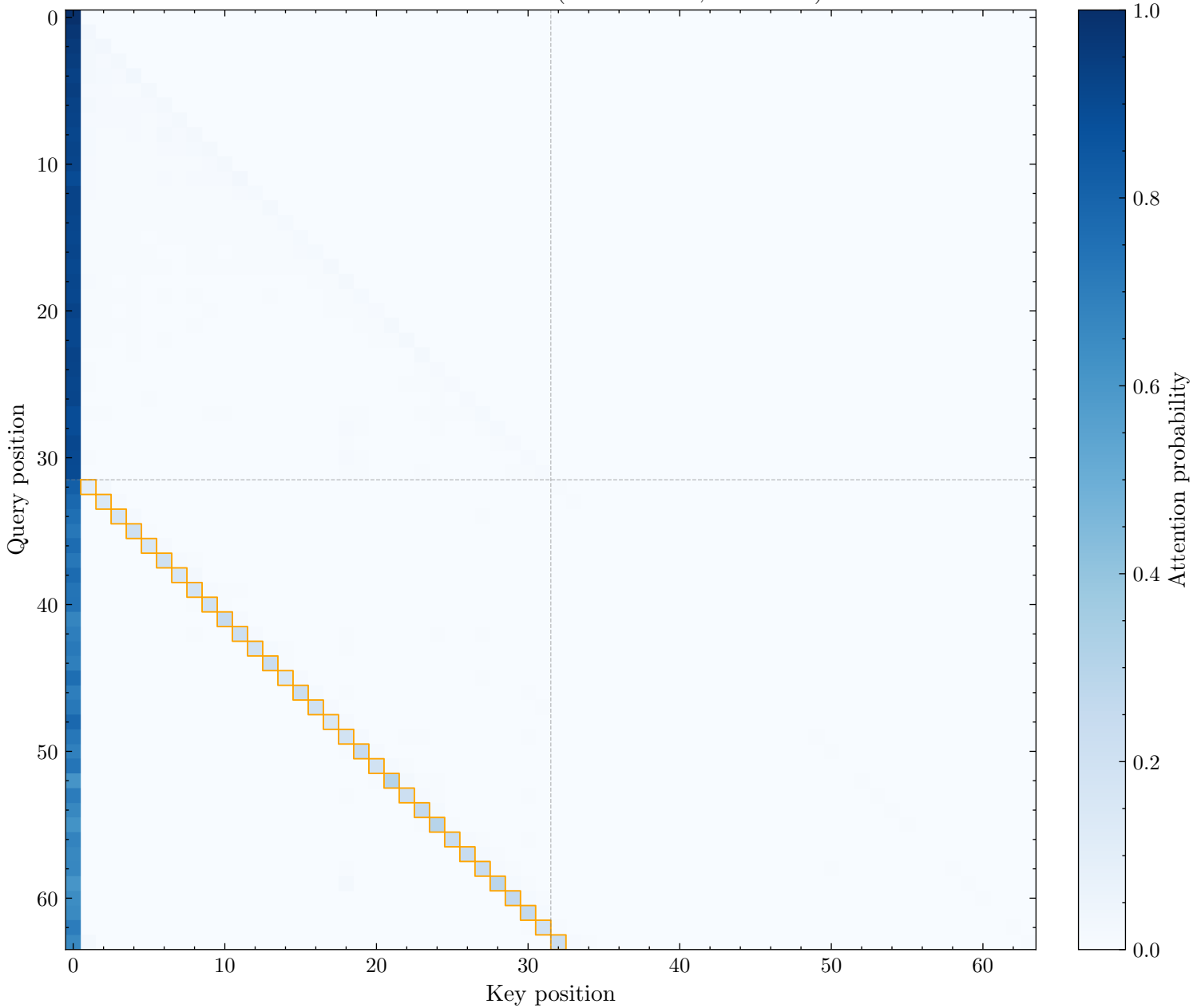
Induction Head: L20H13 (Score: 0.231, Rank: 30)
