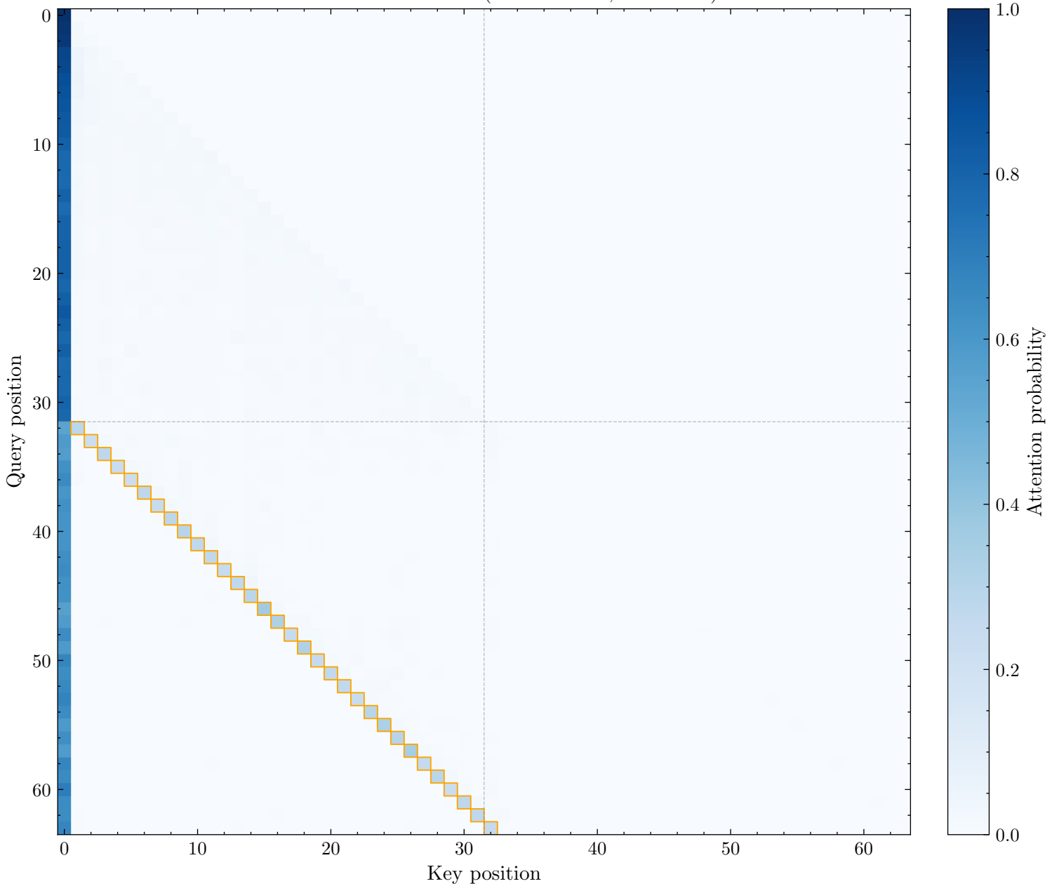
Induction Head: L27H5 (Score: 0.290, Rank: 23)
