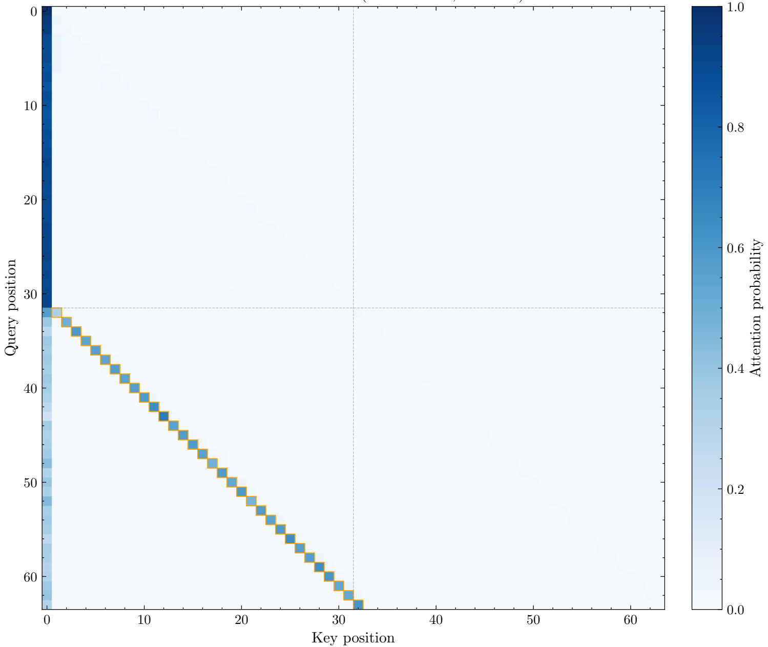
Induction Head: L24H27 (Score: 0.571, Rank: 8)
