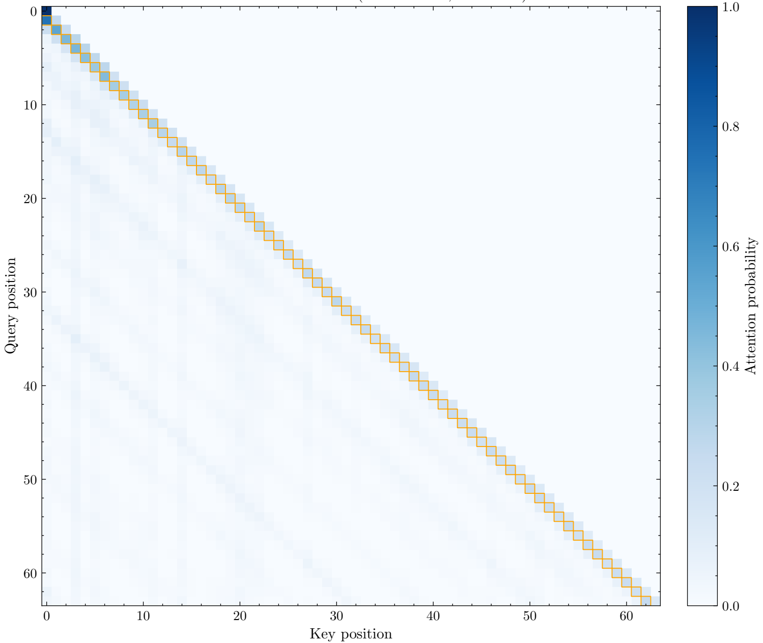
Prev Token Head: L1H24 (Score: 0.275, Rank: 17)
