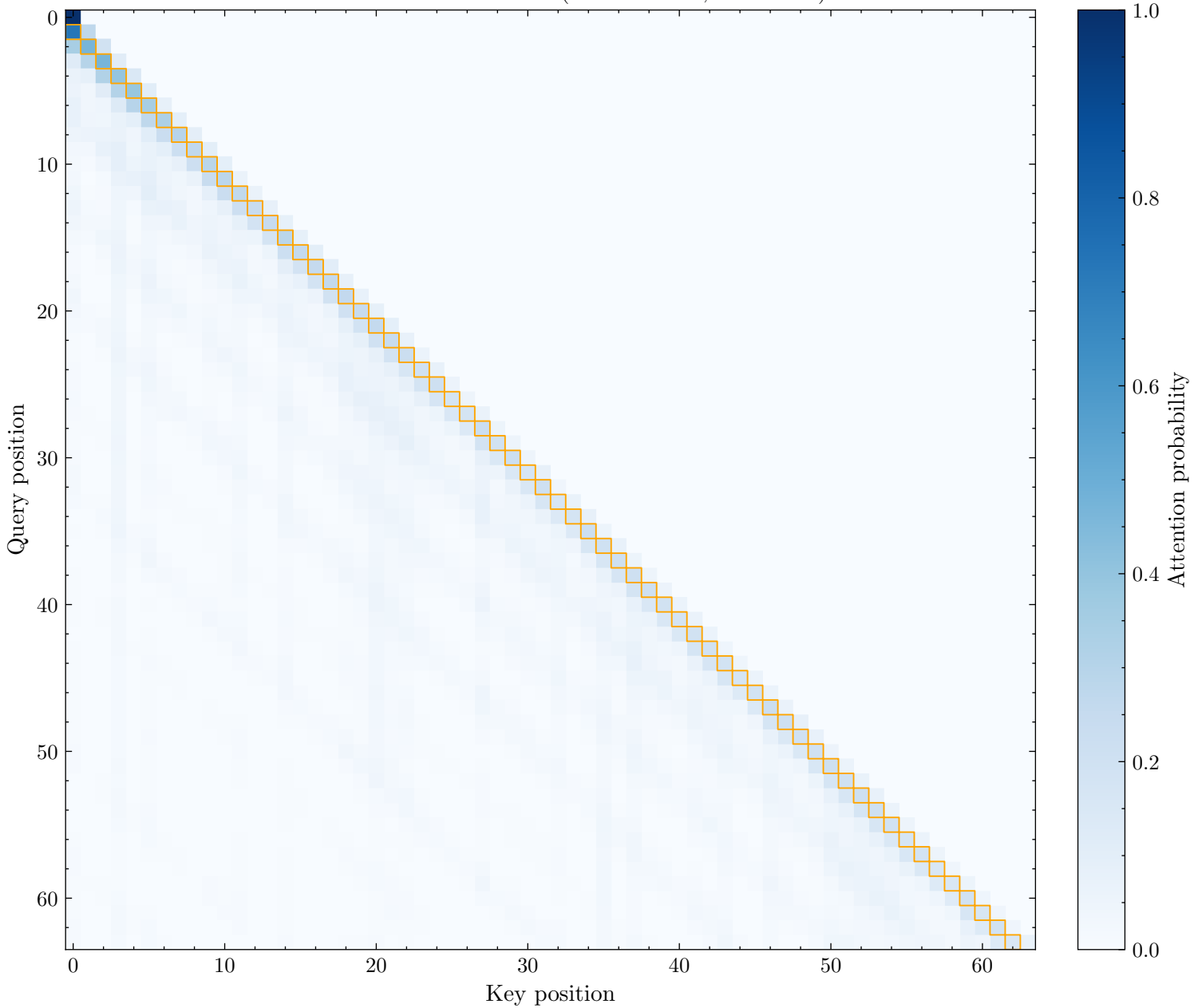
Prev Token Head: L0H29 (Score: 0.236, Rank: 28)
