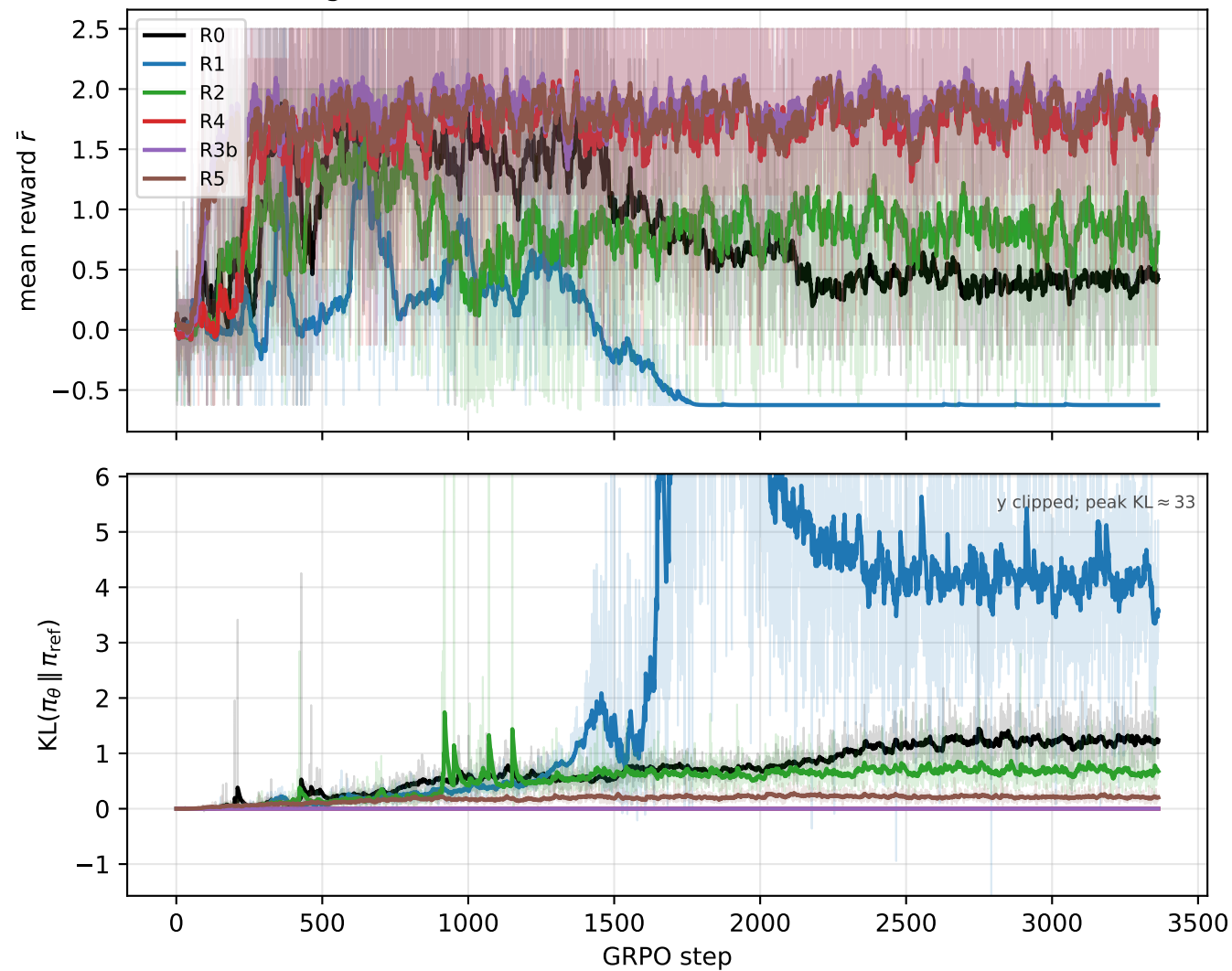
Training reward and reference-KL (faint = raw, bold = EMA)
