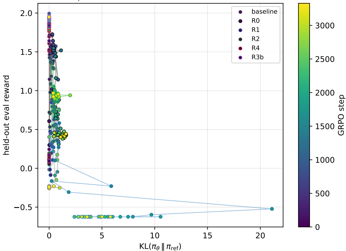
Over-optimisation frontier: KL vs held-out reward
