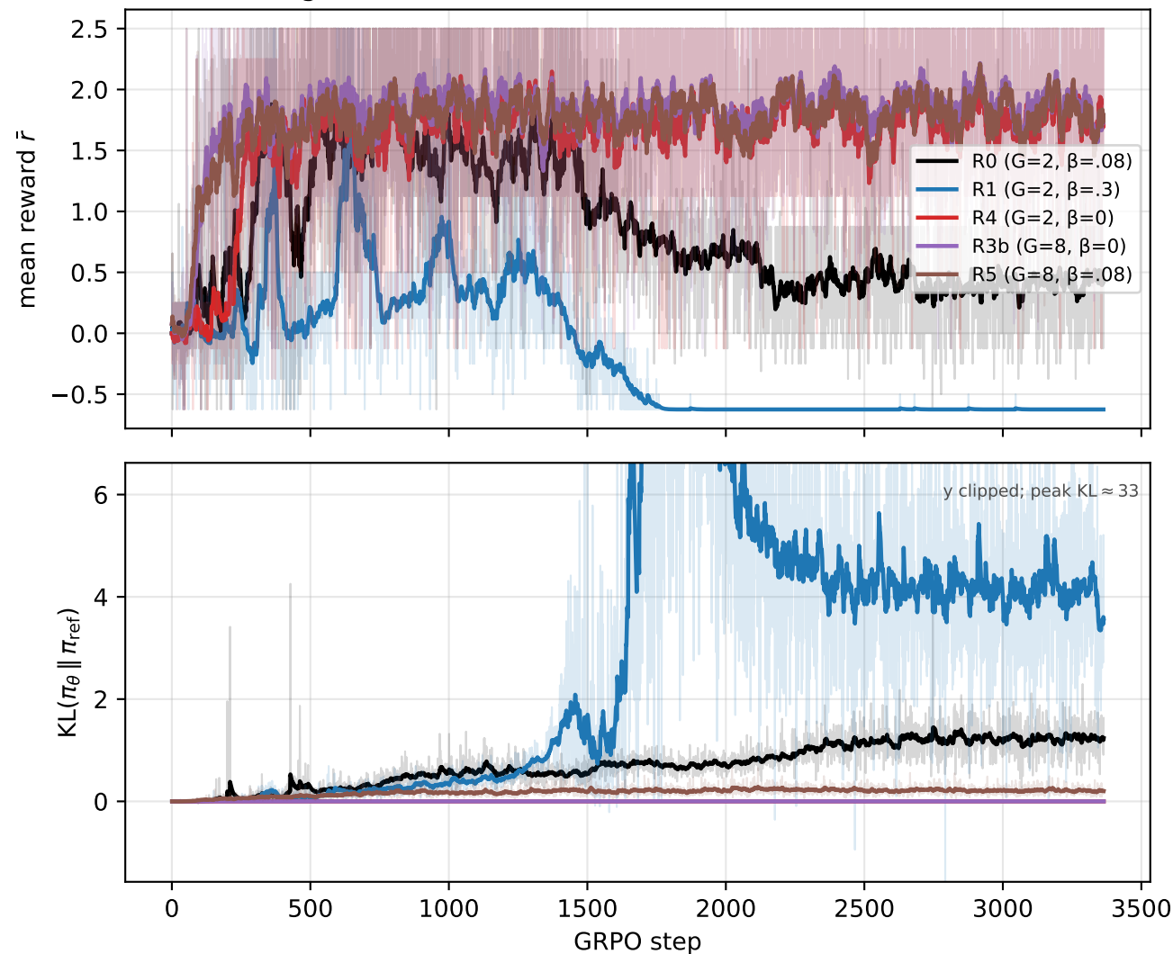
Training reward and reference-KL (faint = raw, bold = EMA)
