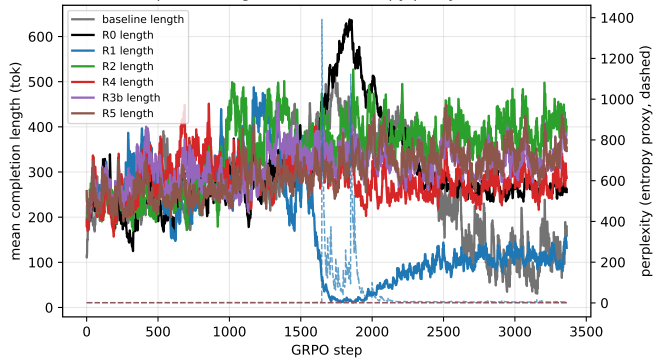
Completion length (solid) + entropy proxy (dashed)
