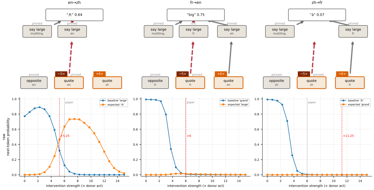
Figure 4: The language swap (raw prompts only; chat pages have no quote nodes). Conventions as in Figure 3; the raw selection has no say large (zh) group, so that readout box is absent in the en→zh panel.
