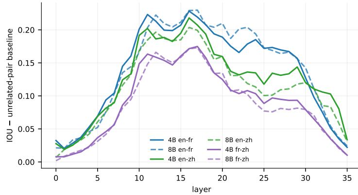
Figure 6: Baseline-subtracted cross-lingual feature overlap by layer (solid: 4B; dashed: 8B, same-recipe transcoders). The paper’s inverted-U and pair ordering reproduce; its cross-scale growth does not.
