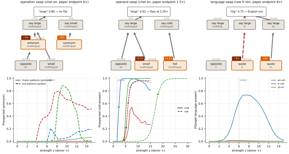
Figure 2: Swap interventions. Top : intervention diagrams with measured supernode readouts (grey percentages; “pinned” = at or below the patch end layer \ell , clamped by the protocol); badges give the paper’s steering multiples. Bottom : strength ladders, P(\text{expected answer}) vs. donor multiple s , with the paper endpoint dotted. Left: the operation swap under the constrained protocol (solid, flat) vs. the live-attention probe (dashed) — the QK-mediated channel. Middle: the operand swap crosses in all six configurations (dots mark crossovers; raw-zh at 18\times ). Right: the language swap peaks near the paper’s own 6\times and saturates; fr \rightarrow en’s curve tracks “large” while the actual output is the paper’s token “big” ( 0.753 at 6\times ).
