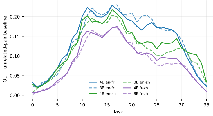
Figure 3: Baseline-subtracted cross-lingual feature overlap by layer (solid: 4B; dashed: 8B, same-recipe transcoders). The paper’s inverted-U and pair ordering reproduce; its cross-scale growth does not.
