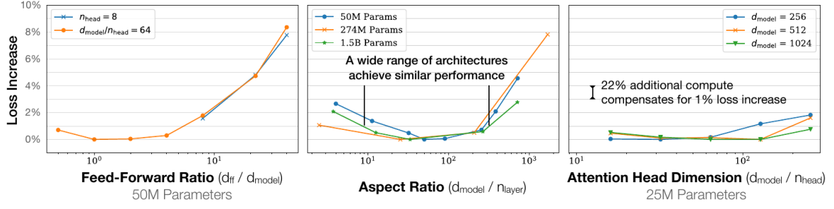
Figure 1: Controlled shape sweeps at fixed non-embedding parameter count. The three panels vary the FFN ratio, depth-to-width aspect ratio, and attention-head dimension. They report the increase in loss relative to the model-size baseline. Reproduced from Figure 5 of Kaplan et al. [5].
