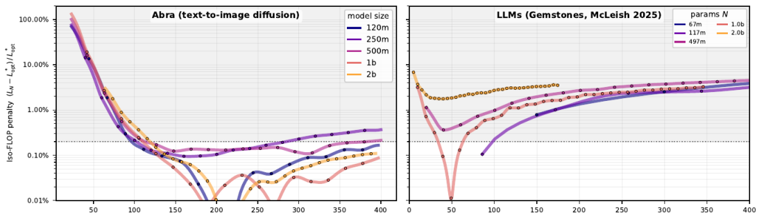
Figure 13: Relative IsoFLOP loss penalty versus TPP. The Abra curves (left) are comparatively flat toward smaller models and more data, but rise sharply when TPP is too small; the LLM comparison (right) illustrates that this asymmetry is empirical rather than a property of the counting convention. Reproduced from Figure 6 of Chickering et al. [1].
