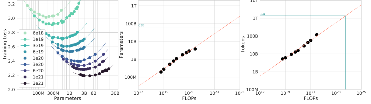
Figure 9: IsoFLOP curves. Left: final loss versus model size at nine fixed budgets; dashed parabolas locate each minimum. Center and right: the minima against compute, with power-law fits extrapolated to Gopher’s budget. Reproduced from Figure 3 of Hoffmann et al. [3].
