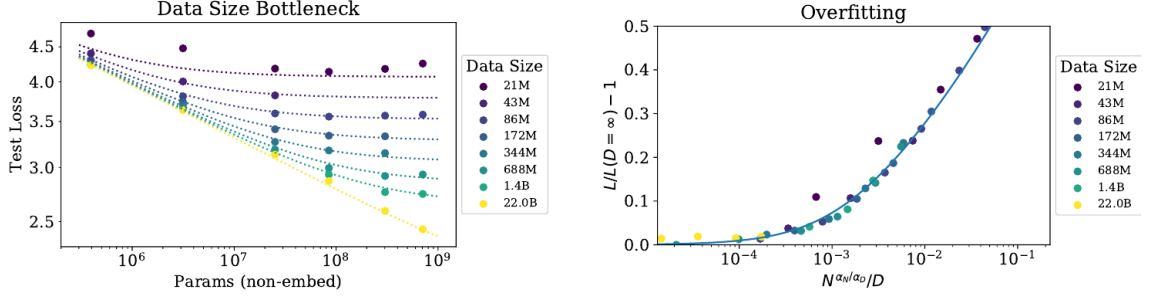
Figure 5: Joint model-data scaling. Left: at fixed finite D , increasing model size eventually reaches a data-limited plateau. Right: measurements from different N_K and D collapse when the relative finite-data penalty \mathcal{L}(N_K, D)/\mathcal{L}(N_K, \infty) - 1 is plotted against N_K^{\alpha_N/\alpha_D}/D . Both horizontal axes are logarithmic; the left loss axis is logarithmic, while the right relative-penalty axis is linear. Reproduced from Figure 9 of Kaplan et al. [5].
