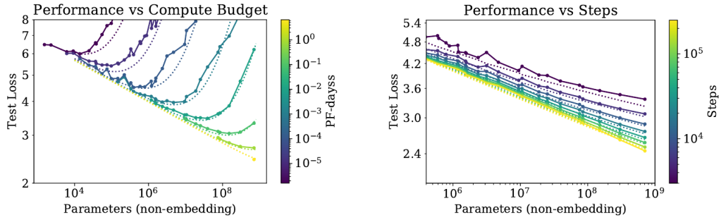
Figure 7: Loss versus non-embedding model size at fixed compute budgets (left) and fixed numbers of training steps (right). Solid curves are experiments and dotted curves are predictions from the learning-curve model. Reproduced from Figure 11 of Kaplan et al. [5].
