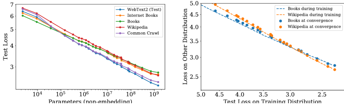
Figure 4: Generalization from WebText2 to other text distributions. Left: every evaluation distribution improves smoothly with non-embedding model size. Right: losses measured during training and at convergence lie on nearly the same mapping from WebText2 loss to target-distribution loss. Reproduced from Figure 8 of Kaplan et al. [5].
