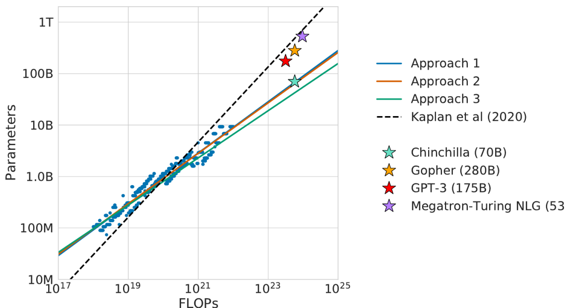
Figure 11: Chinchilla’s three fitting approaches predict a substantially smaller compute-optimal model than the Kaplan extrapolation at large budgets. The marked Chinchilla point lies near the revised frontier. Reproduced from Figure 1 of Hoffmann et al. [3].
