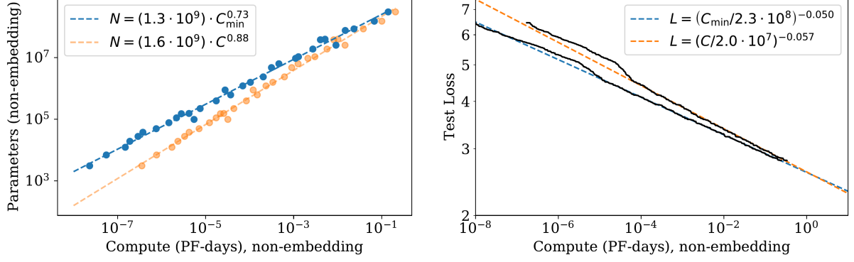
Figure 8: The bottoms of the fixed-budget U-curves versus compute budget. Left: the optimal model size N_K^* ; blue uses C_{\min} , orange raw compute at B = 2^{19} . Right: the lowest loss \ell^* ; the lower curve uses C_{\min} , the upper curve raw compute. Its legend scale 2.3 \times 10^8 differs from the summary value in Eq. (34). Reproduced from Figures 14 (left) and 13 of Kaplan et al. [5].
