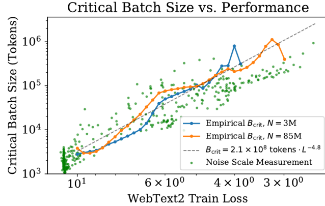
Figure 6: Critical batch size measured for 3M- and 85M-parameter models, together with gradient-noise-scale measurements. The model-size curves approximately share a loss-dependent trend. Reproduced from Figure 10 of Kaplan et al. [5].
