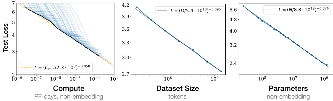
Figure 3: The three one-dimensional scaling experiments, displayed left-to-right as compute, dataset size, and non-embedding model size. The horizontal and loss axes use logarithmic scales; the loss ticks are labelled with loss values rather than their logarithms. A power law is a straight line in these log–log coordinates. The dataset-size panel holds the architecture fixed at the large (n_{\text{layer}}, d_{\text{model}}) = (36, 1280) model, while the model-size panel trains each Transformer on the full WebText2 dataset. The compute panel is instead a lower envelope over checkpoints from many model sizes. The discussion below analyzes dataset size first, then model size, and finally that constructed envelope. Reproduced from Figure 1 of Kaplan et al. [5].
