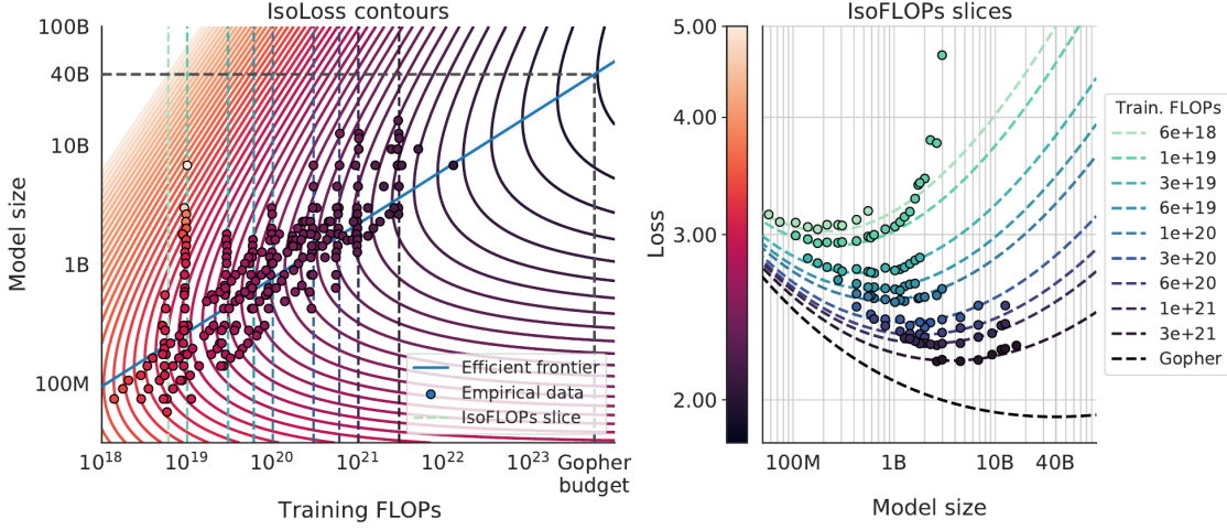
Figure 10: The fitted Chinchilla loss surface (left) and its IsoFLOP slices (right). The blue efficient frontier follows the minimum of each loss contour, while the U-shaped slices expose an interior optimum at fixed compute. Reproduced from Figure 4 of Hoffmann et al. [3].
