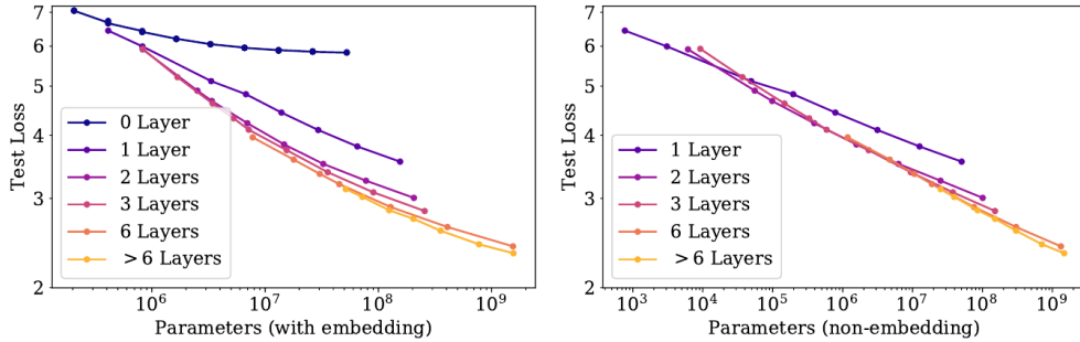
Figure 2: The same family of models indexed by total parameters (left) and non-embedding parameters (right). Including embeddings separates the curves by depth; excluding them collapses models with at least two layers and non-extreme shapes onto a common trend. This establishes a shared scale variable, not by itself a power law. Reproduced from Figure 6 of Kaplan et al. [5].
