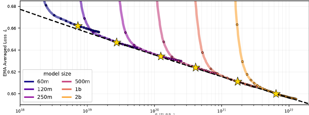
Figure 12: Compute scaling for the Abra model family. At each scale, the compute-optimal checkpoint lies on the common loss frontier; the plotted endpoints support a near-constant visual-data allocation in the measured regime. Reproduced from the upper panel of Figure 1 in Chickering et al. [1].
