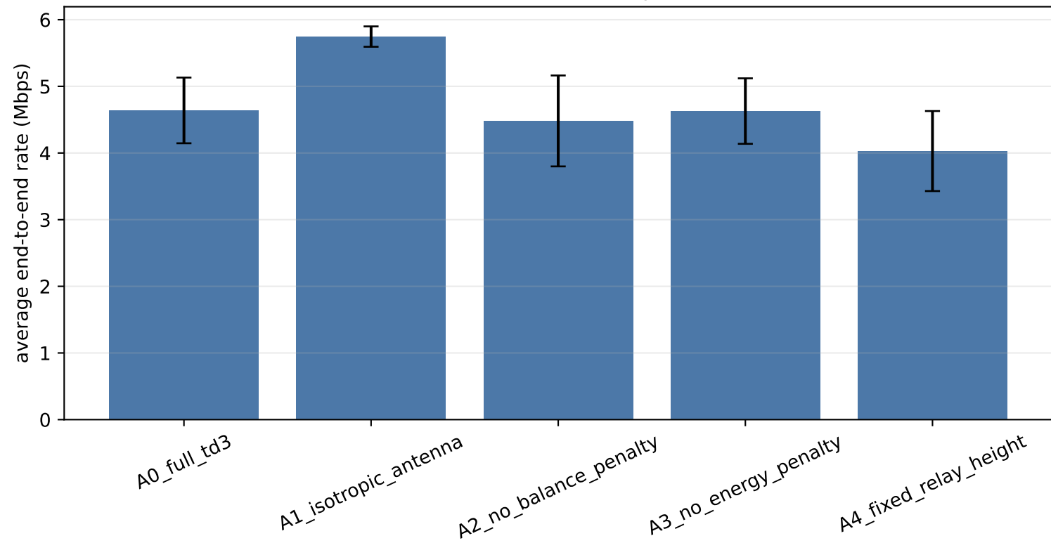
TD3 ablation rate comparison
