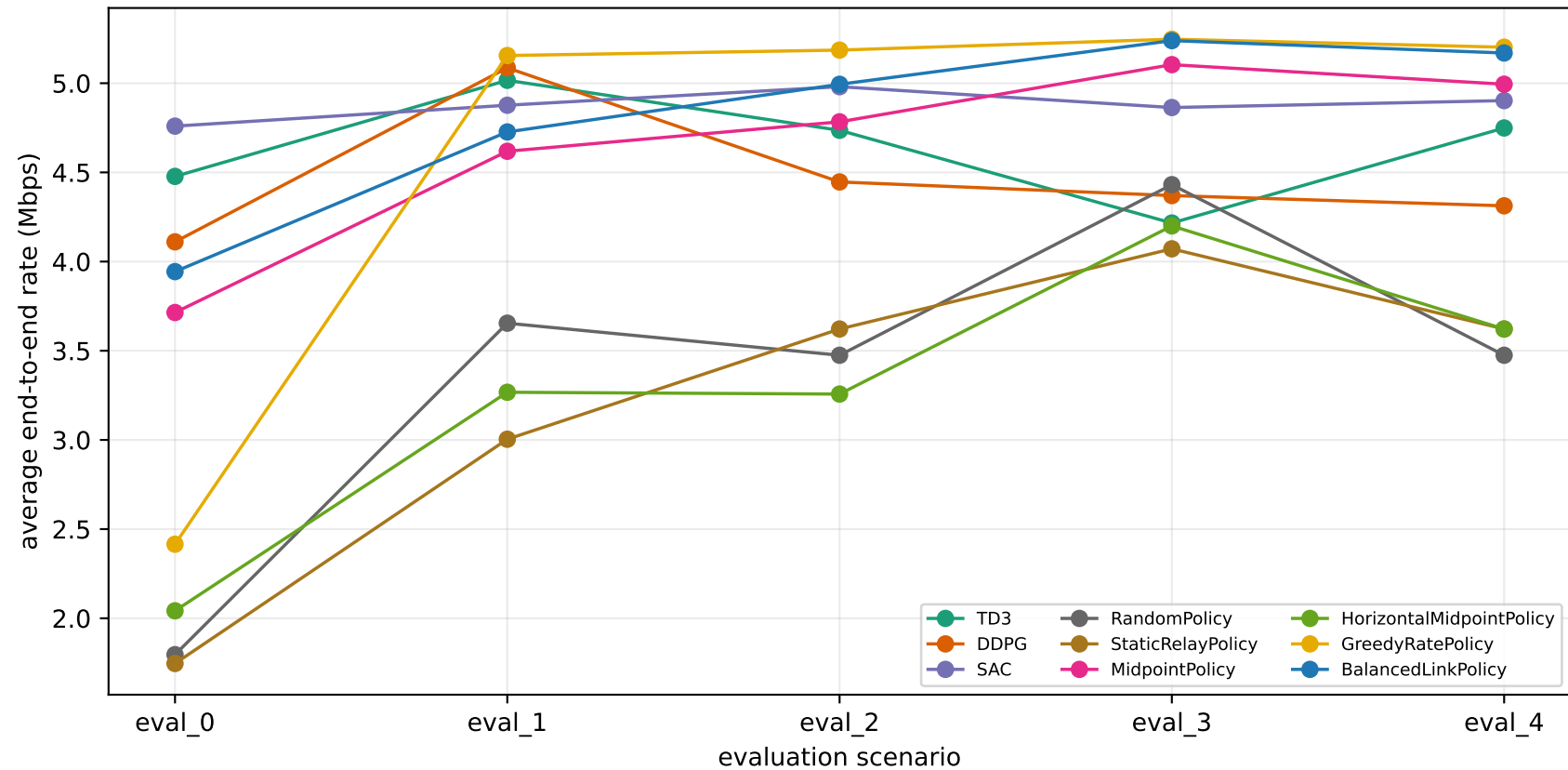
Scenario-wise algorithm performance
