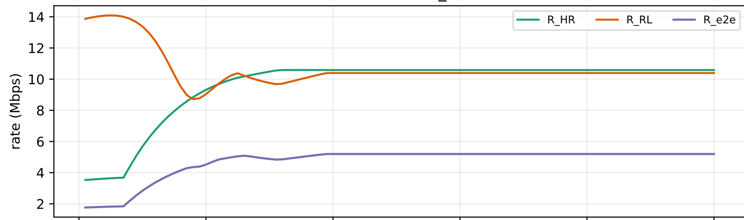
SAC on eval_0
