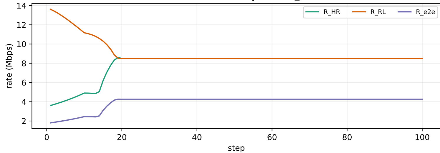
BalancedLinkPolicy on eval_0
