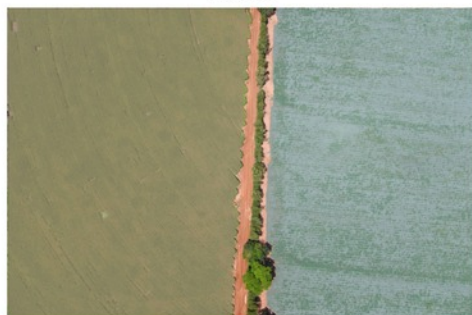
iou_0.92 masks=3
