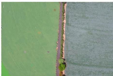
iou_0.70 masks=11
