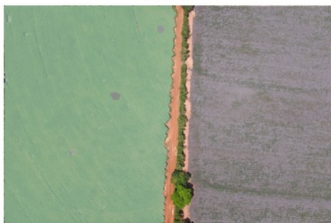
points_16 masks=5
