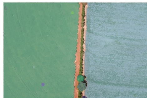
iou_0.82 masks=10
