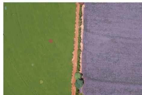
points_32 masks=12
