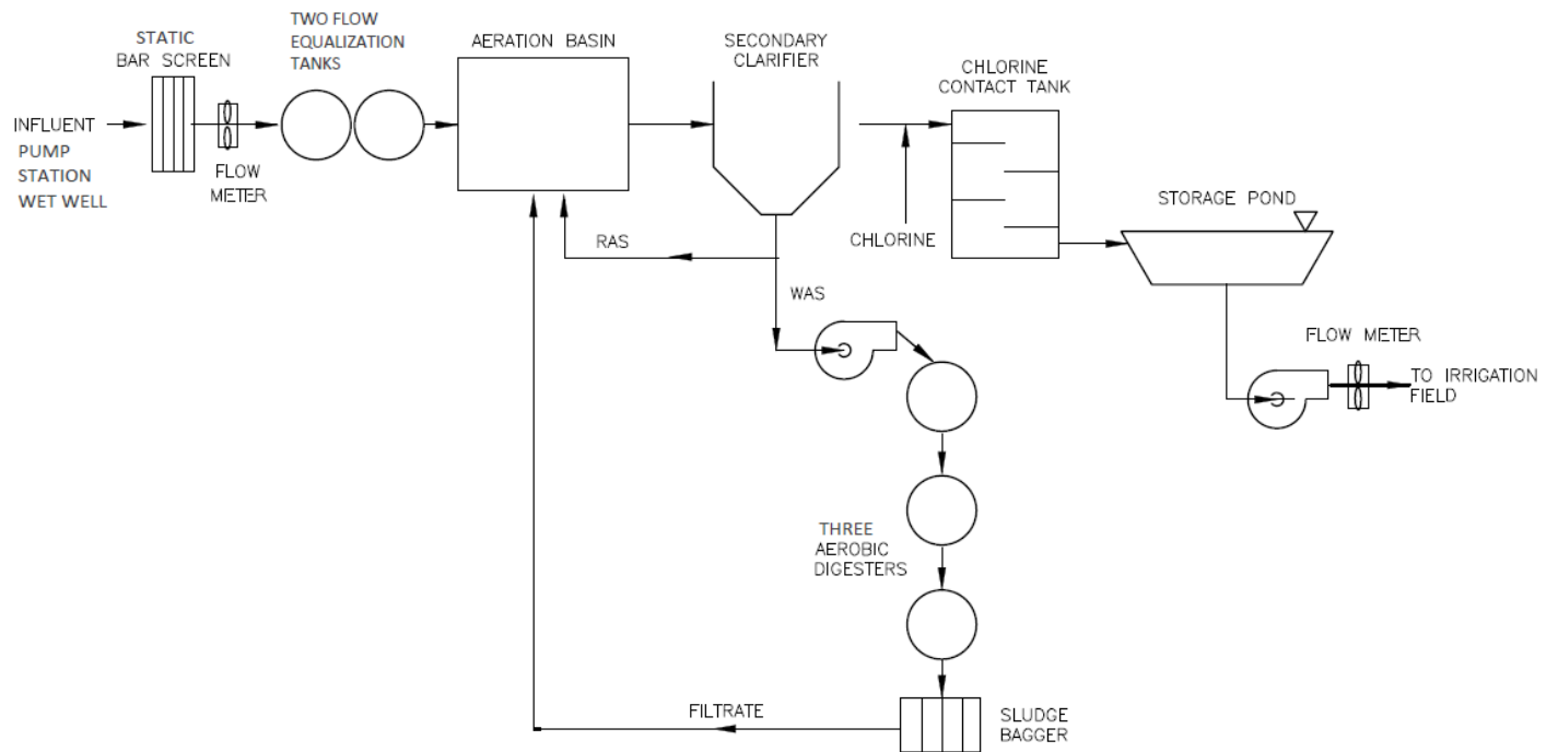
Figure 2. Process Flow Diagram (Source: 2024 Annual Monitoring Report, see Title 22 Engineering Report for more detailed process flow)
