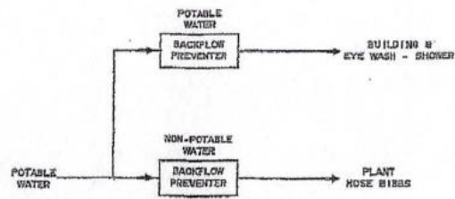
POTABLE AND NON-POTABLE FLOW DIAGRAM
