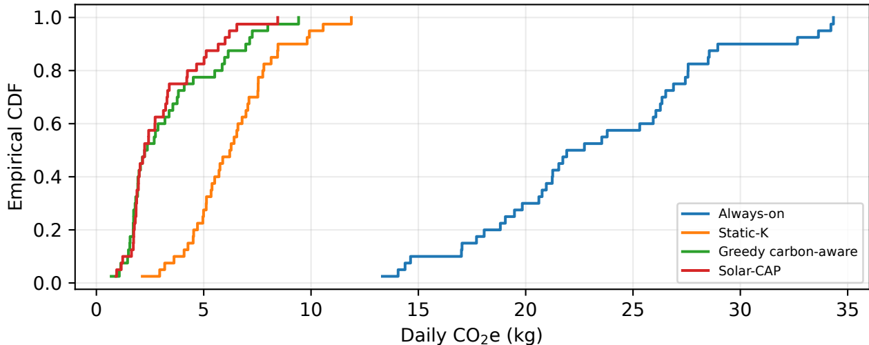
Emission distribution across solar profiles and seeds
