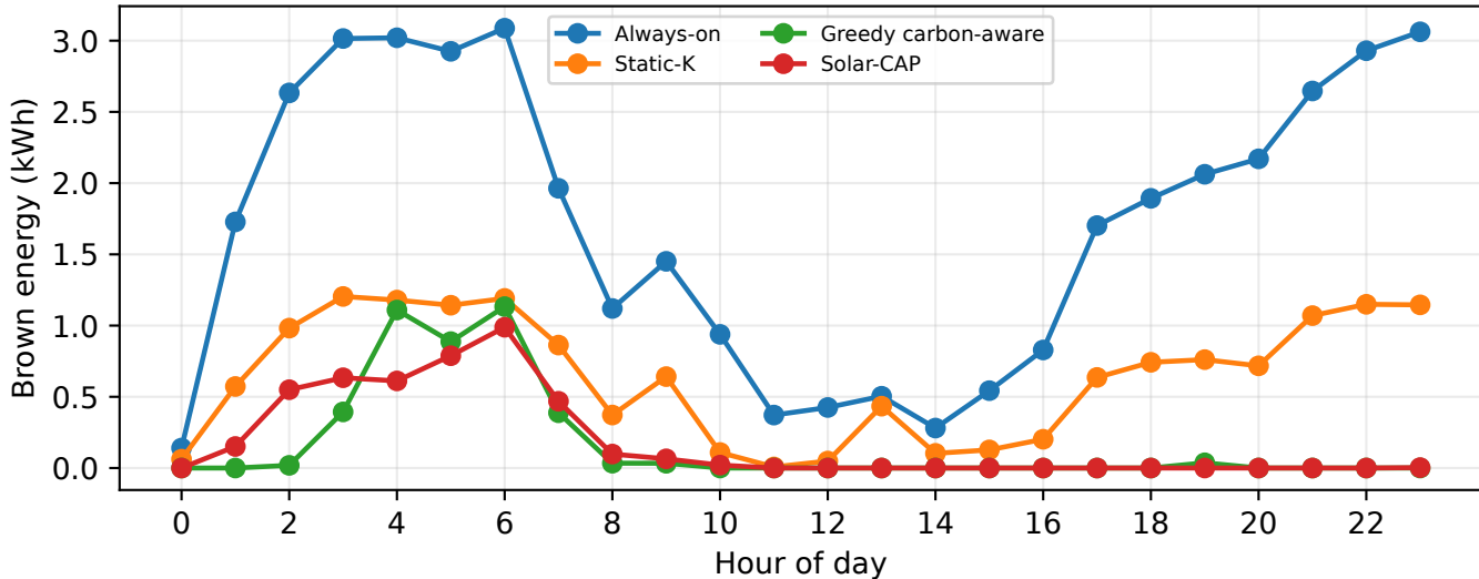
Hourly brown-energy demand under intermittent solar supply
