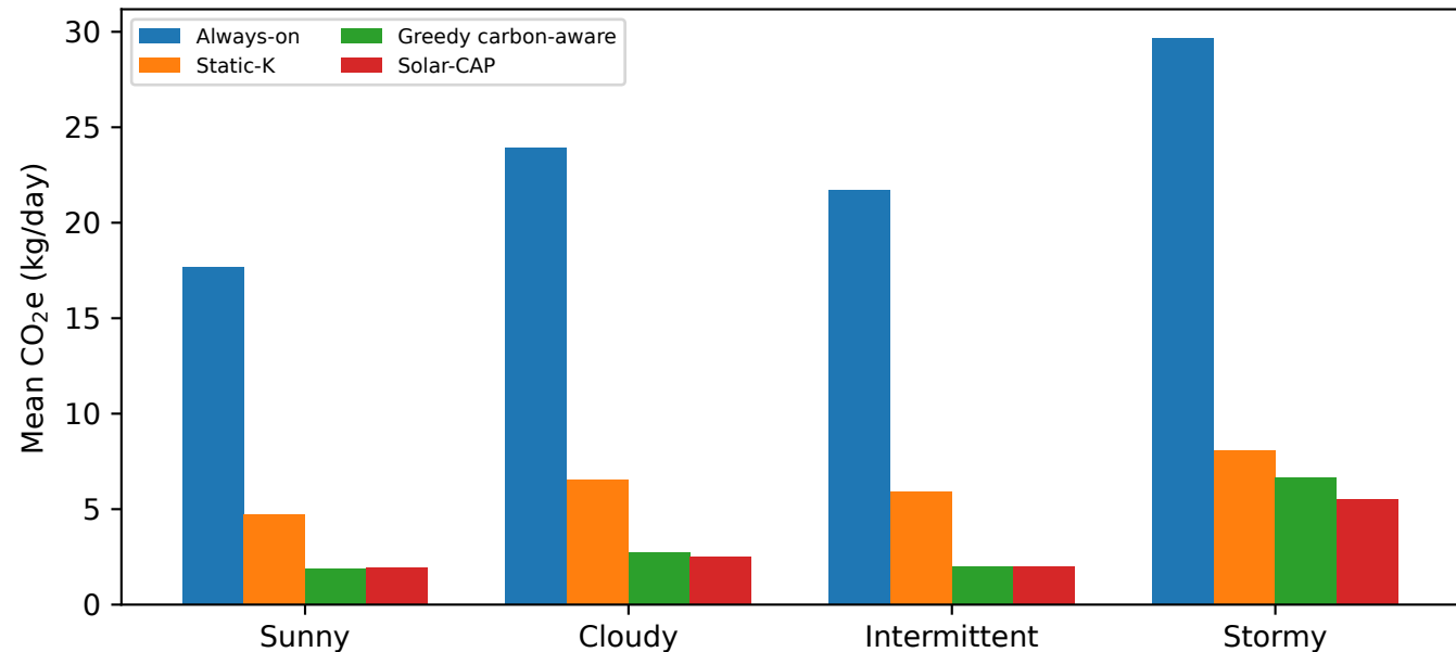
Carbon emissions by solar profile
