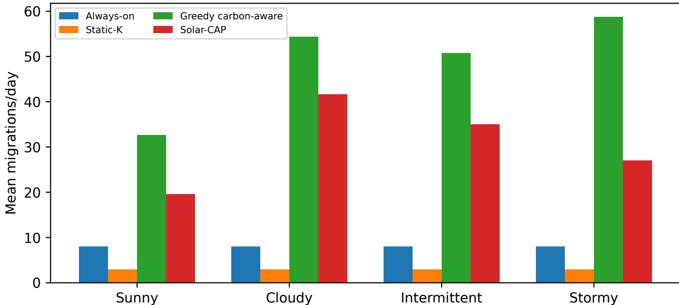
Migration overhead by solar profile
