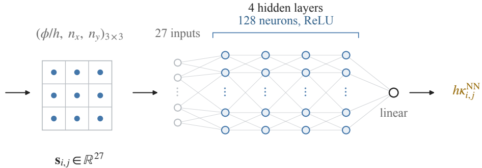
(b) Feature-to-curvature mapping
