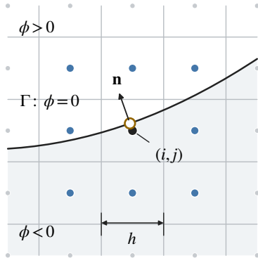
(a) Local level-set geometry
