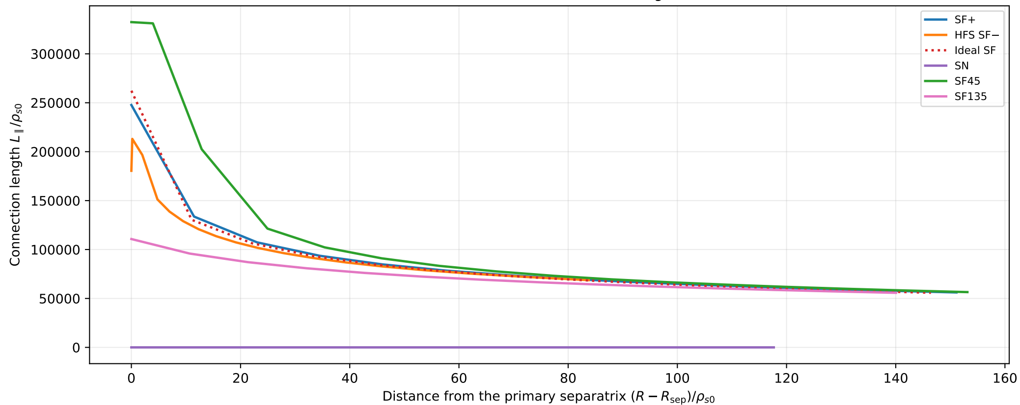
(c) Low-field side connection length
