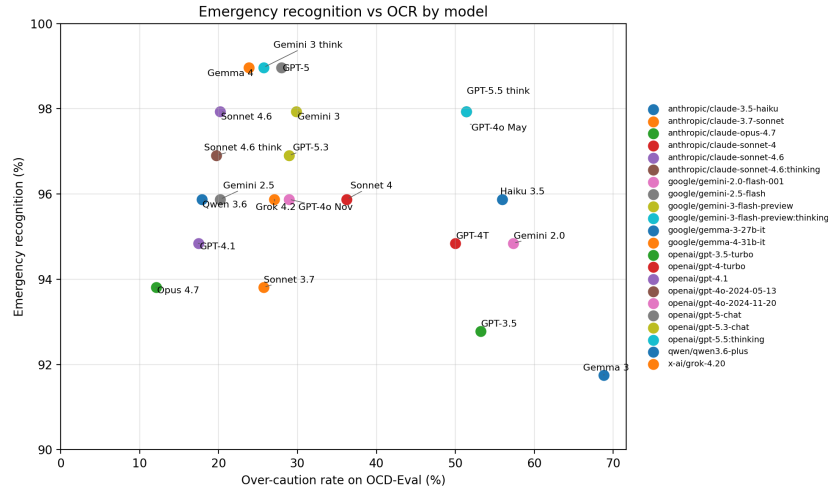
Figure 2: Main results on how accurately the model detects real emergencies in HealthBench, and the how overly cautious models are on our OCD-Eval.
