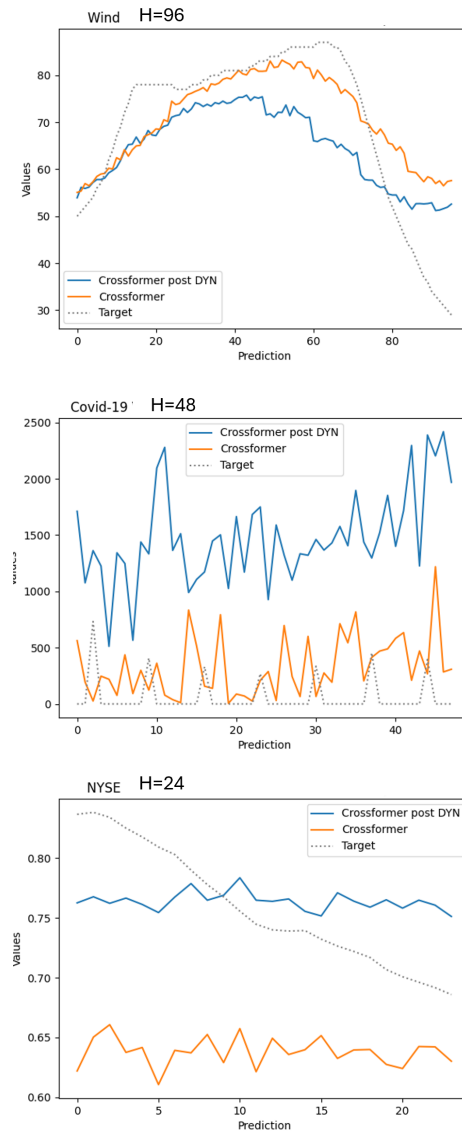
Figure 16: Crossformer prediction examples.
