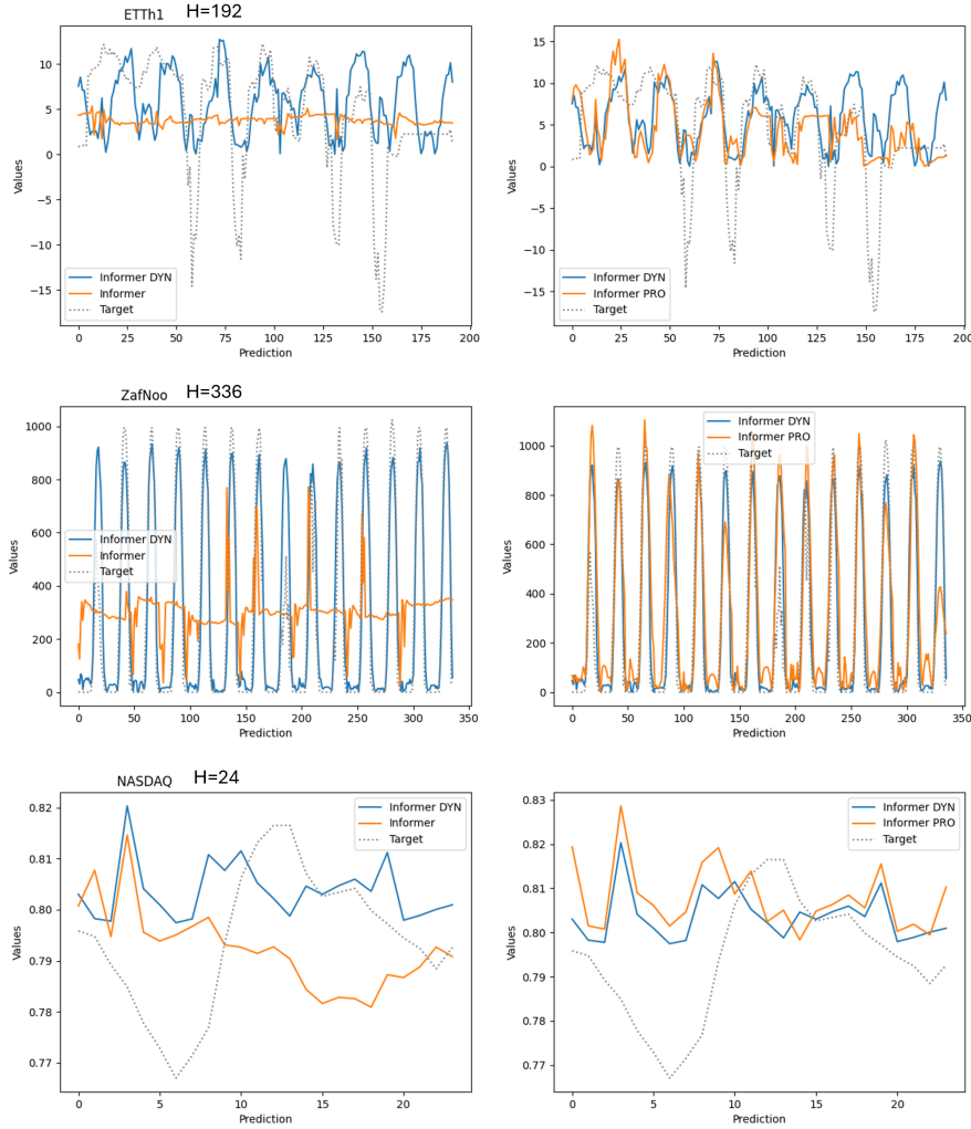
Figure 10: Informer prediction examples.
