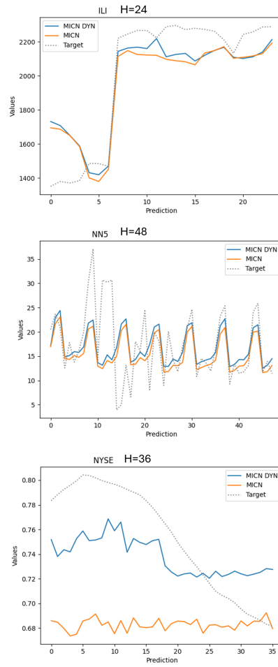
Figure 12: MICN prediction examples.
