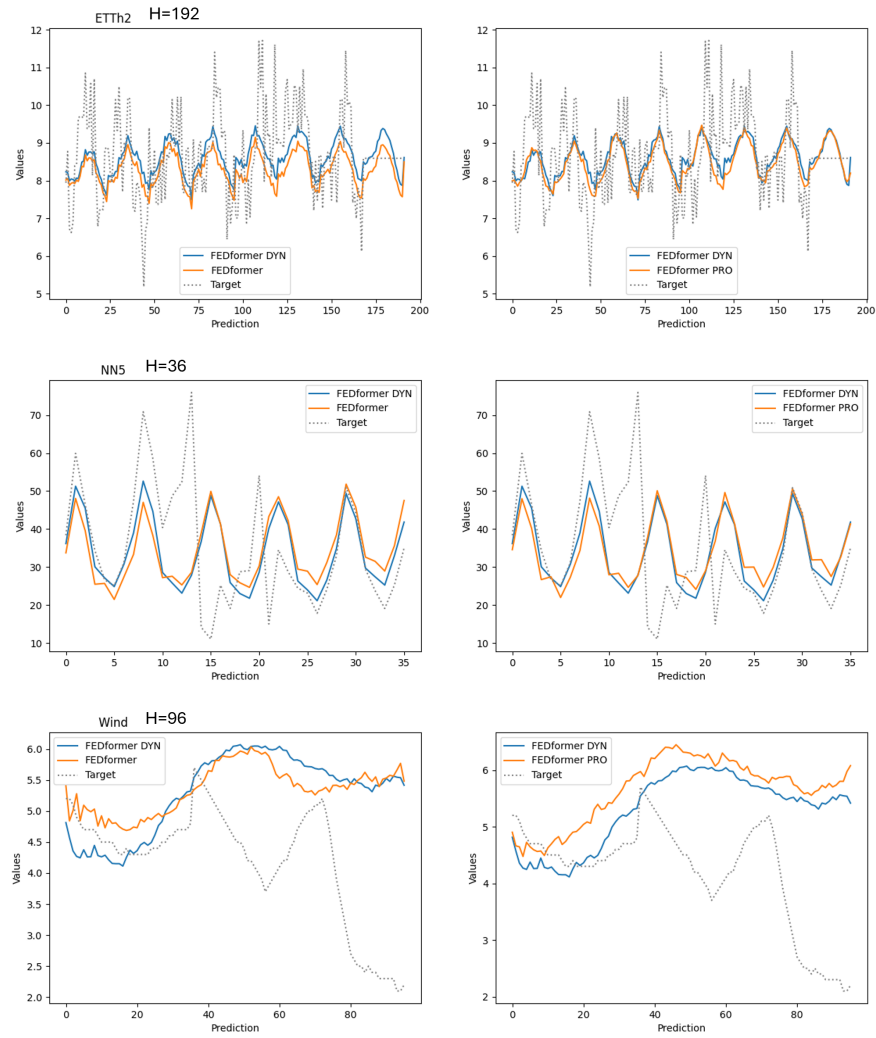
Figure 13: FEDformer prediction examples.
