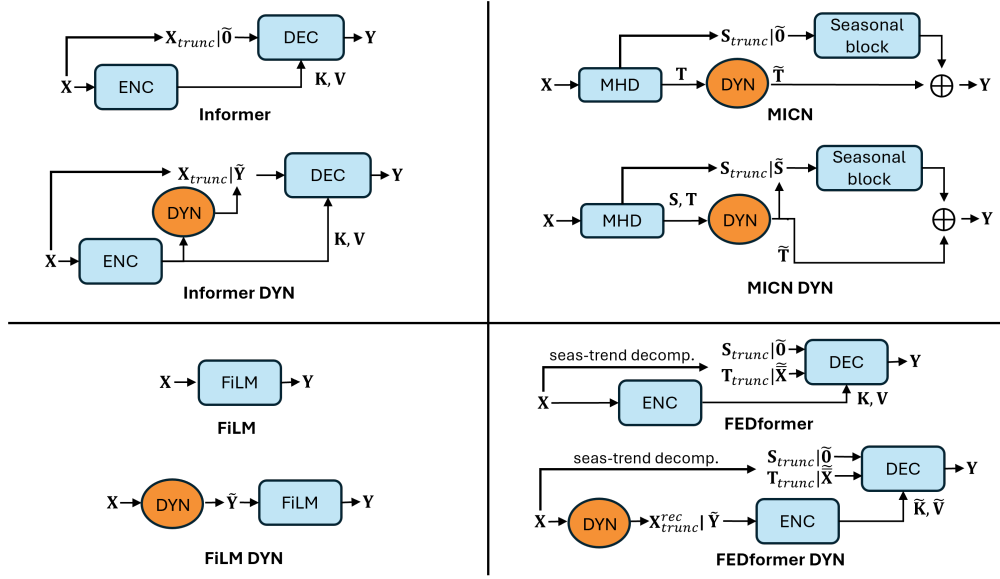
Figure 2: RQ1 models with now full learnable dynamics capabilities. DYN is linear dynamics layer, ENC-DEC is encoder-decoder, MHD is multi-scale hybrid decomposition (defined in MICN, see (Wang et al., 2023)). A|B means A concatenated with B along the time axis, Tilde refers to intermediate variables in the time prediction interval, \tilde{Y} an intermediate prediction from a DYN function, \bar{X} is the mean of X , trunc subscript corresponds to input start tokens.
