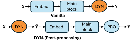
Figure 3: RQ2 models general derivation in their post-processing configuration. For iTransformer, part of the input is concatenated to the DYN output. Embed. stands for embedding layer.
