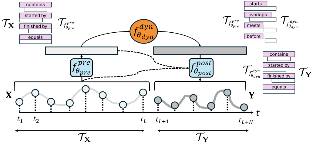
Figure 1: PRO and DYN functions illustrated in the processing chain of a TSF model \mathcal{M}_\theta where “ \mathcal{T}_X before \mathcal{T}_Y ”. PRO functions are framed and blue while DYN function is encircled and orange. Solid lines represent the main data flow. f_{\theta_{post}}^{post} can be fed by \mathbf{X} or/and f_{\theta_{pre}}^{pre}(\mathbf{X}) (dotted lines). Dotted line from \mathbf{X} to f_{\theta_{dyn}}^{dyn} are not drawn for better clarity. Allen relations defined by each function based on its type are illustrated, where the blue interval (resp. white) corresponds to the input - left - (resp. output - right -) interval. The relation name is written in each blue interval.
