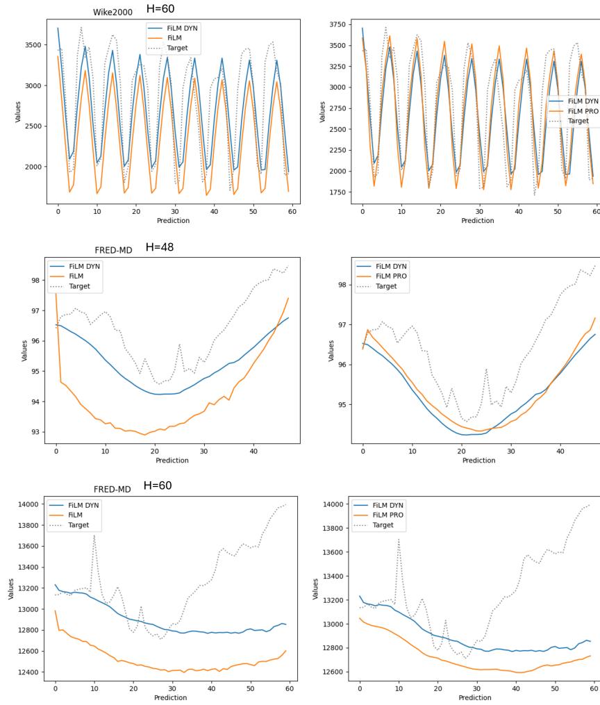
Figure 11: FiLM prediction examples.
