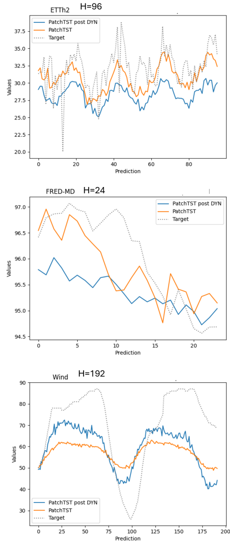
Figure 15: PatchTST prediction examples.
