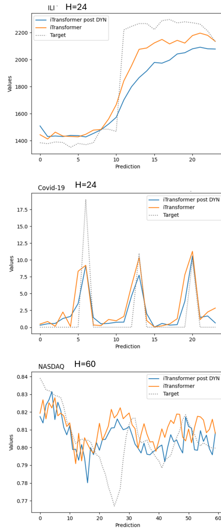
Figure 14: iTTransformer prediction examples.
