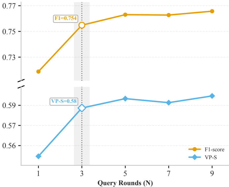
Detection Performance
