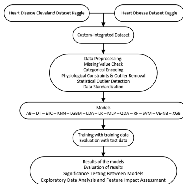
Fig. 1 Block Diagram of the process of using Machine Learning Techniques for heart disease prediction
