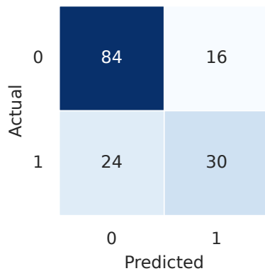
Calibrated SVM
