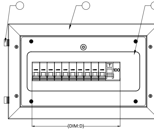
Front view-without Door
